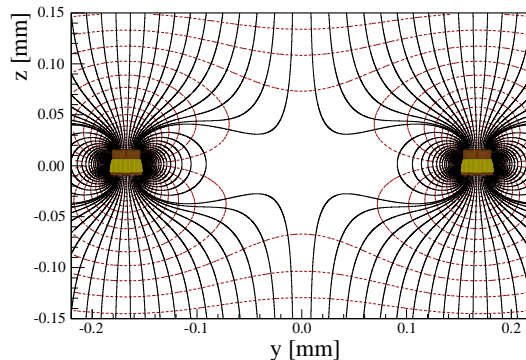
Figure 6. Electric field lines and equipotential lines around a hole in the gating foil placed in an otherwise uniform electric field of 230 V/cm, in the y - z plane at x = 0 . See the left panel of Fig. 1 for the definition of coordinate system. The bias applied to the gating foil ( \Delta V ) is -16.0 V.
