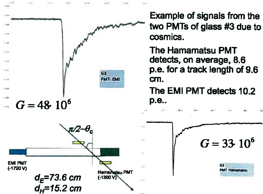
Figure 3: The response of EMI (on the left) and Hamamatsu (on the right) PMTs to cosmic muons as measured by a CRT (time scale: 20 ns/div). Measured PMT Gains (G) are indicated.
