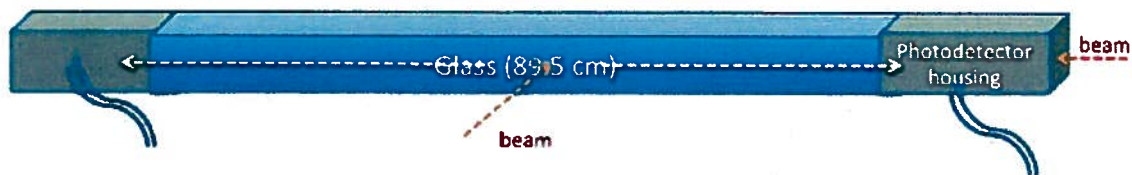
Figure 4.1: SGC1-C glass
