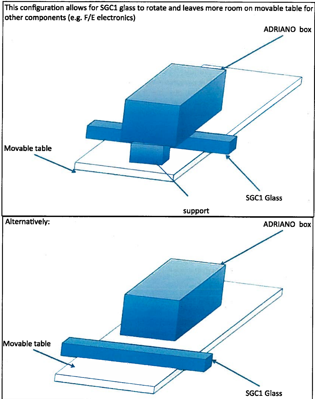
Figure 4.2: SGC1-C glass test beam configuration
