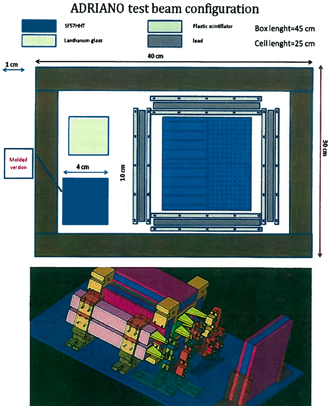
Figure 5: Layout and support structure for testing ADRIANO glass samples
