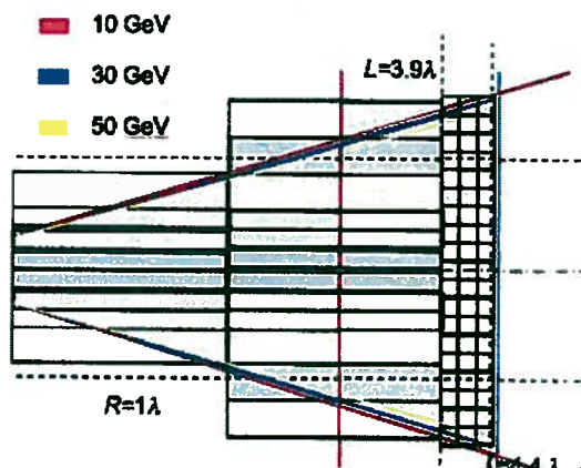
Figure 2: glass calorimeter module configured to contain 95% of the hadron shower, both laterally and longitudinally, up to 30 GeV
