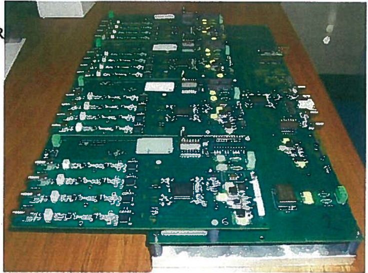
Figure 6: A TB4 Motherboard with a full complement (4) of daughter board for a total of 16 DAQ channels
