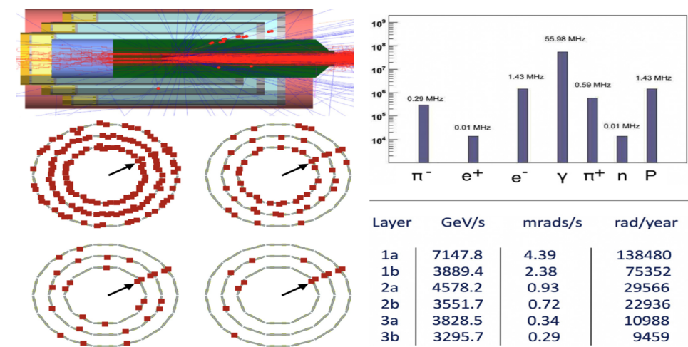
Figure 6: Top Left: one event in the Central Detector at the full CLAS12 10^{35}\text{cm}^{-2}\text{s}^{-1} luminosity Bottom Left: The occupancy in the SVT layers for different thresholds for one event containing a proton track (direction indicated by the arrow). Right: Summary of radiation doses and background rates in the SVT. The rate breakdown for different particles for a threshold of 20 keV at the full luminosity of CLAS12.
