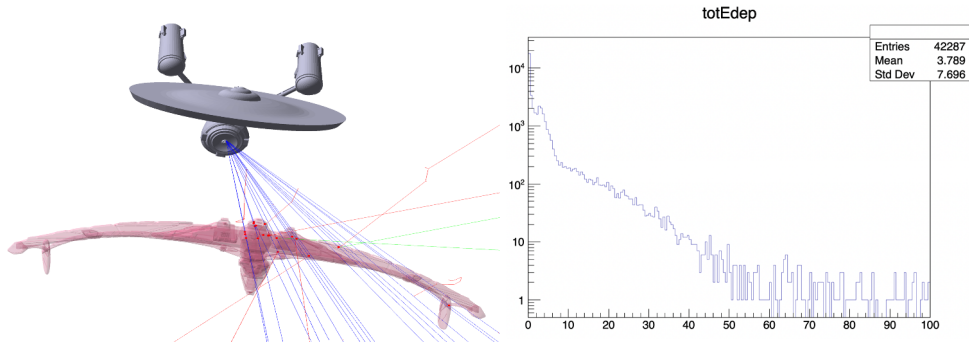
Figure 4: Left: the geometry of the Enterprise and Romulan ships imported from STL files. A proton beam is shot at the Romulan ship and the resulting energy deposited in the Romulan ship is shown to the right.
