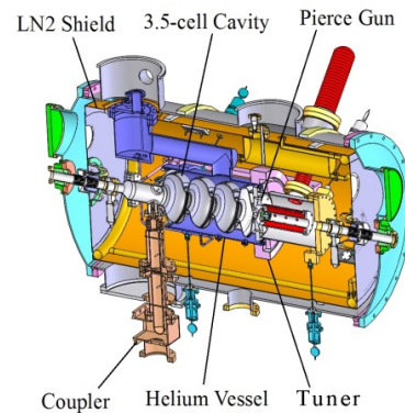
Figure 1: Schematic view of the DC-SRF photoinjector.
