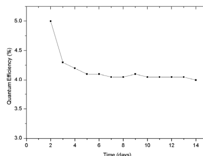
Figure 3: QE of Cs 2 Te cathode.
