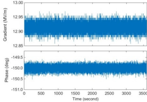
Figure 4: Long-term running of LLRF control system.
