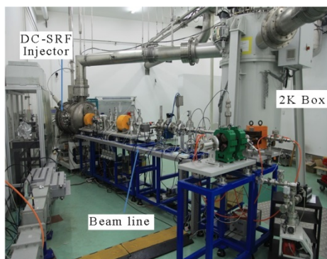
Figure 2: Beam line of the 3.5-cell DC-SRF injector.
