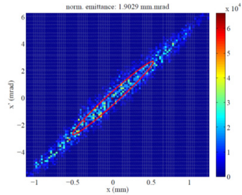
Figure 6: Measured emittance of electron beam.
