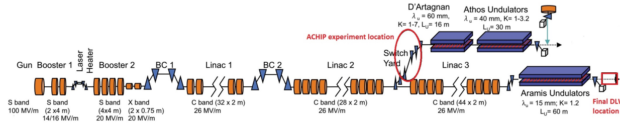
Figure 1: Layout of SwissFEL.
