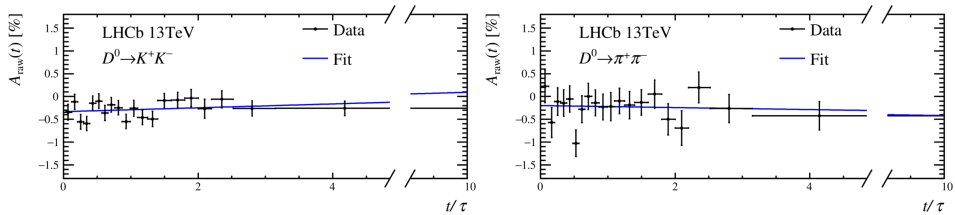
Fig. 2. Measurement of A_\Gamma using Run 2 semileptonic decays of D^0 \rightarrow \pi^+ \pi^- / K^+ K^- [5].
