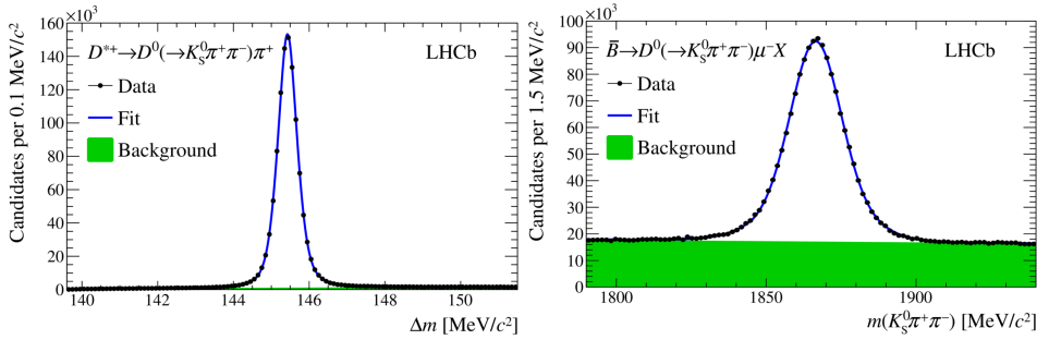
Fig. 1. Invariant mass fits for prompt (left) and semileptonic (right) decays of D^0 \rightarrow K_S^0 \pi^+ \pi^- .
