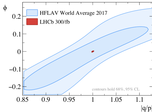
Fig. 3. Potential precision of CP violation parameters measurements.
