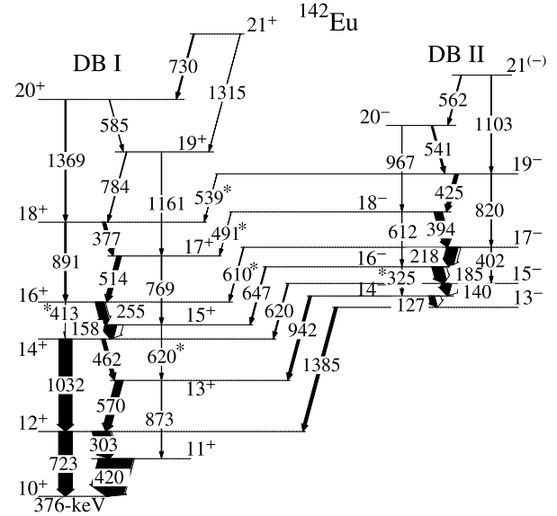
Fig. 1. The partial level scheme of ^{142}\text{Eu} obtained in the present work. The \gamma -ray energies are rounded off to the nearest keV. The newly observed \gamma -ray transitions are marked by an asterisk.
