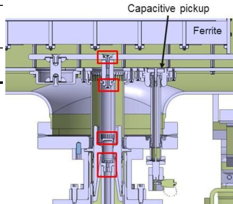
Figure 11: MKI input – red boxes show possible position of high impedance contact.
