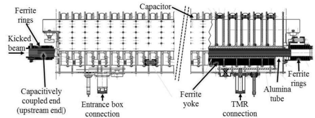
Figure 1: MKI kicker magnet.
