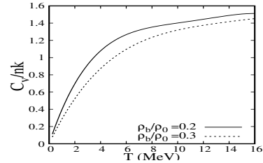
FIG. 3: Specific heat for symmetric nuclear matter for the set IOPB-I
