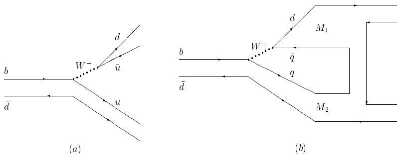
Fig. 1. Dominant diagrams for B decay: (a) tree T and (b) penguin P .
