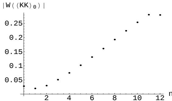
Fig. 3. Dependence of FSI-induced effects on the number of intermediate channels included for B \rightarrow (K\bar{K})_{I=0} decays.
