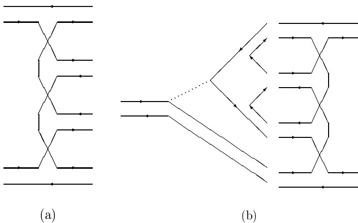
Fig. 2. (a) Multiparticle production at high energy. (b) Suppression mechanism for B \rightarrow |f_4\rangle \rightarrow PP .
