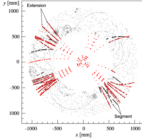
Figure 4.3: Hits used in tracks associate with a simulated t\bar{t} event with no pileup [116]. Red points indicate hits that were used in the first round of tracking, and the black TRT hits show those that were associated in the back tracking step.
