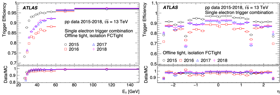
Figure 3.23: Efficiency for single electron trigger as a function of the offline (fully processed) E_T (left) and \eta (right) [112]. The electrons considered for this plot must be “tight” and satisfy the “FCTight” isolation requirement, which indicate high confidence that they are well-isolated, real electrons (see Section 4.2).
