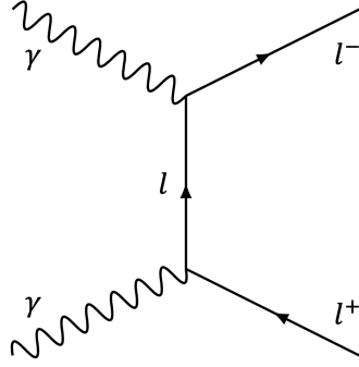
Figure 2.16: Feynman diagram depicting the process \gamma\gamma \rightarrow l^+l^- .
