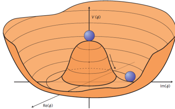
Figure G.1: Form of the Higgs potential when \lambda > 0 [277]. The vacuum expectation value of the scalar field is then non-zero.
