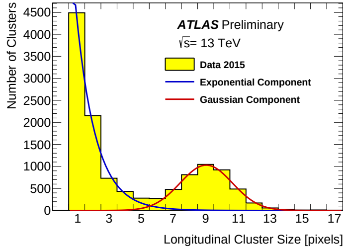
Figure D.1: Typical distribution of the pixel-cluster size in the direction parallel to the beam axis, in the second-most forward IBL module. The 12413 clusters that populate this plot originate from 10433 randomly-triggered events during ATLAS physics data-taking in 2015. The distribution is fit to the sum of a Gaussian signal, plus an exponentially-falling background of shorter clusters. The mean of the Gaussian from the fit is a cluster length of 9-pixels, and its area is proportional to the number of charged particles originating from the luminous region. The exponential area contains contributions from secondary interactions and afterglow that will deviate from linear proportionality to luminosity.
