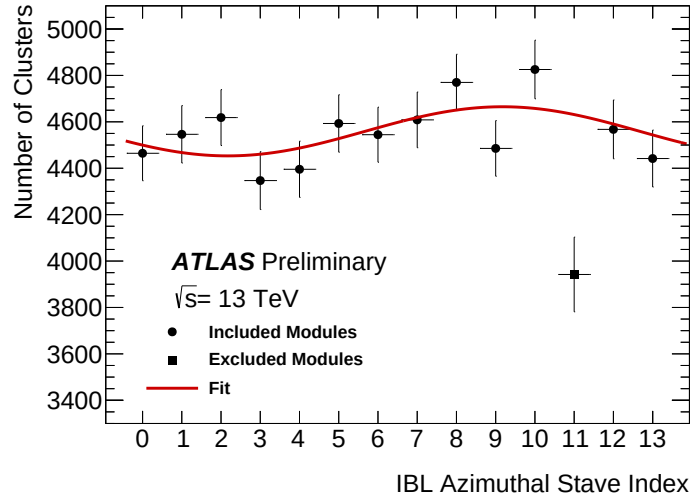
Figure D.3: Azimuthal dependence of the long-cluster (Gaussian) signal for the forward-most modules of the IBL. The sinusoidal dependence arises because in the plane perpendicular to the average beam direction, the luminous region is not perfectly centered on the IBL’s central axis. In order to avoid being affected by occasional underperforming or noisy modules, the measured azimuthal dependence of the long-cluster signal is fit to a sinusoidal function. Outliers are excluded from the fit on the basis of internal consistency. In this example, the number 12 module was inefficient during the run considered and was excluded from the fit because its residual exceeded 4 sigma.
