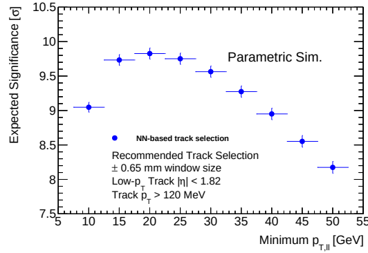
Figure 17.14: The expected significance as a function of the minimum p_{T,\ell\ell} cut for a new signal region. In the first round of the analysis, this was placed at 30 GeV.
