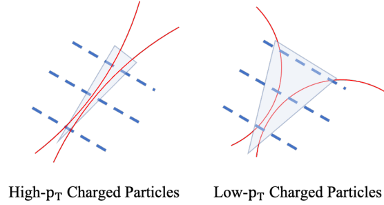
Figure 15.2: Lower- p_T charged particles curve more in ATLAS’s magnetic field than high- p_T particles. Because of this, hits on different layers associated with a single particle can be further apart. To make a complete set of seeds, a much larger number of hit combinations must be considered.
