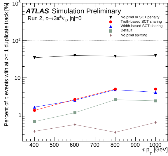
Figure B.5: Curves representing the proportion of events with at least one duplicate track as a function of \tau p_T . An event has a duplicate track if more than one reconstructed track is matched to any pion at generator level. The different marker styles represent different settings in the ambiguity solving stage. “Default” uses the pixel neural network.
