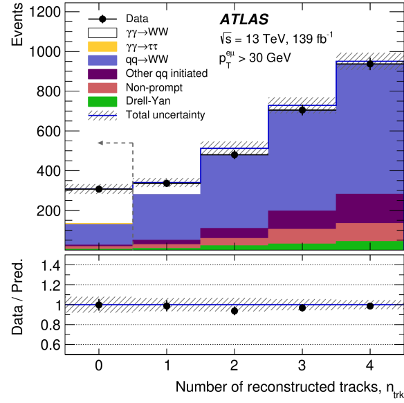
Figure 13.8: Data and post-fit yields in the signal region and CR2 [187]. All events in this plot have p_{\text{T},\ell\ell} > 30 \text{ GeV} , so the signal region is events with n_{\text{trk}} = 0 , and CR1 are those events with 1 \leq n_{\text{trk}} \leq 4 . The signal region has about a 1.3:1 signal to background ratio.
