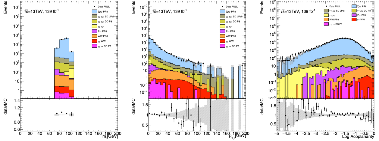
Figure 18.1: The data and simulation agreement for di-lepton m_{\ell\ell} (left), p_{T,\ell\ell} (middle), and acoplanarity (right) for \mu\mu events in the Z -peak region. The natural log of the acoplanarity is plotted, such that the most back-to-back leptons are on the left-hand side of the plot. The data comes from the event picked data selected with the requirements of Table 18.1, and the simulation is that laid out in Table 18.2. The data in this region has a scale factor of 50 applied.
