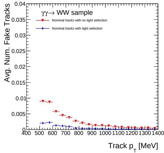
Figure 17.2: The average contribution of fake nominal tracks with and without tight selection that fall into a \pm 1 mm window around the lepton vertex, as a function of track p_T . When there is a fake track in such a window, it is more likely to have lower- p_T . This plot was made using tracks from the HERWIG 7 elastic \gamma\gamma \rightarrow W^+W^- sample, which are either pileup or fake tracks. The tracks are required to have |d_0| < 1.0 mm. On average 99% of nominal tracks are considered true.
