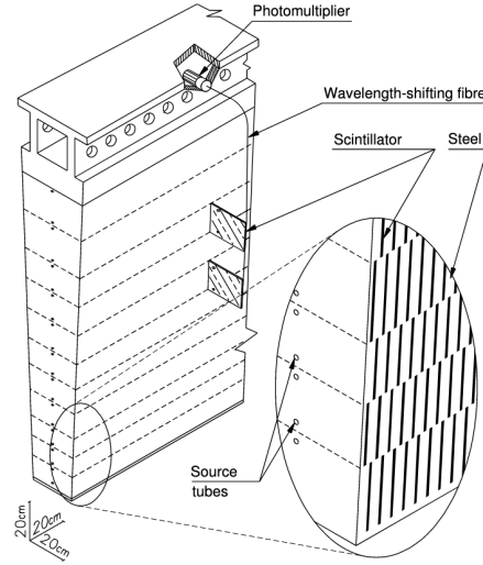
Figure 3.12: Layout of the Tile Calorimeter [76]. Steel and scintillating tiles are interleaved to created and measure hadronic showers.
