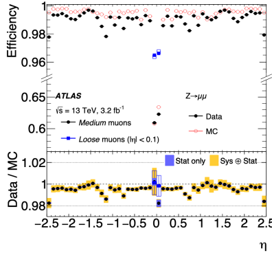
Figure 4.9: Reconstruction efficiency for medium tagged muons with p_T > 10 GeV as a function of \eta [130]. The efficiency is determined using the tag-and-probe method in Z \rightarrow \mu\mu events.
