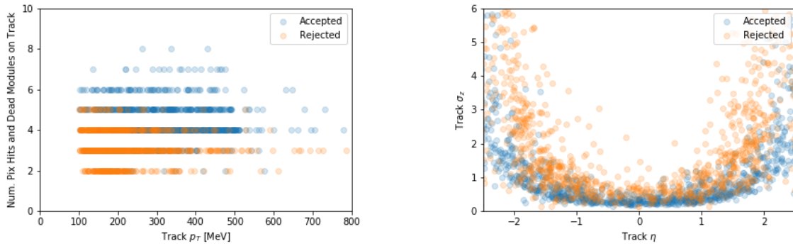
Figure 17.12: (Left) Scatter plot of p_T and number of pixel hits plus dead modules for 1000 accepted and 1000 rejected low- p_T tracks after applying the suggested neural network cut. (Right) Scatter plot of \eta and uncertainty on the z parameter in the track fit for 1000 accepted and 1000 rejected low- p_T tracks. The tracks in these plots must have |d_0| < 1.0 mm and p_T > 100 MeV. Both of these plots were made using tracks from the HERWIG 7 elastic \gamma\gamma \rightarrow W^+W^- sample, which are either pileup or fake tracks.
