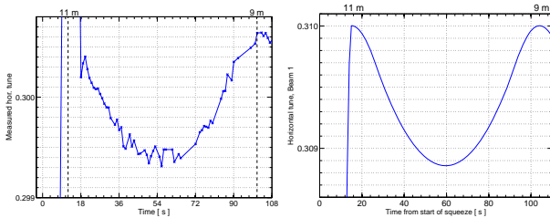
Figure 10: Measured (left) and simulated (right) tune excursion during the \beta^* step from 11 m to 9 m. Simulations are performed by running MADX on the LSA settings extracted every second (simulations by X. Buffat, EPFL).
