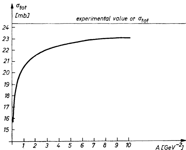
Fig. 2. Total cross-section calculated from the model
