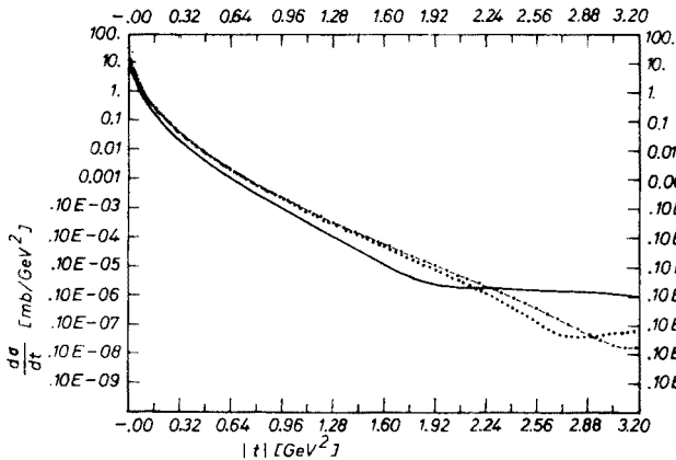
Fig. 3. Differential elastic cross-section: — A = 0.01 \text{ GeV}^{-2} ; ..... A = 1 \text{ GeV}^{-2} ; - - - A = 10 \text{ GeV}^{-2}
