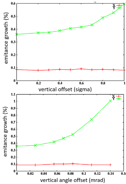
Figure 4: The proton beam emittance growth after electron beam replacement as a function of the electron beam vertical offset amplitude (top) and angle (bottom).
