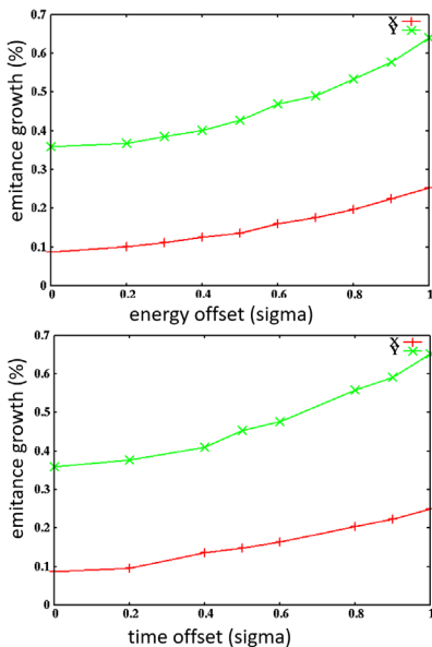
Figure 5: Proton beam horizontal and vertical emittance growth as a function of longitudinal energy (top) and time (bottom) offsets of the electron injection replacement.
