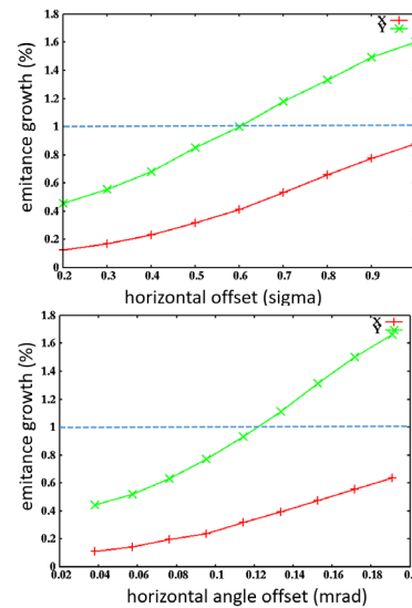
Figure 3: proton beam horizontal and vertical emittance growth as a function of horizontal position (top) and angle (bottom) errors of the electron injection replacement.
