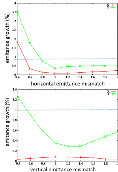
Figure 6: Proton beam horizontal and vertical emittance growth as a function of horizontal (top) and vertical (bottom) emittance mismatch factors of the electron injection replacement.
