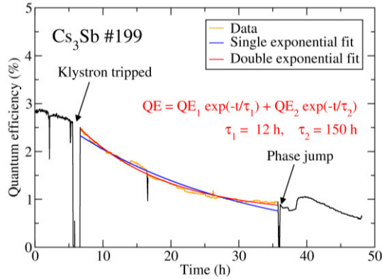
Figure 3: Lifetime measurement of fresh \text{Cs}_3\text{Sb} cathode #199 with 2.3 nC/bunch and 350 ns train length.
