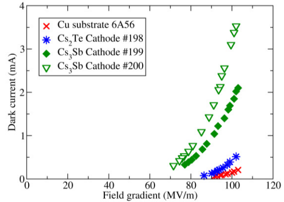
Figure 5: Dark current measured with \text{Cs}_3\text{Sb} , \text{Cs}_2\text{Te} and Cu cathodes.
