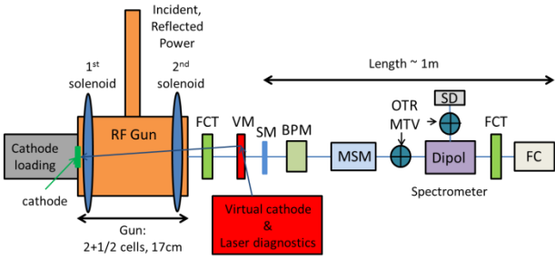
Figure 1: Layout of PHIN. Fast current transformers (FCT), vacuum mirror (VM), steering magnet (SM), beam position monitor (BPM), multi-slit mask (MSM), optical transition radiation screens (OTR), gated cameras (MTV), segmented beam dump (SD), Faraday cup (FC).
