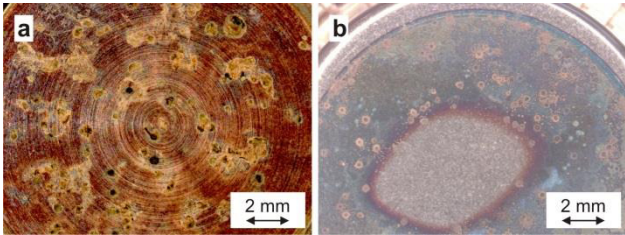
Figure 2: Optical microscope images of Cs 3 Sb cathode #193 (a) and Cs 2 Te #198 (b) after usage. A concentric ring structure of the substrate of cathode #193 is clearly visible. The spot in the center of cathode #198 is due to ion sputtering during XPS studies [6].
