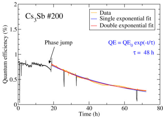
Figure 4: Lifetime measurement of used \text{Cs}_3\text{Sb} cathode #200 with 1 nC/bunch and 800 ns train length.
