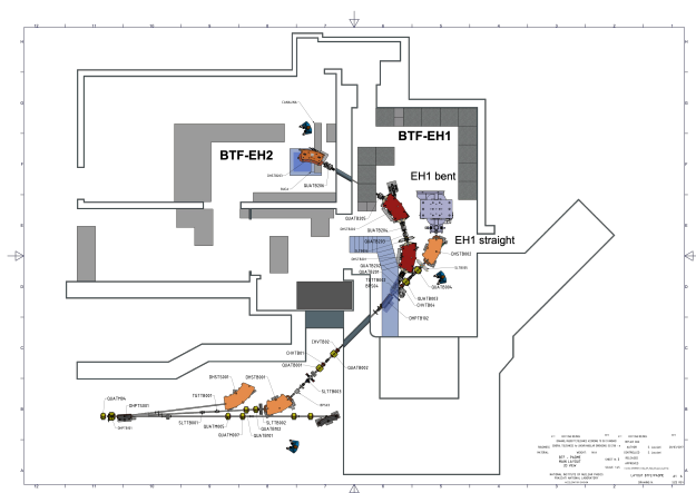
Figure 2: Layout of the BTF line and area.
