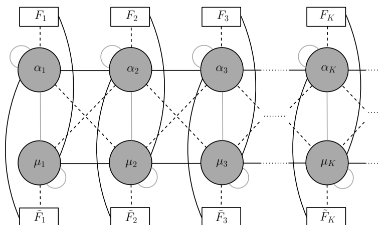
Figure 2. A generic quiver field theory in which the IR is dual to the holographic background defined by the functions in (6) and (7).
