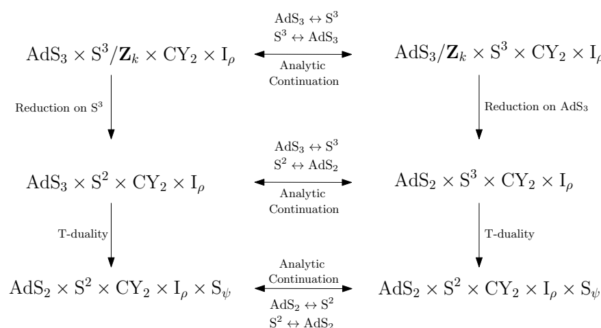
Figure 7. Connections between the different classes of solutions reviewed in this paper.
