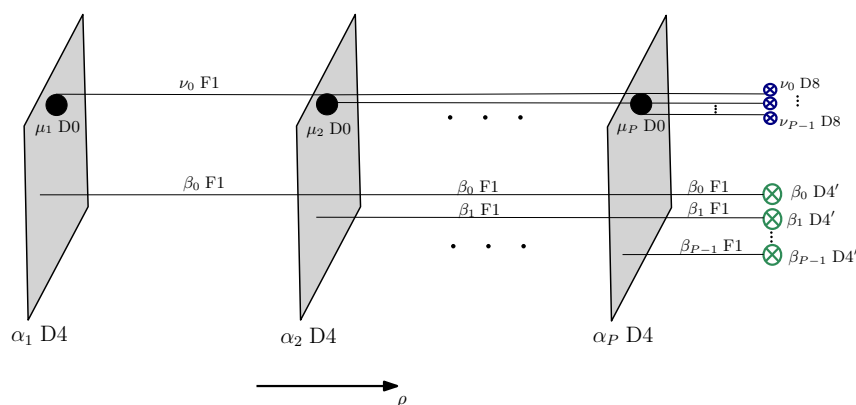
Figure 5. Hanany–Witten brane set-up equivalent to the brane configuration in Table 4.
