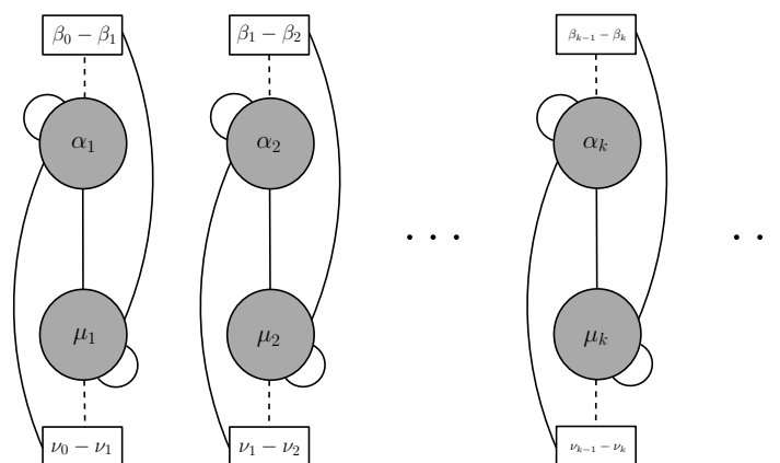
Figure 6. One-dimensional quiver field theory in which the IR limit is dual to the AdS_2 backgrounds reviewed in Section 4.
