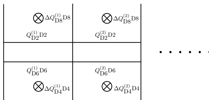
Figure 1. Generic Hanany–Witten brane set-up associated with the holographic background defined by the functions in (6) and (7). The vertical lines are NS5-branes, the horizontal lines represent D2- and D6-branes, and the crosses indicate D4- and D8-branes.
