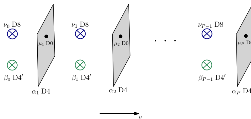
Figure 4. Hanany–Witten brane set-up associated with the brane charges of the solutions.
