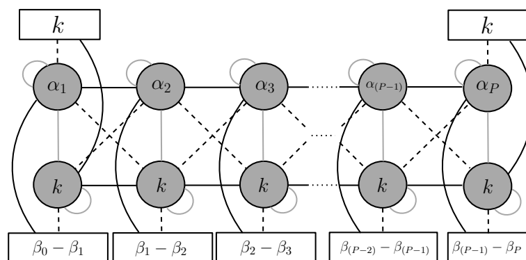
Figure 3. Generic quiver field theory in which the IR is dual to the AdS_3 \times S^3/Z_k \times CY_2 \times I M-theory solutions defined by the functions in (6) and (7).
