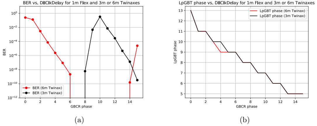
Figure 3.33: BER and phase difference tests on the uplink with the entire transmission chain consisting of 1 m flex and 3 m twinAx and 6 m twinax with GBCR2 in retiming mode respectively. The DLL phase difference between lpGBT V0 and GBCR2 depends on the length of the data transmission chain and consequently the configuration for the lowest BER. It shows that depending on the length of the chain, the parameters must be set
