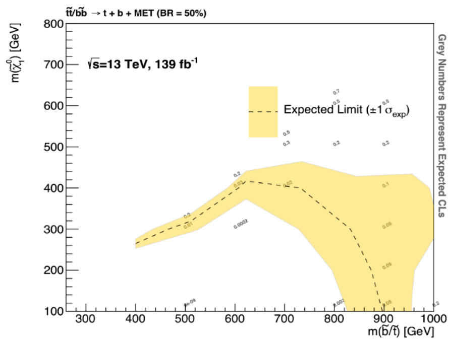
Figure 4.25: Expected model-dependent exclusion limits for SRB at 139\text{ fb}^{-1} , with no systematic uncertainties included. The limit is shown in the \tilde{b} mass (x-axis) and \tilde{\chi}_1^0 mass (y-axis) plane. The limit plot uses background normalisation factors obtained from background-only fits in t\bar{t} and t\bar{t}Z CRs for SRB.
