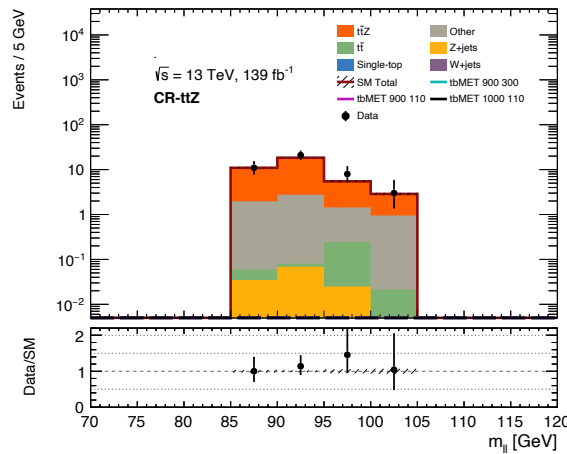
Figure 4.16: Distribution of invariant mass of the two leptons from Z -boson in the three lepton CR-ttZ. The coloured, solid histograms show the SM backgrounds scaled to 139 \text{ fb}^{-1} . The hashed area represents the statistical error on the prediction. The black points show the data with statistical error bars. The lower panel contains the ratio of data over SM prediction.
