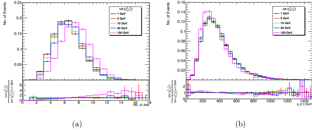
Figure 4.4: No. of jets vs. number of events (a) and leading jet p_T (b) for m_{\tilde{t}} 900 \text{ GeV} and m_{\tilde{\chi}_1^0} 400 \text{ GeV} .
