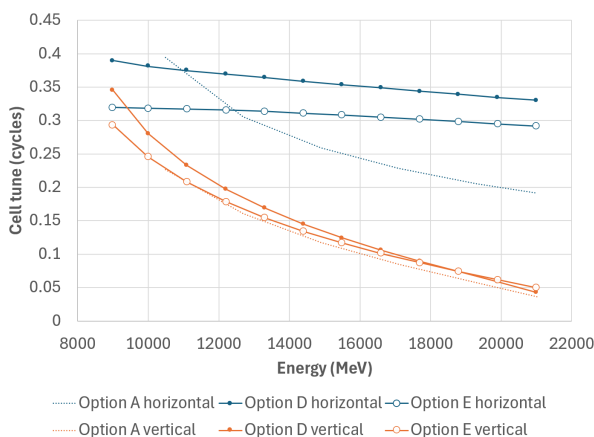
Figure 3: Cell tunes of the extended energy range sextupole lattices (D and E) compared to the baseline option A.
