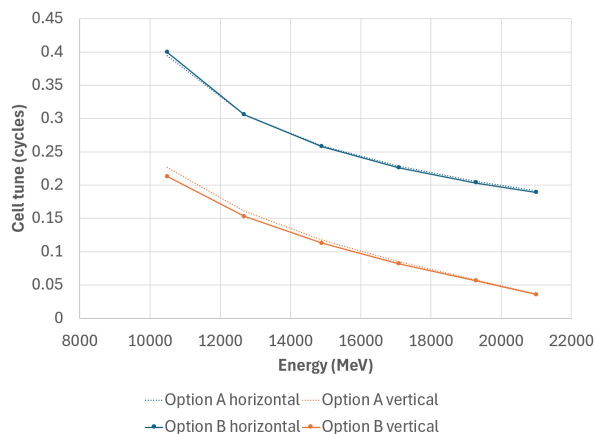
Figure 1: Cell tunes of the optimised linear field option B compared to the baseline option A.
