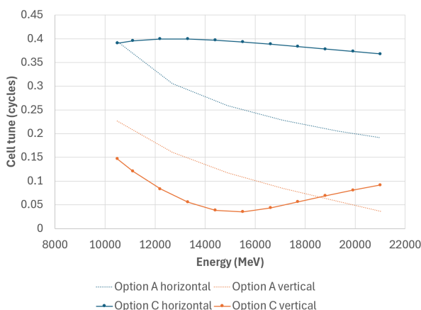
Figure 2: Cell tunes of the optimised lattice with sextupole (option C) compared to the baseline option A.
