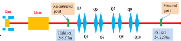
Figure 2: layout of the PITZ beam line for simulation studies of the multi-quads scan method for 4D emittance measurements.
