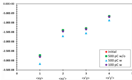
Figure 4: Reconstructed 4D emittance correlation terms from simulation studies with multi-quads scan method and compared with the initial ones.
