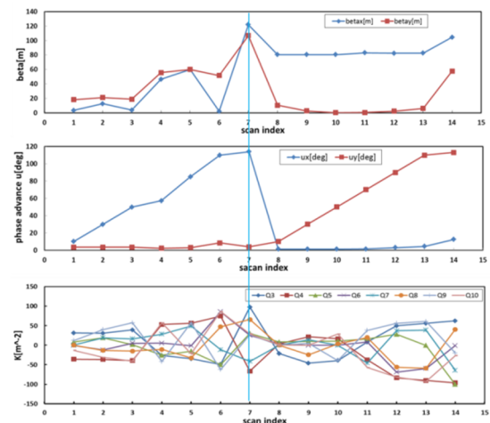
Figure 3: Beam matching for multi-quads scan method for simulation studies: beam size ( \beta_x, \beta_y ) at measured point, phase advance ( \mu_x, \mu_y ) between reconstructed point and measured point, and eight quads (Q3-Q10) settings for each scan.
