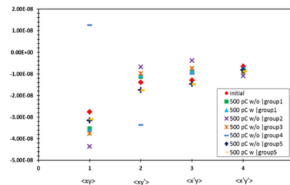
Figure 7: Reconstructed 4D beam matrix correlation terms from simulation studies with rotated slits plus two quads method and compared with the initial ones.
