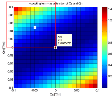
Figure 1: Simulation results for the coupling factor (colour code) as a function of Qs and Qn.
