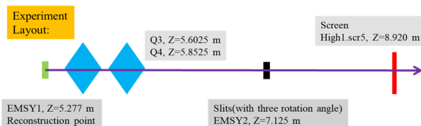
Figure 5: Layout of PITZ beam line used for the simulation study of the 4D emittance measurement with rotated slits plus two quads.
