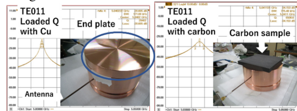
Figure 6: Cavity for measurement of electronic conductivity of the sample.
