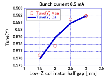
Figure 10: Measured tune shift compared with the estimated values from calculated impedance.
