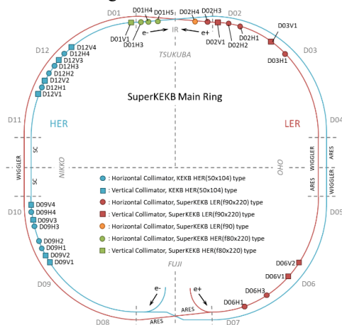
Figure 1: Location of collimators in the main ring of SuperKEKB. The terms H and V in the collimator represent the horizontal and vertical collimators [2].
