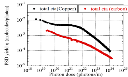
Figure 2: Comparison between PSD of copper and carbon.
