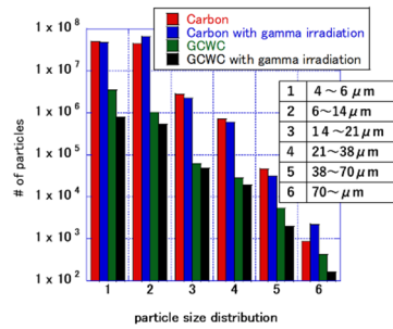
Figure 5: Measurement results of the size and number of the dust particles generated.
