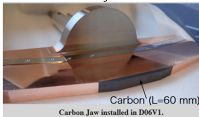
Figure 4: The jaw attached carbon.
