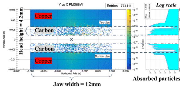
Figure 3: Absorbed particle distribution at the D06V1 jaw attached carbon (L = 60 mm).
