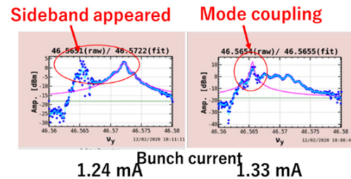
Figure 11: Observation of TMCI phenomenon.
