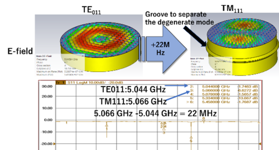
Figure 7: Excited mode in the cavity.
