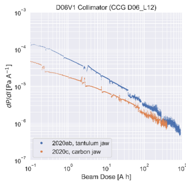
Figure 9: dP/dI beside the low-Z collimator as a function of the beam dose.
