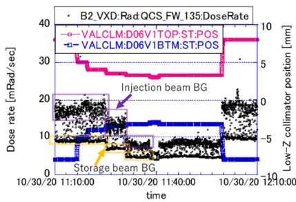
Figure 8: Measured value of BG when the gap of low-Z collimator changed.
