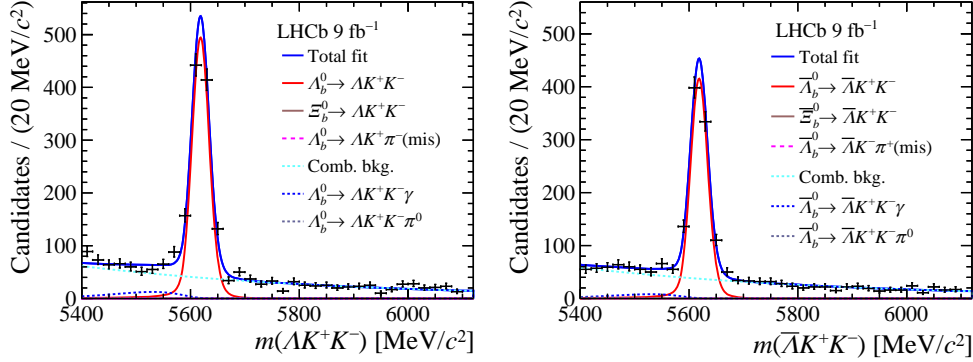
Fig. 2. – Fit to the invariant-mass spectrum for the \Lambda K^+ K^- final state and its CP conjugate [10].
