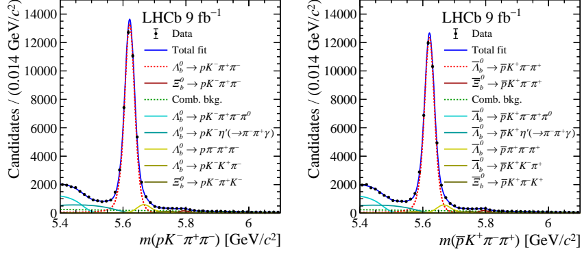
Fig. 3. – Fit to the invariant-mass spectrum for the pK^-\pi^+\pi^- final state and its CP conjugate [11].
