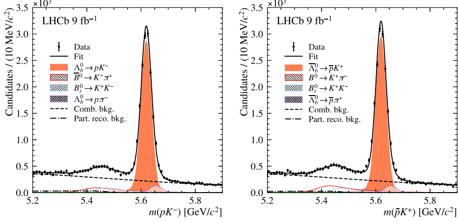
Fig. 1. – Fit to the pK^- invariant-mass spectrum (full dataset) for the A_{CP}(\Lambda_b^0 \rightarrow pK^-) selection [8].
