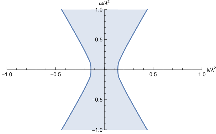
Figure 3.10. The region of convergence. In the shaded area the L \rightarrow \infty ( N_f \rightarrow 0 ) limit is not convergent while outside this area \lim_{L \rightarrow \infty} G_L = G_{\text{quenched}} .
