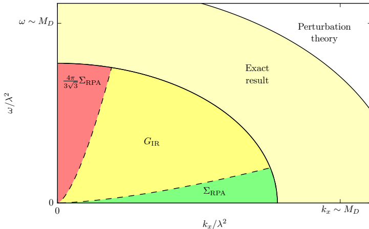
Figure 3.8. A sketch of the regimes of applicability of various approximations to the exact fermion Green's function of the elementary quantum critical metal in the double scaling limit. The G_{\text{IR}} approximation is applicable both in the deep yellow region and the red and green regions.
