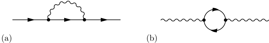
Figure 2.1. One loop corrections to fermion (a) and boson (b) self-energies due to Yukawa interaction. For a gapless boson (b) is the one loop contribution to Landau damping: this contribution to the self-energy can dominate in the IR. This term (b) is clearly proportional to the number of fermions N_f in contrast to the one-loop correction to the fermion self-energy (a). In the limit N_f \gg N_b the boson self-energy/Landau damping therefore dominates, whereas it is suppressed in the opposite limit N_f \ll N_b .
