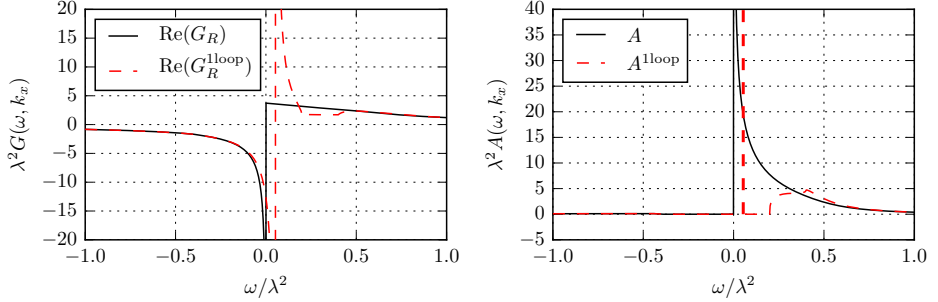
Figure 2.8. The real and the imaginary part Green's function at the outer Fermi surface ( k_x = k_x^* \approx 0.4\lambda^2 , v = 0.5 ) as a function of \omega (solid line), and the one-loop truncated result (dashed). The spectral weight of the one-loop approximation is concentrated to a \delta -function whereas the spectral weight of the full result is spread in the power-law singularity.
