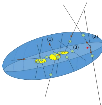
Figure 1: It illustrates how the different entanglement cases, discussed in the text, appear as dark matter with attraction towards the galaxy center and mass in the center or in halos. Green circles represent center of masses. (Reused from [5]).
