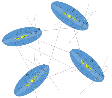
Figure 2: The violet lines between galaxies in a cluster sketch some entanglement support domain that would exist between the galaxies of the cluster. Per the dark matter mechanisms discussed in [1,5], these contribute additional gravity like attraction effects. Combinatorial considerations suggest that the additive contributions could rapidly amount to apparently 10 times or more dark matter that conventionally predicted.
