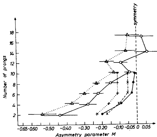
Fig. 6. Median value M of the CMS angular distribution vs number of prongs for: \bullet — 16 GeV \pi^-p , exact transformation; \times — 16 GeV \pi^-p , folding procedure transformation; + \cdots 16 GeV \pi^-p , ultrarelativistic transformation; \circ — 60 GeV \pi^-p , folding procedure transformation; \Delta \cdots 60 GeV \pi^-p , ultrarelativistic transformation. Horizontal bars represent statistical errors
