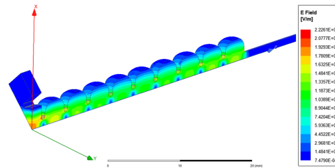
Figure 2: 3D model of one-eighth of half a SW structure simulated with the HFSS software. The surface electric field is shown for a 125 MV/m on-axis accelerating gradient.
