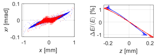
Figure 8: Transverse and longitudinal phase space at the photo-injector exit spaces with (red line) and without (blue line) the Ka-band linearizer.
