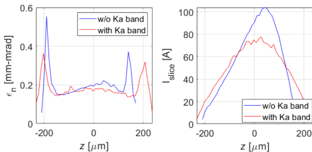
Figure 7: Electron beam slice analysis in terms of emittance (left) and peak current (right) at the photo-injector exit spaces with (red line) and without (blue line) the Ka-band linearizer.
