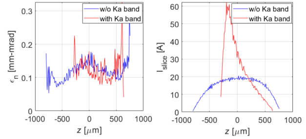
Figure 4: Electron beam slice analysis in terms of emittance (left) and peak current (right) at the photo-injector exit spaces with (red line) and without (blue line) the Ka-band linearizer.
