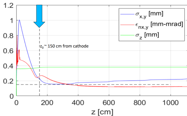
Figure 3: Evolution of the electron beam transverse normalized emittance (red line), transverse spot size (blue line) and bunch length (green line) without linearizer until the photo-injector exit.
