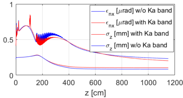
Figure 6: Evolution of the electron beam transverse normalized emittance and bunch length with (red line) and without (blue line) the Ka-band linearizer until the photo-injector exit.
