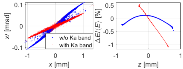
Figure 5: Transverse and longitudinal phase space at the photo-injector exit spaces with (red line) and without (blue line) the Ka-band linearizer.
