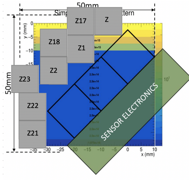
Figure B.3: Irradiation profile for TILE 6.
