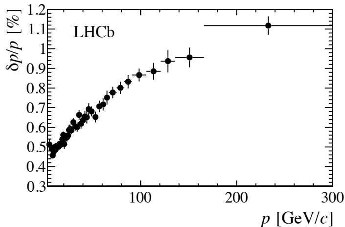
Figure 3.9: Relative momentum resolution versus momentum for long tracks in data obtained using J/\psi decays. Figure from [88].
