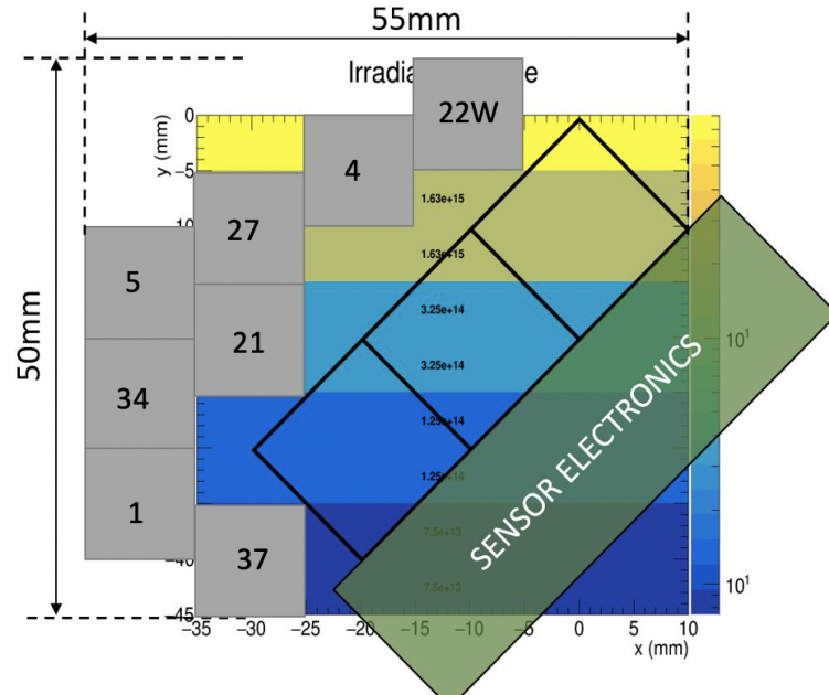
Figure B.2: Irradiation profile for the TILE 5.
