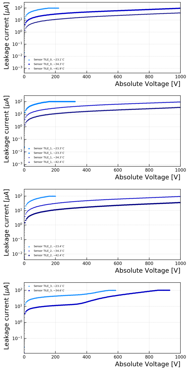
Figure 4.11: IV temperature dependence for the IRRAD sensors: TLE 0, TLE 1, TLE 2 and TLE 3
