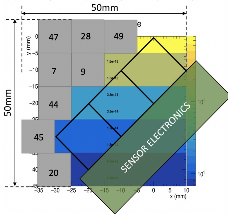
Figure B.1: Irradiation profile for the TILE 4.
