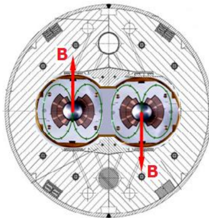
Figure 3.2: Transverse cross section of cryostat housing LHC twin dipole magnet. Extracted from [83].
