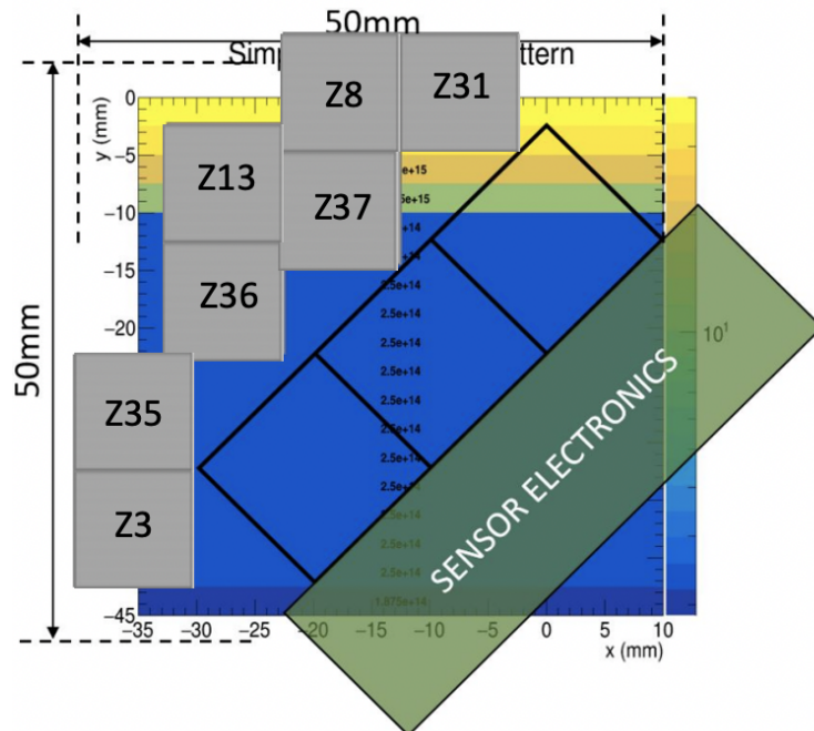
Figure B.4: Irradiation profile for TILE 7.
