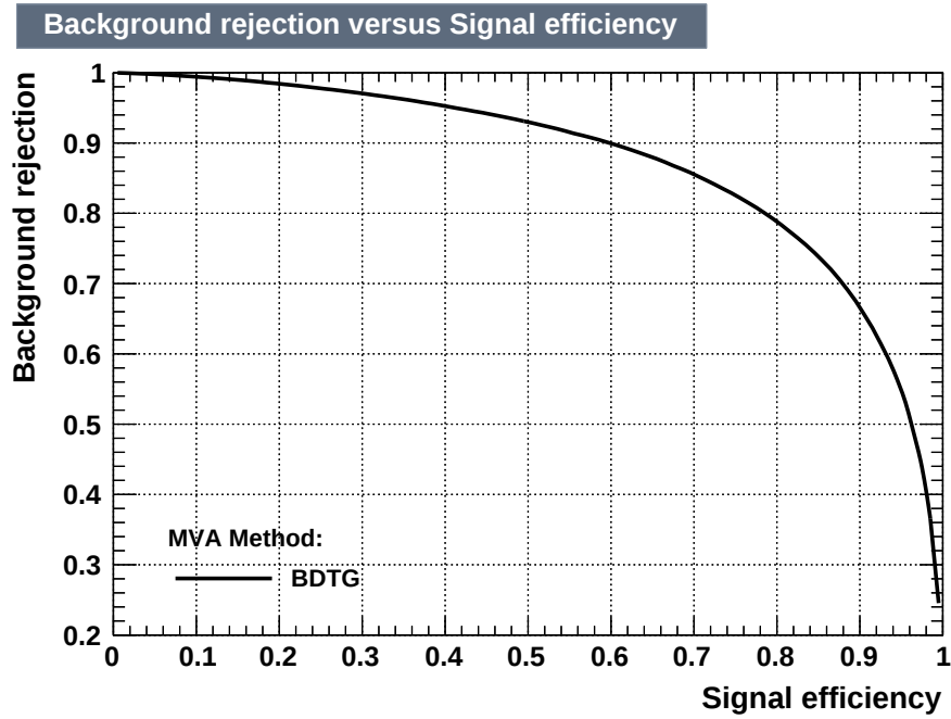
Figure 6.21: BDT background rejection vs signal efficiency.
