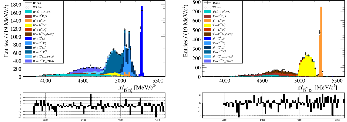
Figure 7.1: \bar{D}^0 D_s^+ (left) and D^{*-} D_s^+ (right) sub-samples invariant mass data and PDF after fitting.
