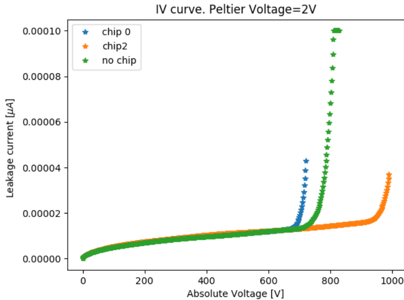
Figure 4.14: IV curves with PT100 attached in different chips of the TILE 5 at -38^{\circ}\text{C} .
