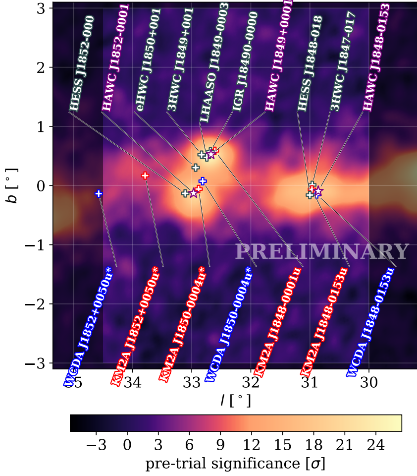
Figure 1: HAWC pre-trial significance map with an spectral index of 2.7 using data within 1 TeV – 316 TeV. The black labels are taken from TeVCat, and the purple labels are the three sources found from this work. 1LHAASO sources are denoted as WCD A (blue) and KM2A (red) by their independent measurement of positions.
