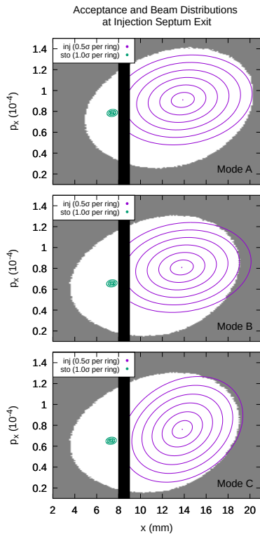
Figure 2: Injected and stored beam profiles out to 3\sigma at septum exit during an injection cycle. The white region is the acceptance in x - x' space at the septum exit. The x - x' space septum image is drawn in black and is 1 mm thick with its inward edge 8 mm from the stored beam reference trajectory.
