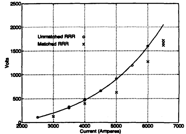
Fig. 2. Comparison of the measured maximum voltage to ground observed in Runs 1&2 (unmatched RRR, variation ~2) versus those measured in Run 3 (matched RRR, variation ~10%).
