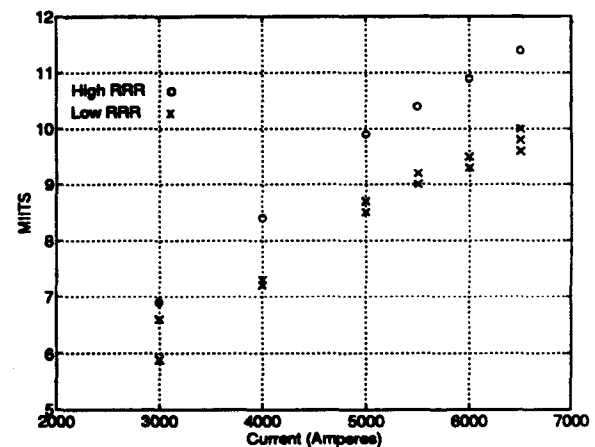
Fig. 3. MIITS values calculated from the measured current profiles versus maximum string current for strip heater induced events showing that high RRR magnets experience higher MIITS than low RRR magnets due to the resulting longer current decay times.
