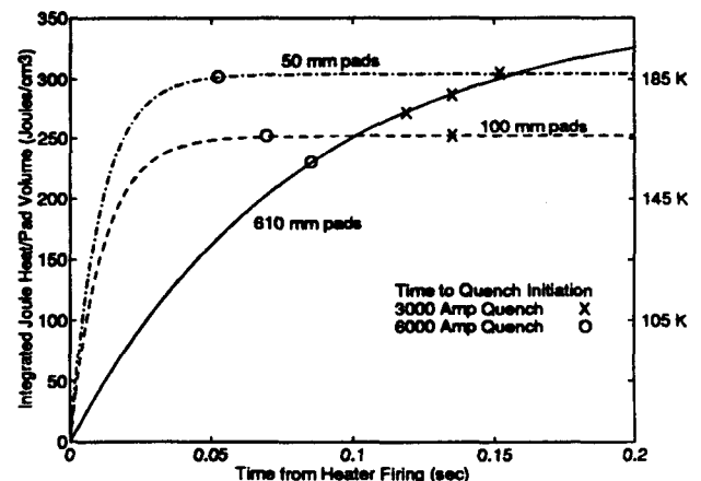
Fig. 4. Integrated Joule heating energy per unit heater pad volume giving the total energy density in the strip heaters from the time of heater firing as a function of time.
