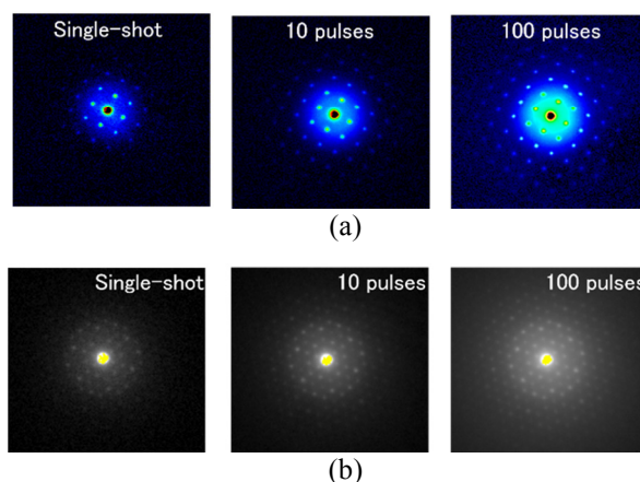
Figure 4: Relativistic-energy electron diffractions observed from single-crystal gold (a) and single-crystal Mica (b) with single-pulse, 10-pulse and 100-pulse averaging measurements.
