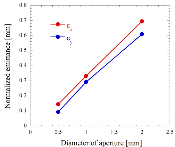
Figure 2: The normalized transverse emittance of the femtosecond electron beam generated from the RF gun as a function of the aperture diameter.
