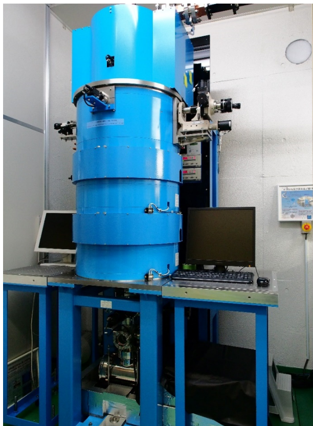
Figure 3: The prototype of RF gun based relativistic-energy electron microscopy which was constructed at Osaka University in 2012 and improved in 2014.
