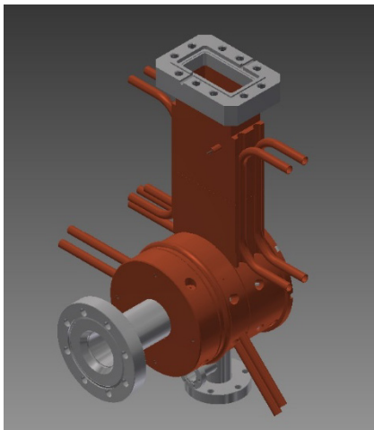
Figure 1: New photocathode RF gun for electron microscopy.
