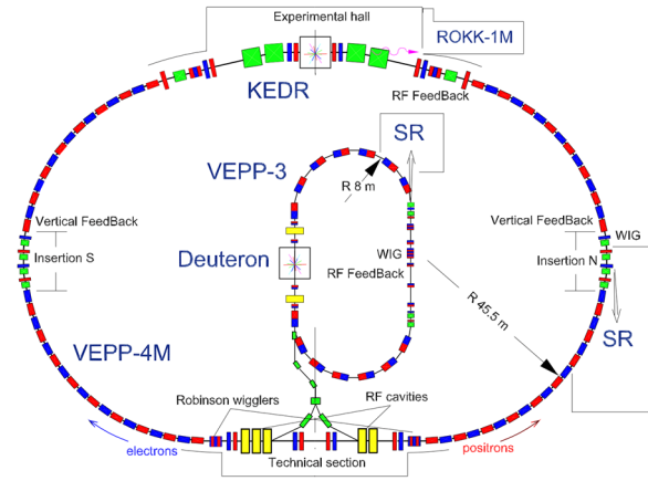
Figure 1: VEPP-4 layout.
