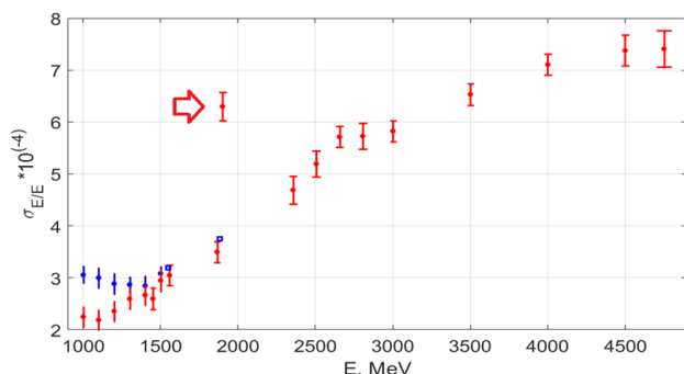
Figure 3: VEPP-4M beam energy spread in energy range 1000 – 4750 MeV.
