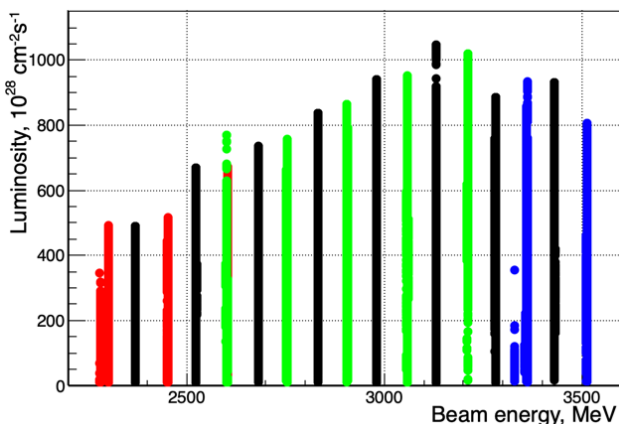
Figure 2: The luminosity in R-scan 2.3÷3.5 GeV.
