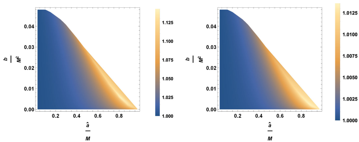
Fig. 22 For the left panel the inclination angle is 90^\circ and for the right panel the inclination angle is 17^\circ
