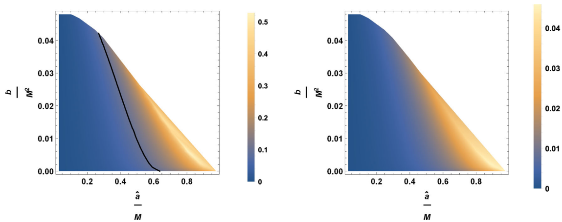
Fig. 20 For the left panel the inclination angle is 90^\circ and for the right panel the inclination angle is 17^\circ . The black solid lines correspond to \Delta C = 0.1
