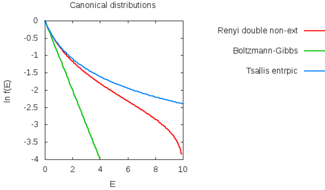
Fig. 1. (Color online) Canonical distributions in classical and generalized thermodynamics (schematic curves).
