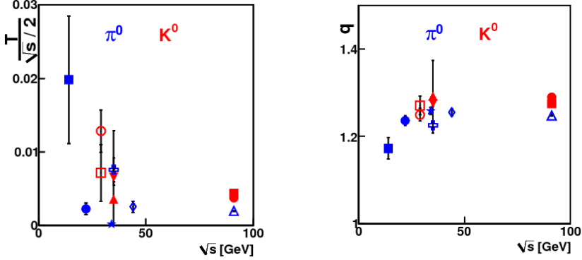
Fig. 3. Fitted values of the T and q parameters in Eq. (14) with D = 3 and N_0 = 1 + 1/D to measured fragmentation functions shown in Fig. 2.
