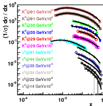
Fig. 2. Fragmentation functions of \pi^0 s and K^0 s measured at various collision energies (data, from top to bottom, are published in Refs. [13, 14, 15, 16, 17, 18, 19, 20, 21, 22, 22, 22]) and fitted with microcanonical Tsallis–Pareto distributions (Eq. (14) with D = 3 and N_0 = 1 + 1/D ).
