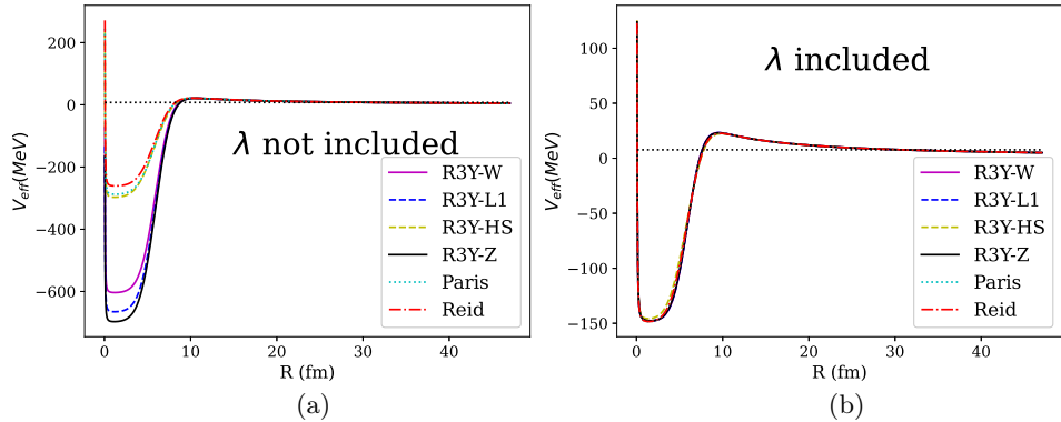
Fig. 1. Plot of the effective \alpha -nucleus potential V_{\text{eff}} for ^{190}\text{Po} using the density-independent (DD0) R3Y-W, R3Y-L1, R3Y-HS, R3Y-Z, M3Y-Paris, and M3Y-Reid interactions. (a) quantization factor not applied and (b) quantization factor included.
