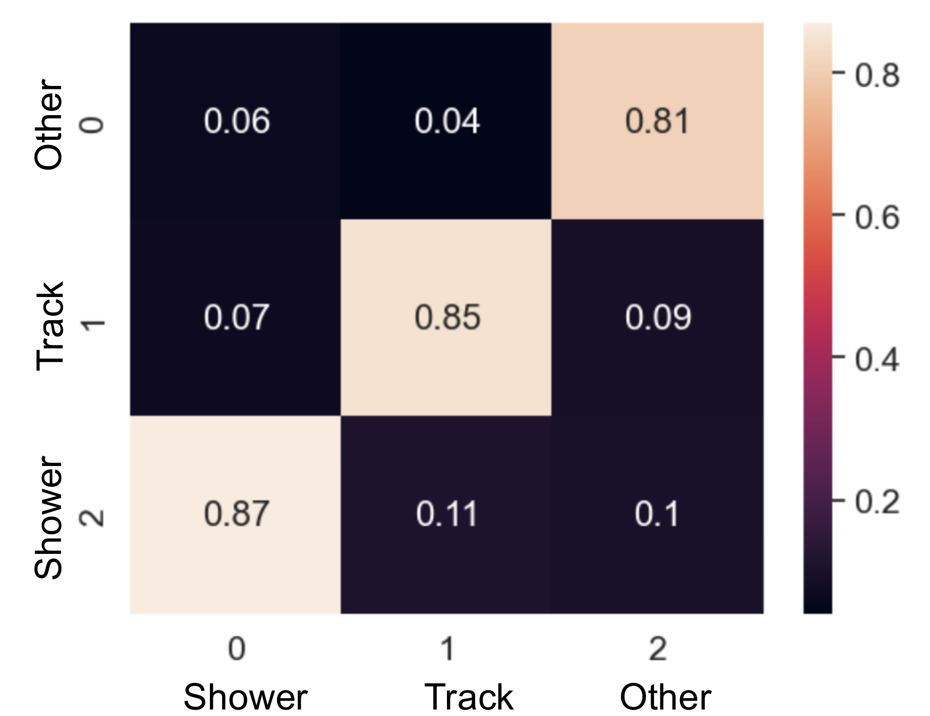
Fig 6: Preliminary performance results of sparse CNN approach.
