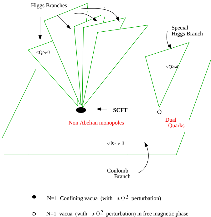
QMS of N=2 \text{USp}(2n) Theory with n_f Quarks
