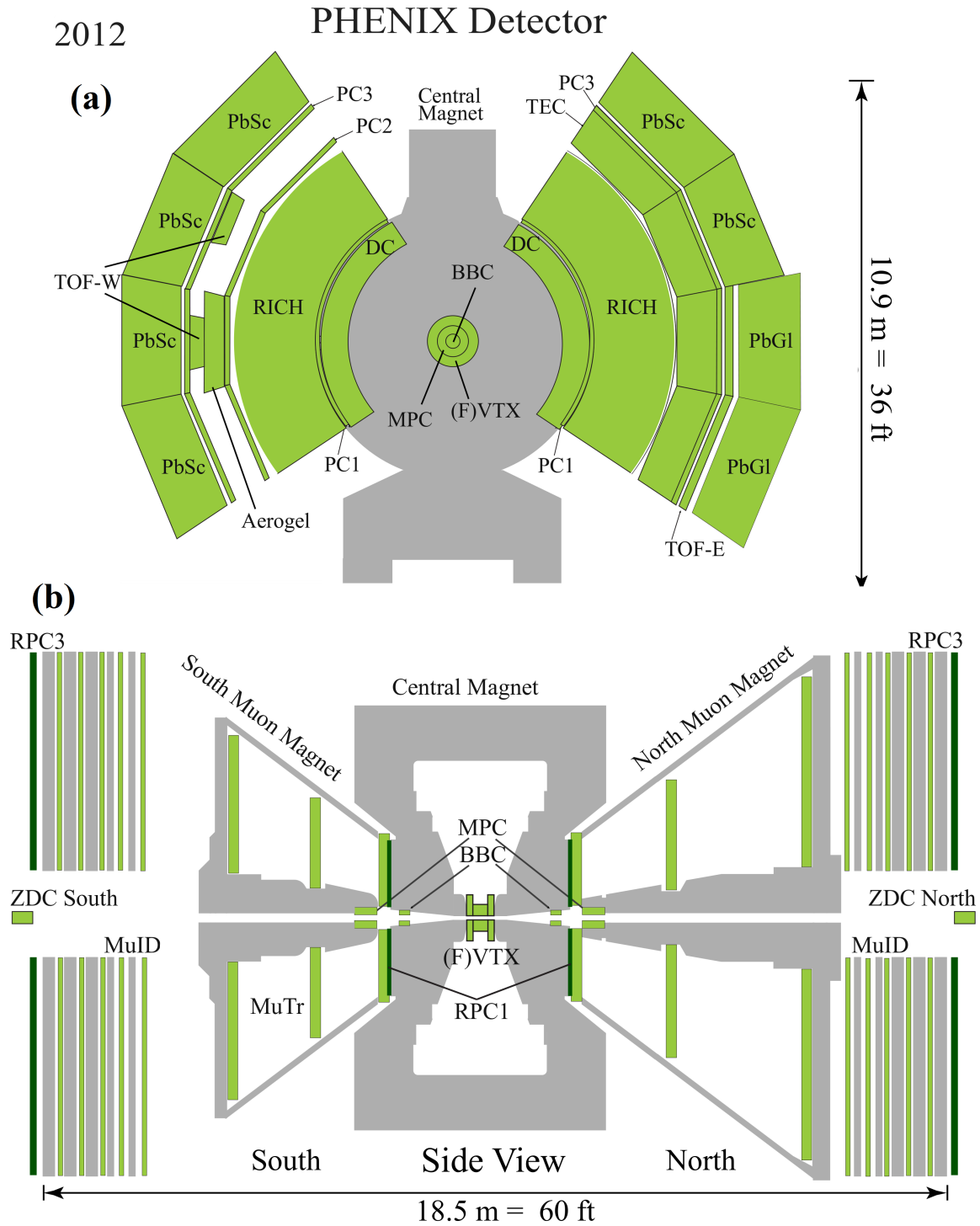
Figure 2.2. A schematic of the PHENIX detector, including the (a) central arms and (b) forward and backward muon arms during 2012.
