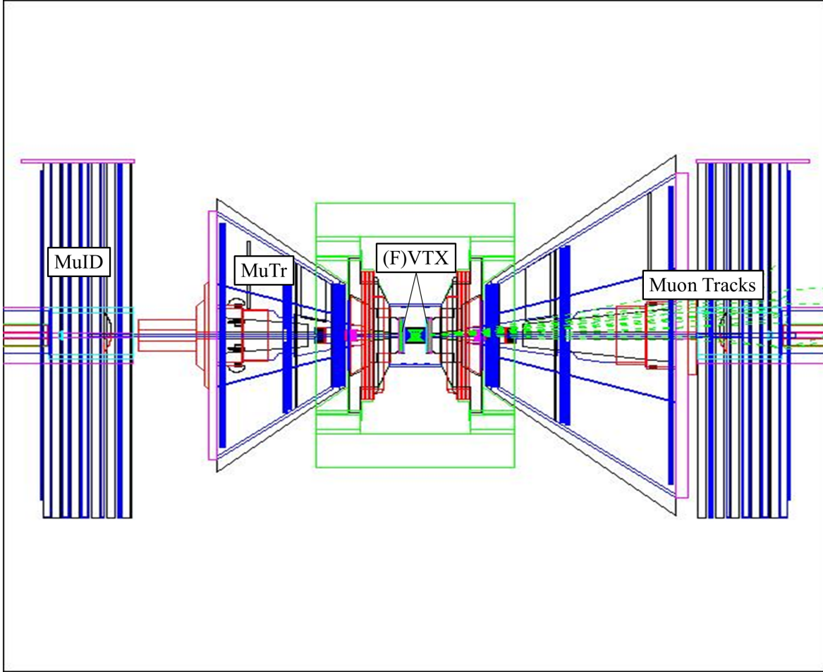
Figure 3.16. A PISA event display for muons of momentum 3.5 \text{ GeV}/c as they traverse the PHENIX detector in simulation. Muons generated in PHENIX collisions need at least p \sim 3 \text{ GeV}/c to make it to the back of the MuID.
