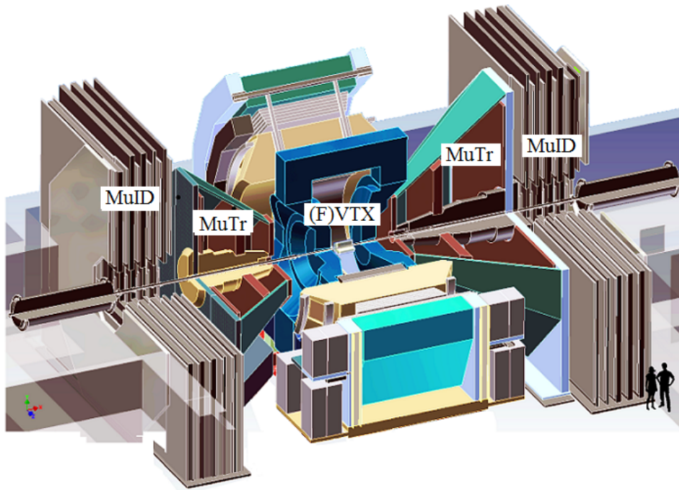
Figure 2.3. A cross-section of the PHENIX detector.
