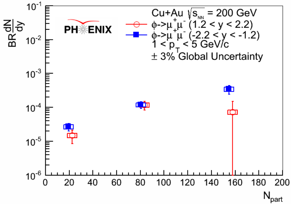
Figure 4.1. Invariant yield plotted as a function of the number of participating nucleons for 1.2 < |y| < 2.2 and 1 < p_T < 5 GeV/c.
