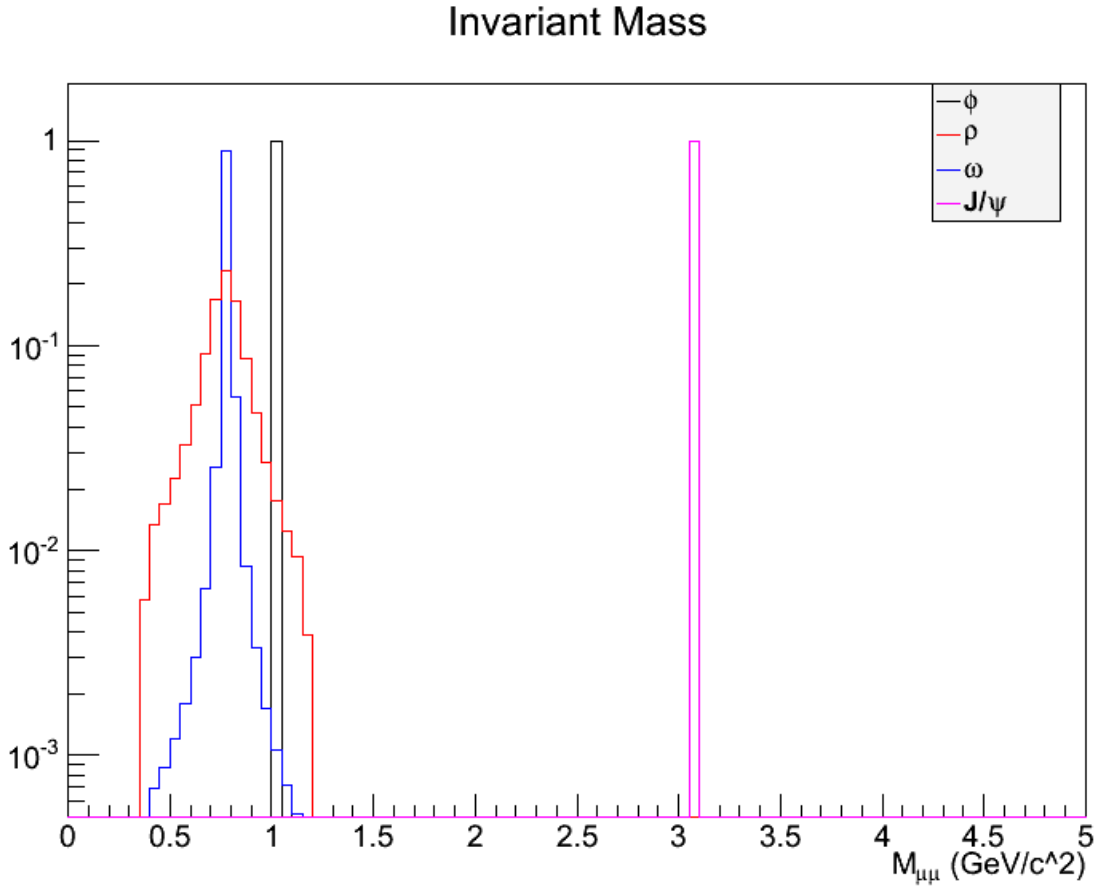
Figure 3.15. The mass distributions of the low-mass vector mesons, \phi (black), \rho (red), and \omega (blue), and the J/\psi meson (pink) at the PYTHIA-level.
