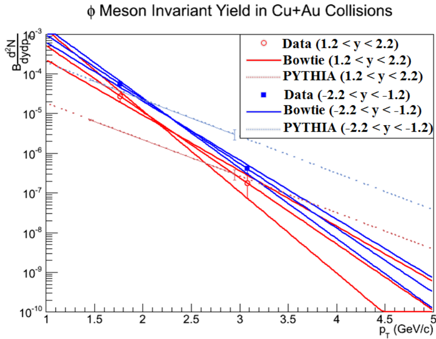
Figure 3.19. The transverse momentum distributions in real data (solid) and the PYTHIA simulation (dashed) for both forward rapidity (red) and backward rapidity (blue). The PYTHIA distributions are altered to match real data over the error bars.
