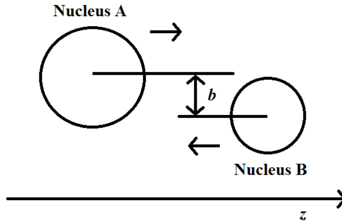
Figure 1.4. Schematic of the collision of two nuclei separated by impact parameter b .
