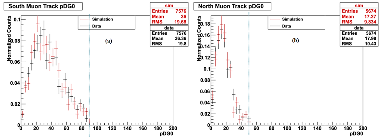
Figure 3.28. pDG0 distributions for reconstructed \phi mesons in real data (black) and in the PISA simulation (red). The quality cut is represented by the dotted line.
