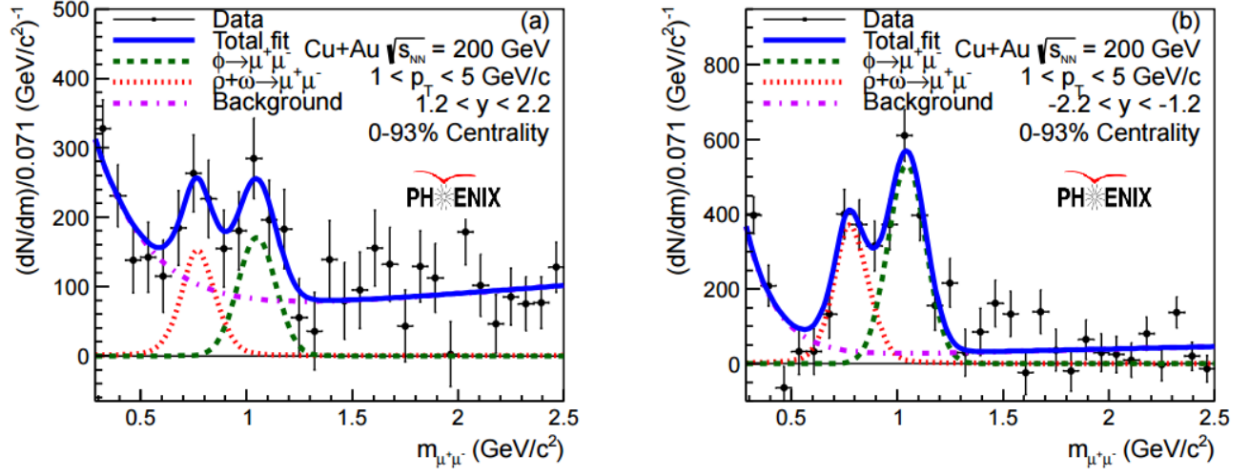
Figure 3.14. The dimuon mass spectra after mixed-event background subtraction for forward rapidity (a) and backward rapidity (b).
