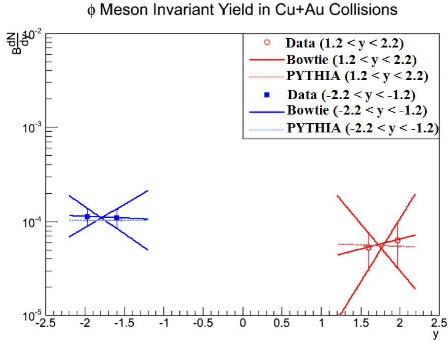
Figure 3.20. The rapidity distributions in real data (solid) and the PYTHIA simulation (dashed) for both forward rapidity (red) and backward rapidity (blue). The PYTHIA distributions are altered to match real data over the error bars.
