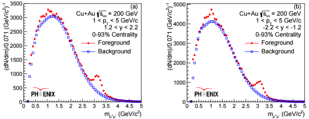
Figure 3.13. The mass distribution at forward rapidity (a) and backward rapidity (b) prior to background subtraction. The foreground is represented by red, closed circles, while the background is blue, open squares.
