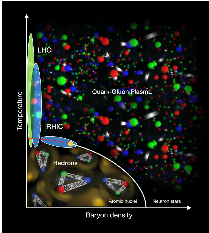
Figure 1.12. The QCD phase diagram.
