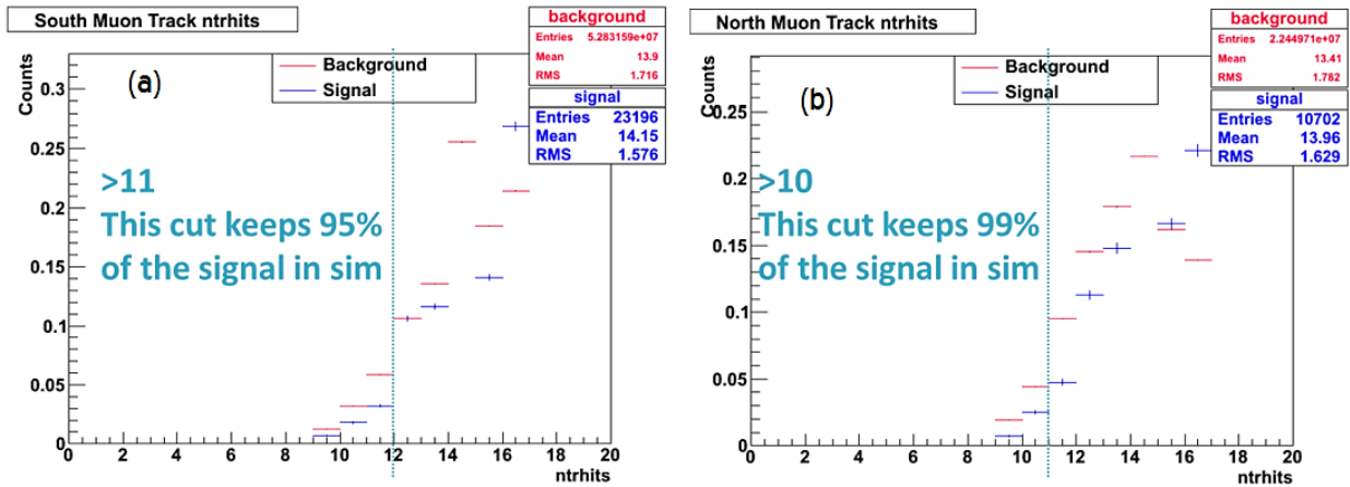
Figure 3.7. Single muon ntrhits distribution for the backward arm (a) and forward arm (b) and the associated quality cut. The distributions are plotted in blue for the \phi meson signal, which comes from simulation, and in red for the background, which comes from real data.
