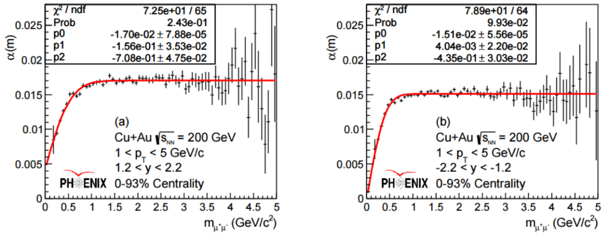
Figure 3.12. The normalization factor as a function of mass. The mass dependence of \alpha is clearly visible in the low-mass region where the \phi meson lies. The data is shown in black and the fit function is shown in red.
