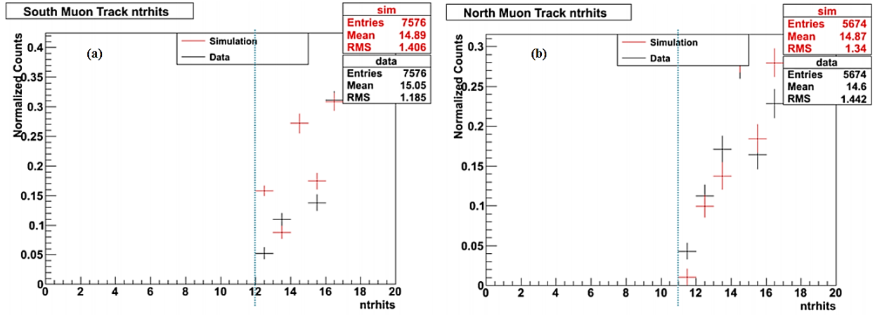
Figure 3.25. ntrhits distributions for reconstructed \phi mesons in real data (black) and in the PISA simulation (red). The quality cut is represented by the dotted line.
