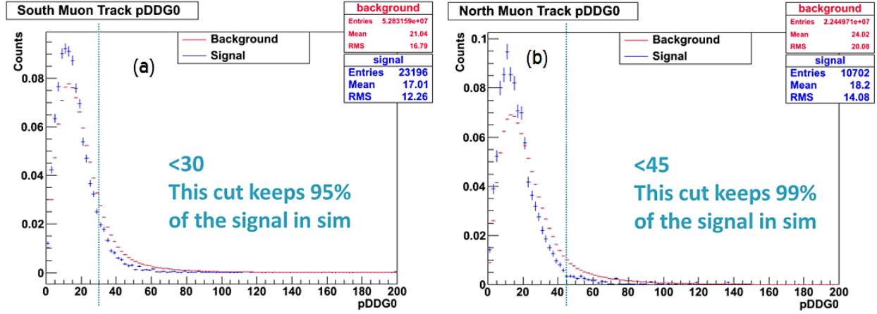
Figure 3.10. Single muon p_{DDG0} distribution for the backward arm (a) and forward arm (b) and the associated quality cut. The distributions are plotted in blue for the \phi meson signal, which comes from simulation, and in red for the background, which comes from real data.
