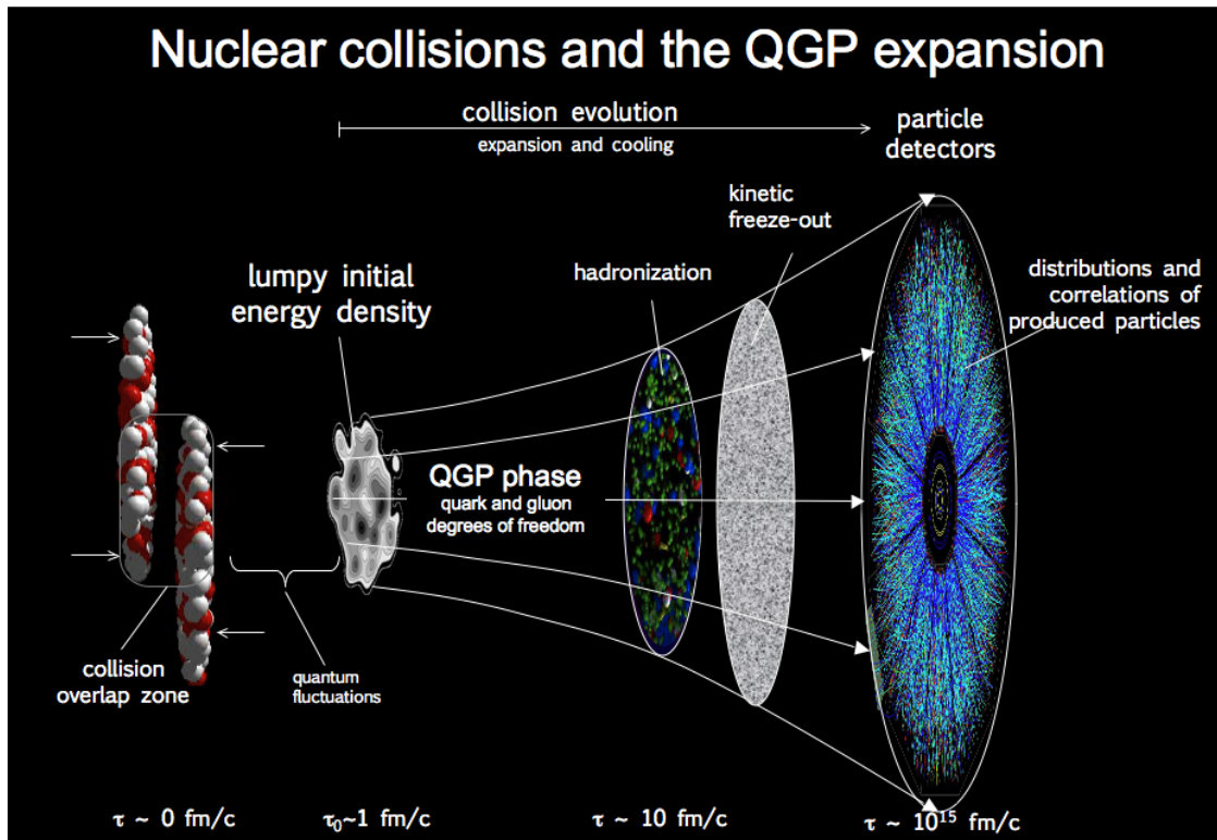
Figure 1.13. The time-evolution of a heavy-ion collision.
