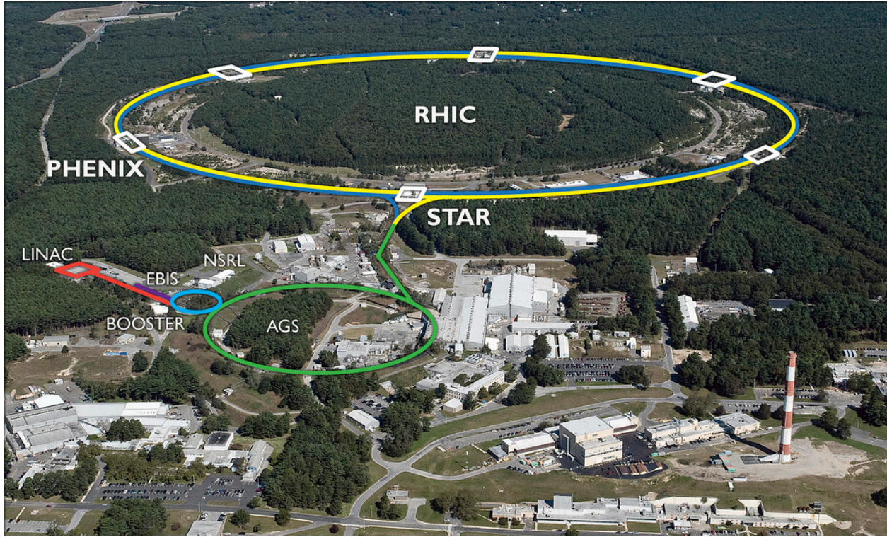
Figure 2.1. A diagram of the RHIC accelerator complex.
