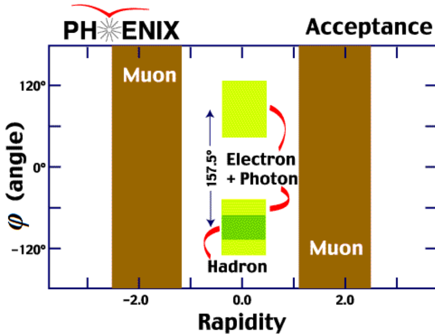
Figure 2.6. The acceptance of the PHENIX muon and central arms in \phi vs. y .
