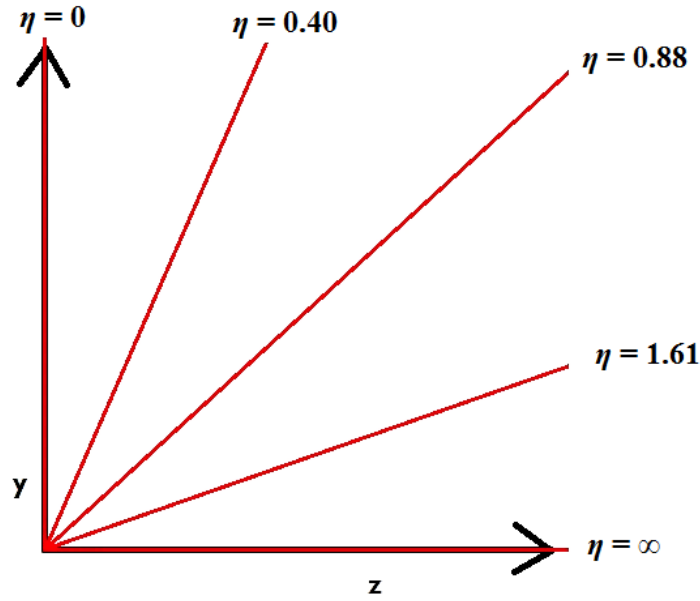
Figure 1.2. Pseudorapidity values for different angles from the beam axis.
