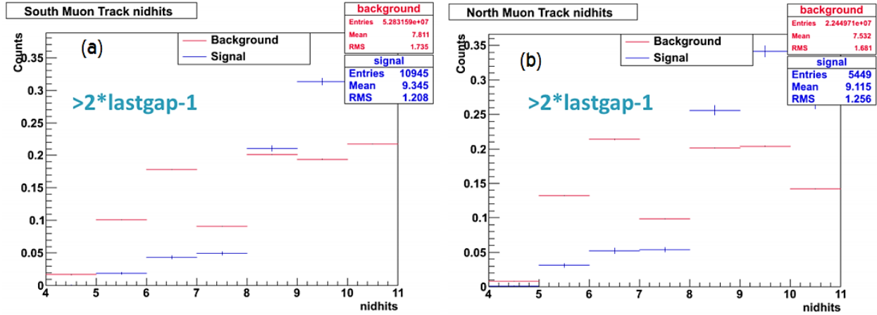
Figure 3.8. Single muon nidhits distribution for the backward arm (a) and forward arm (b) and the associated quality cut. The distributions are plotted in blue for the \phi meson signal, which comes from simulation, and in red for the background, which comes from real data.
