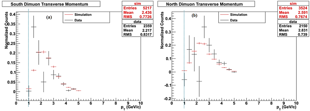
Figure 3.21. Transverse momentum distributions for reconstructed \phi mesons in real data (black) and in the PISA simulation (red). The quality cut is represented by the dotted line.
