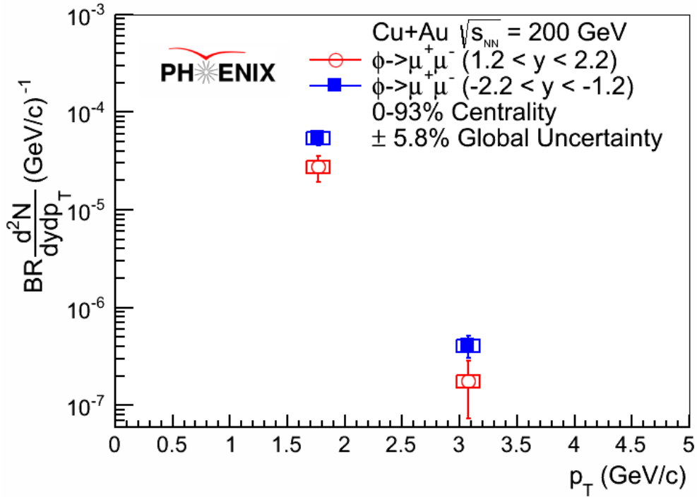
Figure 4.2. Invariant yield plotted as a function of transverse momentum for 1.2 < |y| < 2.2 and 0%-93% centrality.
