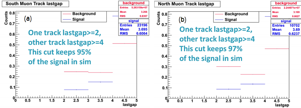
Figure 3.6. Single muon lastgap distribution for the backward arm (a) and forward arm (b) along with the associated quality cut. The distributions are plotted in blue for the \phi meson signal, which comes from simulation, and in red for the background, which comes from real data.
