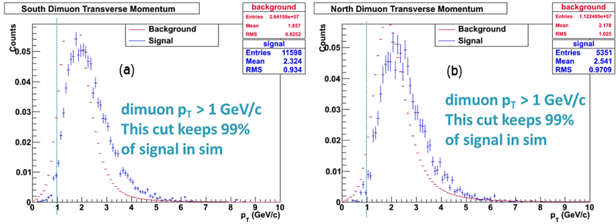
Figure 3.3. Dimuon transverse momentum and quality cut for the backward arm (a) and forward arm (b). The distributions are plotted in blue for the \phi meson signal, which comes from simulation, and in red for the background, which comes from real data.
