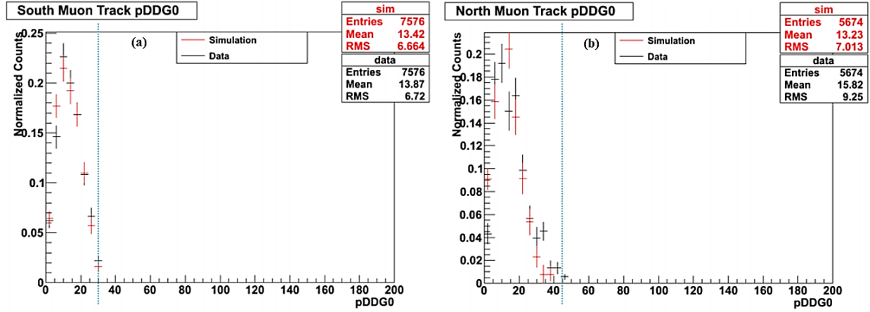
Figure 3.29. pDDG0 distributions for reconstructed \phi mesons in real data (black) and in the PISA simulation (red). The quality cut is represented by the dotted line.
