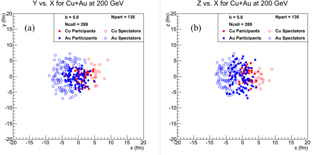
Figure 1.8. A typical Glauber event for Cu+Au collisions with b = 5.0 fm in (a) the xy -plane and (b) the xz -plane.
