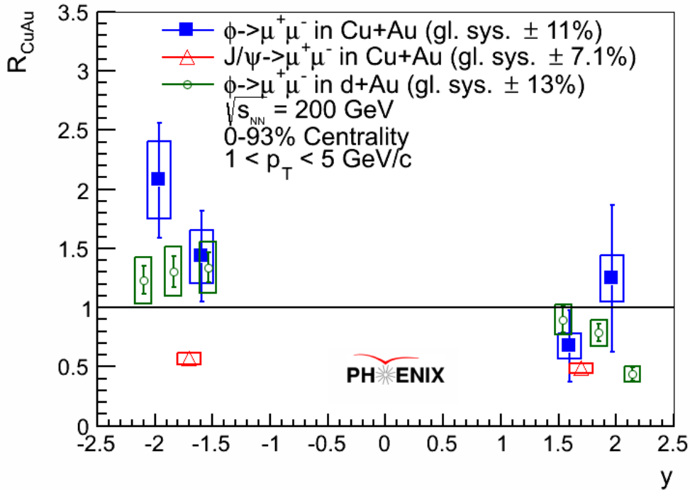
Figure 4.7. Nuclear-modification factor plotted as a function of rapidity for 1 < p_T < 5 GeV/ c and 0%-93% centrality.
