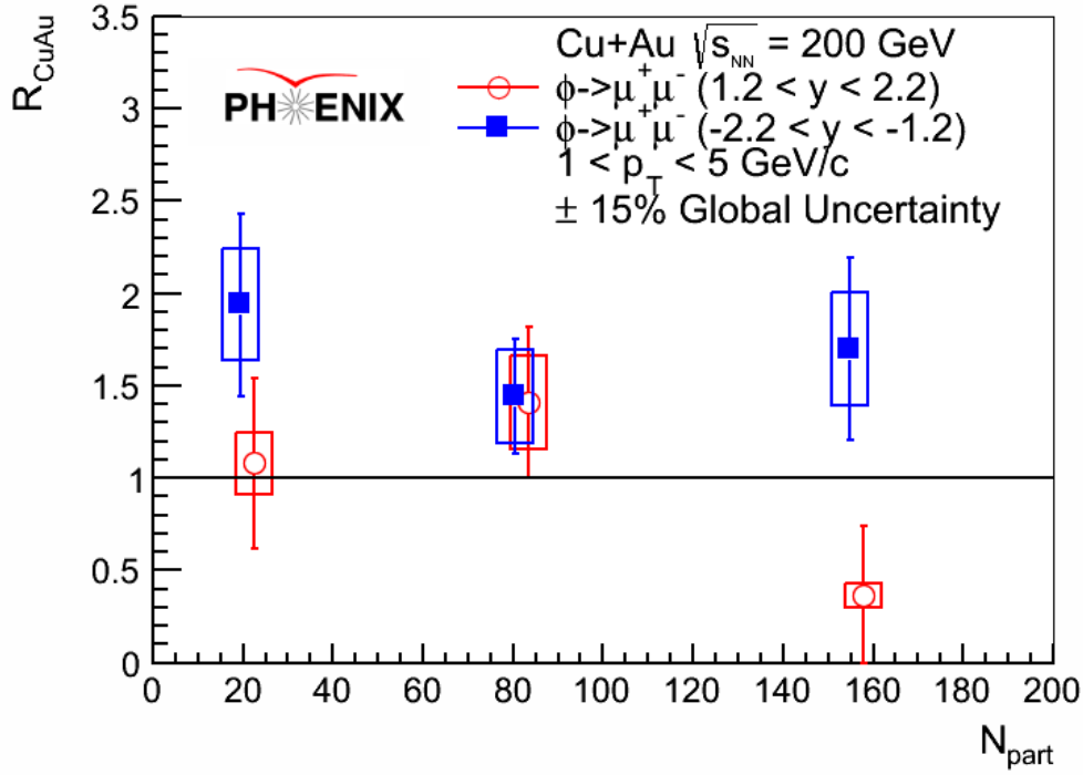
Figure 4.5. Nuclear-modification factor plotted as a function of the number of participating nucleons for 1.2 < |y| < 2.2 and 1 < p_T < 5 GeV/c.
