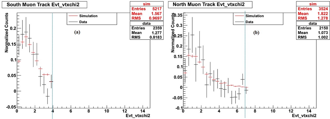
Figure 3.26. Vertex \chi^2 distributions for reconstructed \phi mesons in real data (black) and in the PISA simulation (red). The quality cut is represented by the dotted line.
