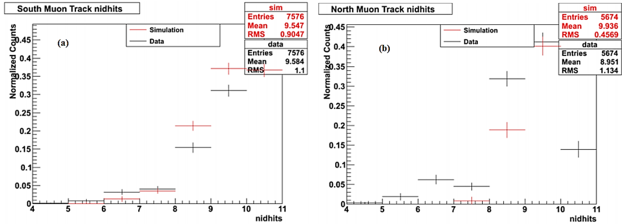
Figure 3.27. nIdhits distributions for reconstructed \phi mesons in real data (black) and in the PISA simulation (red).
