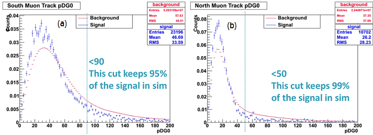
Figure 3.9. Single muon pDG0 distribution for the backward arm (a) and forward arm (b) and the associated quality cut. The distributions are plotted in blue for the \phi meson signal, which comes from simulation, and in red for the background, which comes from real data.
