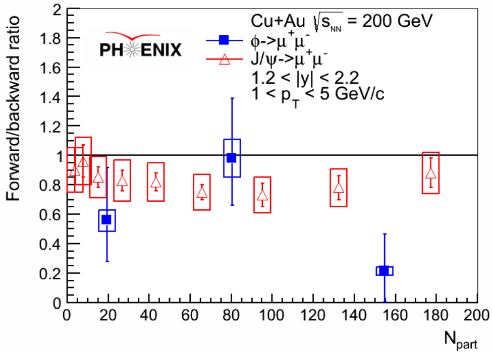
Figure 4.4. The forward/backward ratio as a function of the number of participating nucleons for 1.2 < |y| < 2.2 and 1 < p_T < 5 GeV/c.
