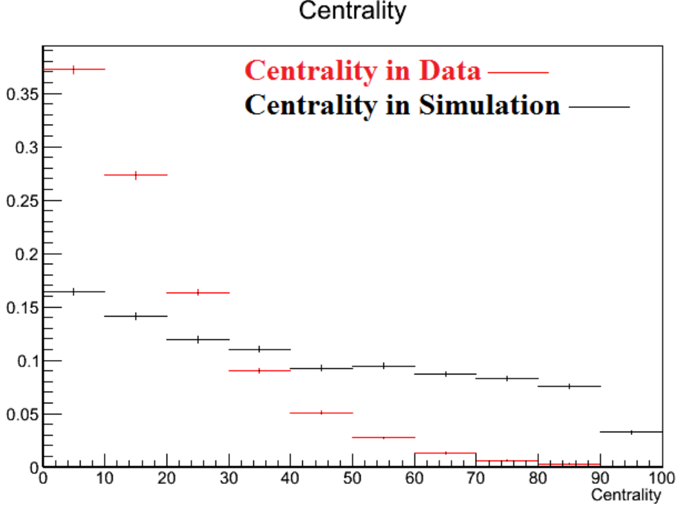
Figure 3.17. The centrality distributions of \phi mesons in simulation (black) and in real data (red). This is for unlike-sign same-event dimuons in the resonance region with all cuts applied.
