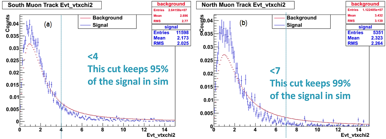
Figure 3.11. Vertex \chi^2 distributions for the backward arm (a) and forward arm (b) and the associated quality cut. The distributions are plotted in blue for the \phi meson signal, which comes from simulation, and in red for the background, which comes from real data.
