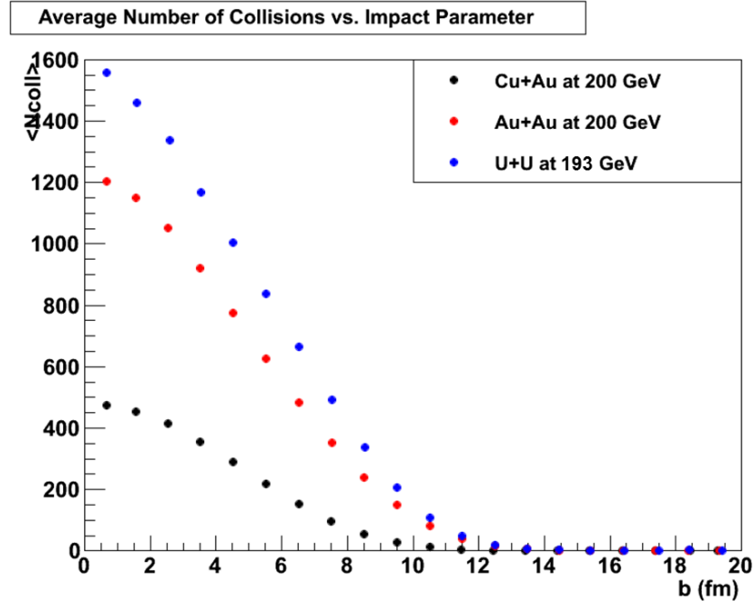
Figure 1.9. Average number of binary collisions as a function of impact parameter.
