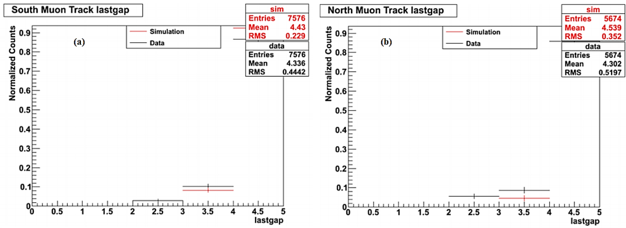
Figure 3.24. Lastgap distributions for reconstructed \phi mesons in real data (black) and in the PISA simulation (red).
