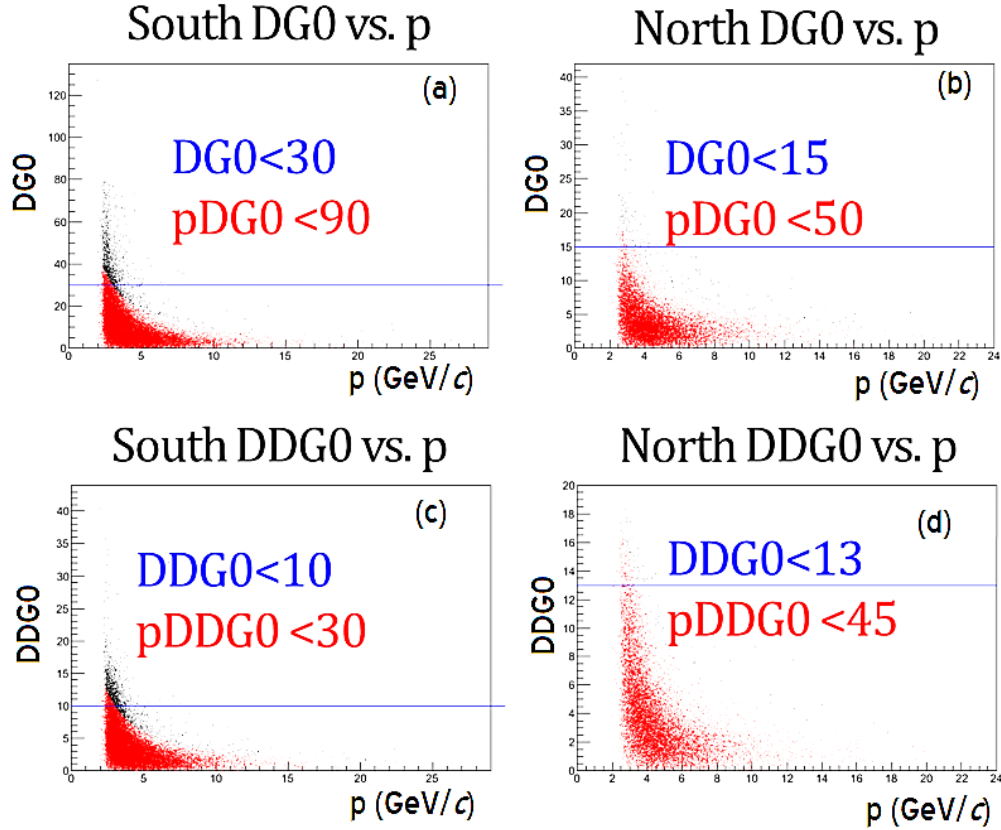
Figure 3.2. The momentum-dependent and momentum-independent cuts for DG0 and DDG0 .
