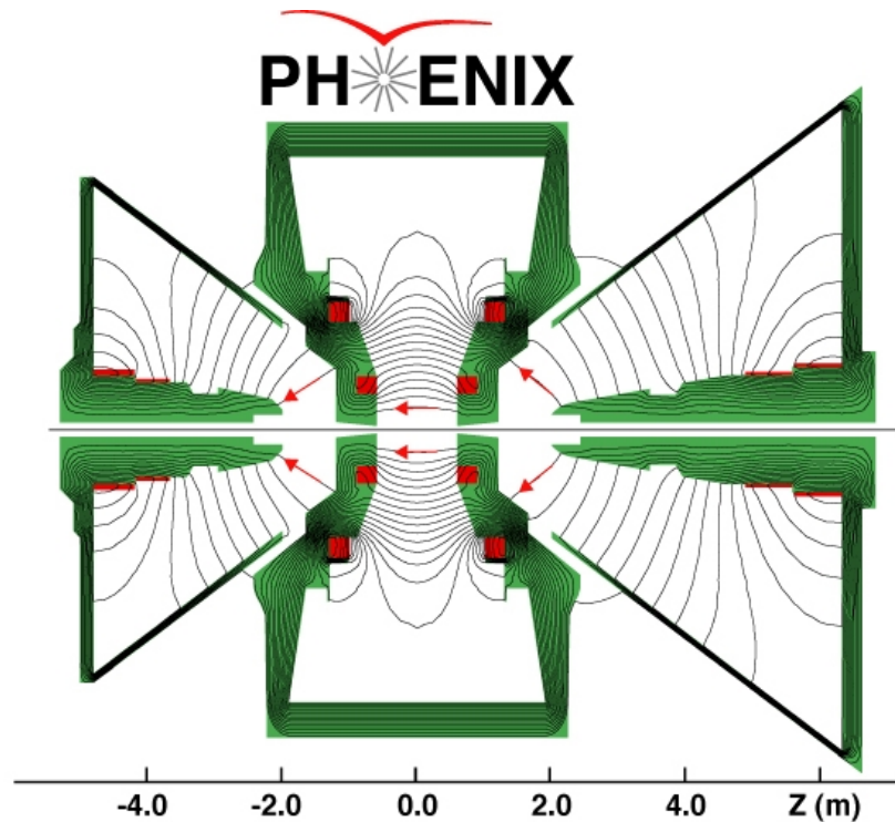
Figure 2.5. Magnetic field lines for the coils in combined (++) mode. This was the polarity used for taking data during the 2012 Cu+Au run at 200 GeV.
