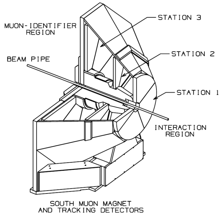
Figure 2.4. A schematic of the south muon magnet and MuTr detector showing the location of the three stations with respect to the beam pipe, MuID, and interaction region.
