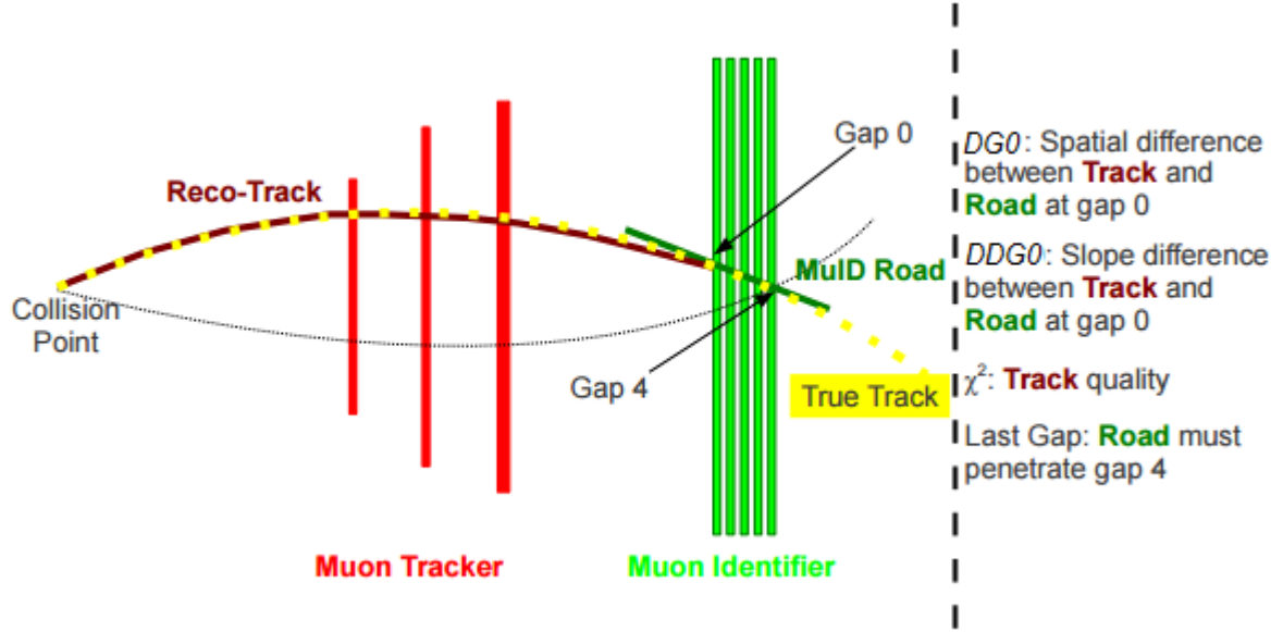
Figure 3.1. Schematic of the DG0 , DDG0 , and \chi^2_{tr} in the PHENIX muon arms
