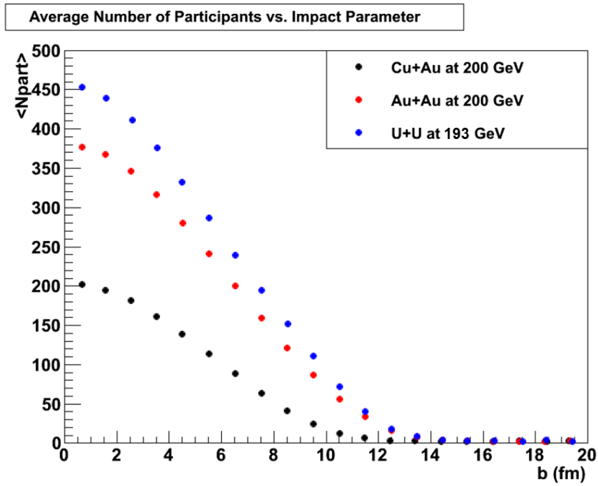
Figure 1.10. Average number of participating nucleons as a function of impact parameter.
