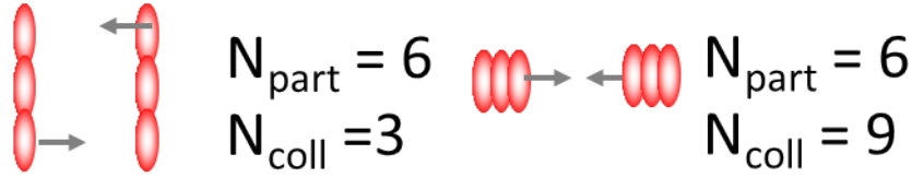
Figure 1.7. The number of participating nucleons and number of collisions for two different geometries.
