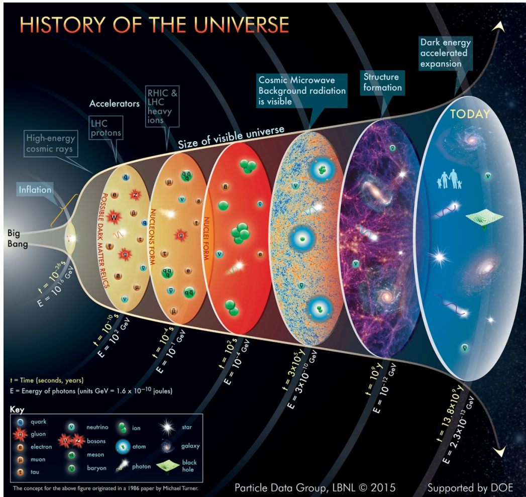
Figure 1.11. The time evolution of the universe from the Big Bang to present day.
