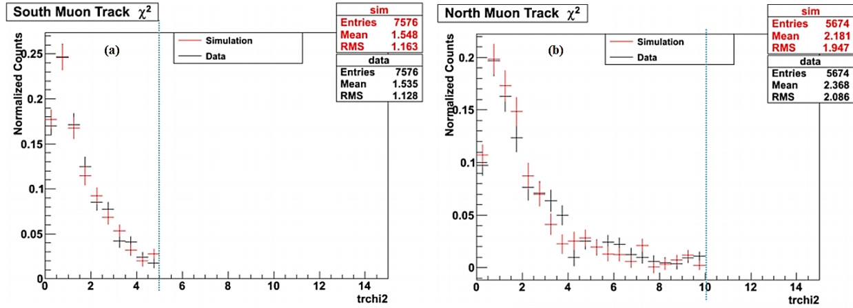
Figure 3.23. Track \chi^2 distributions for reconstructed \phi mesons in real data (black) and in the PISA simulation (red). The quality cut is represented by the dotted line.
