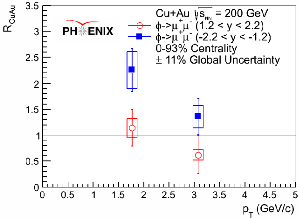
Figure 4.6. Nuclear-modification factor plotted as a function of transverse momentum for 1.2 < |y| < 2.2 and 0%-93% centrality.
