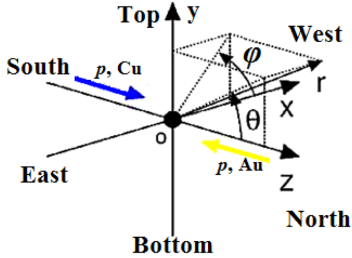
Figure 1.1. The global coordinate system for the PHENIX experiment with the Cu-going and Au-going directions clearly marked for this analysis.
