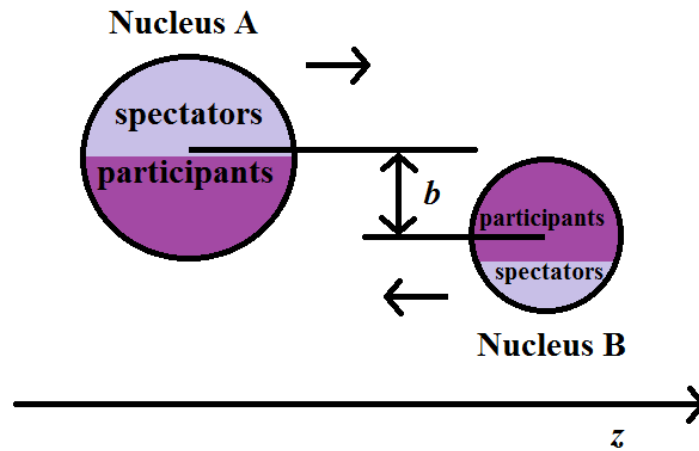
Figure 1.6. The regions of spectators and participants in nuclei A and B during a heavy-ion collision.
