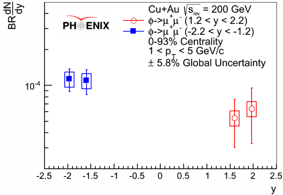
Figure 4.3. Invariant yield plotted as a function of rapidity for 0%-93% centrality and 1 < p_T < 5 GeV/c.
