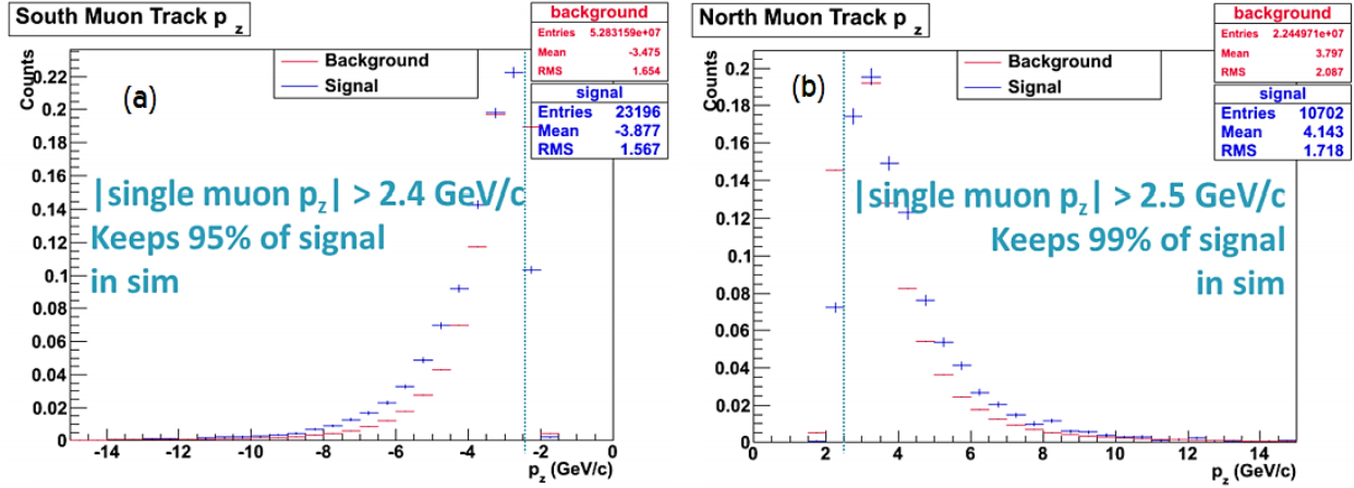
Figure 3.4. Single muon momentum along the z -axis for the backward arm (a) and forward arm (b) as well as the associated quality cut. The distributions are plotted in blue for the \phi meson signal, which comes from simulation, and in red for the background, which comes from real data.
