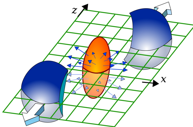
Figure 1.5. Sketch of the reaction plane in a heavy-ion collision.
