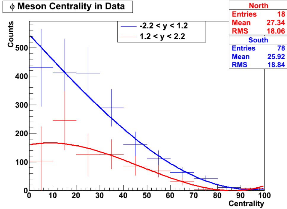
Figure 3.18. The centrality distribution for \phi meson candidates in real data for the north (forward rapidity) arm in red and the south (backward rapidity) arm in blue. Due to limited statistics, these distributions are fit with a polynomial.
