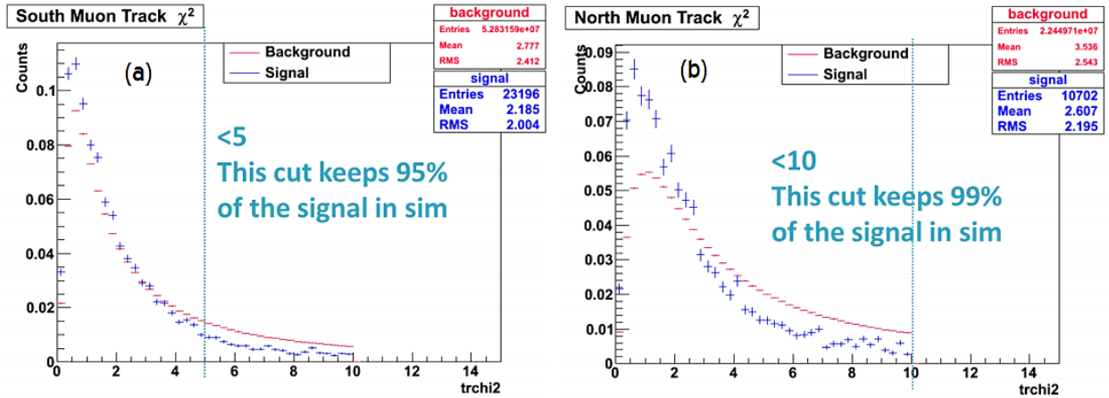
Figure 3.5. Track \chi^2 distributions for the backward arm (a) and forward arm (b) and the associated quality cut. The distributions are plotted in blue for the \phi meson signal, which comes from simulation, and in red for the background, which comes from real data.
