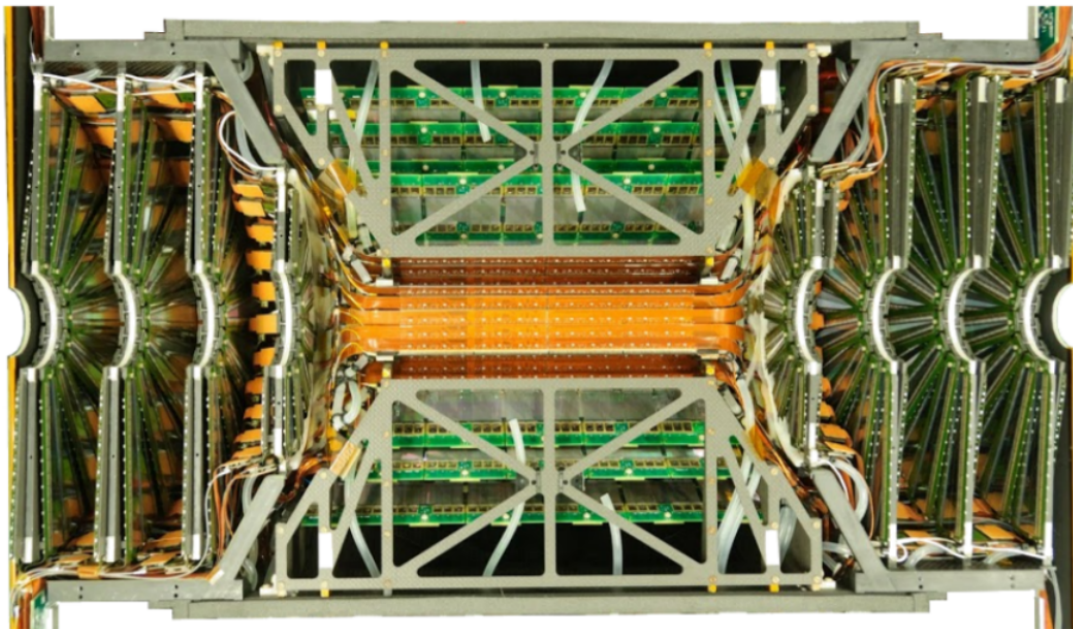
Figure 2.8. A photo of one-half of the combined VTX+FVTX detector system.
