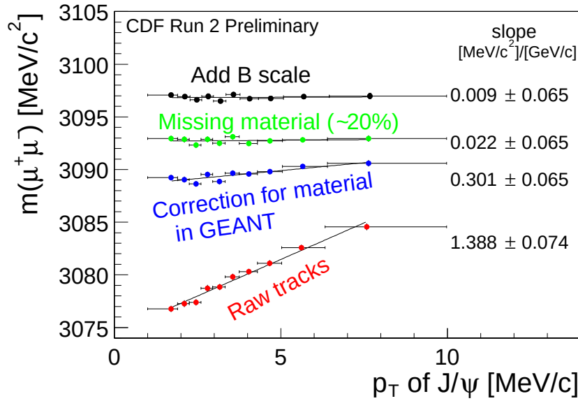
Figure 4.8: Dependence of the reconstructed invariant mass of J/\psi \rightarrow \mu^+\mu^- decays on the transverse momentum of the J/\psi .
