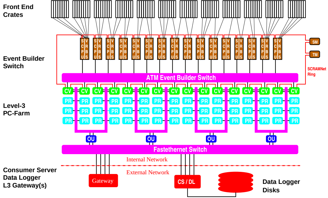
Figure 4.14: Event building and Level 3 operating principle: data from the front end crates is prepared by Scanner CPU's (SCPU) and fed into the ATM switch (purple). On the other side of the switch, converter nodes (green) assemble events and pass them to processor nodes. Accepted events are passed to output nodes (dark blue) which send them to the Consumer Server and data logging systems (red).
