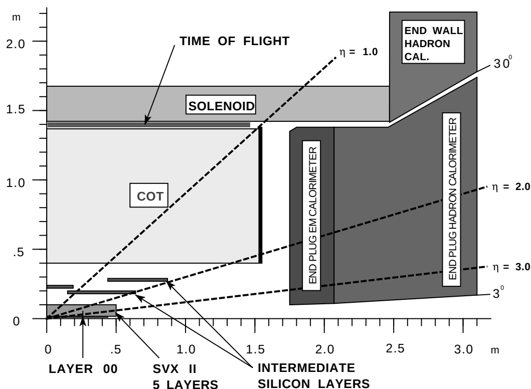
Figure 4.4: A diagram of the CDF-II tracker layout showing the different subdetector systems.
