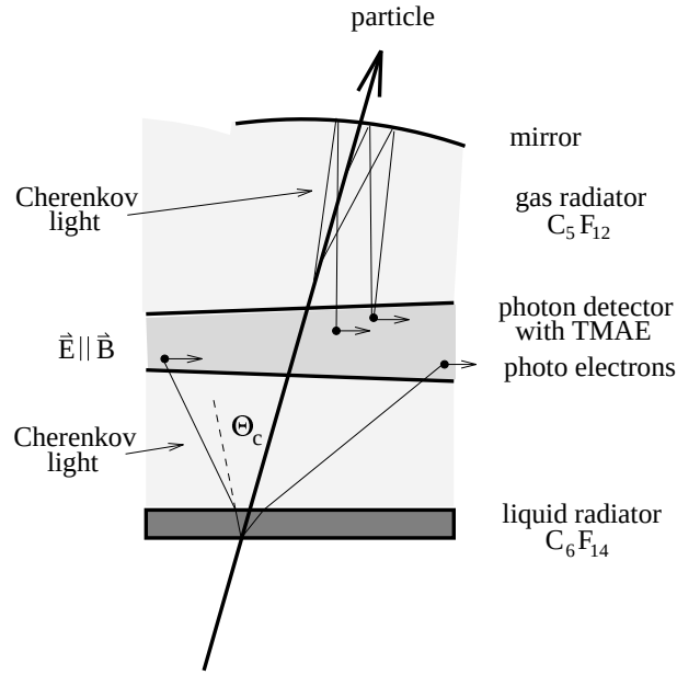
Figure 3.8: Operation principle of the RICH detector.
