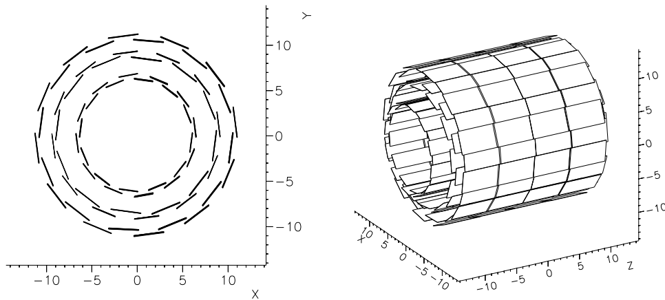
Figure 3.4: Schematic cross-sections of the DELPHI Vertex Detector (1994-1995 configuration).
