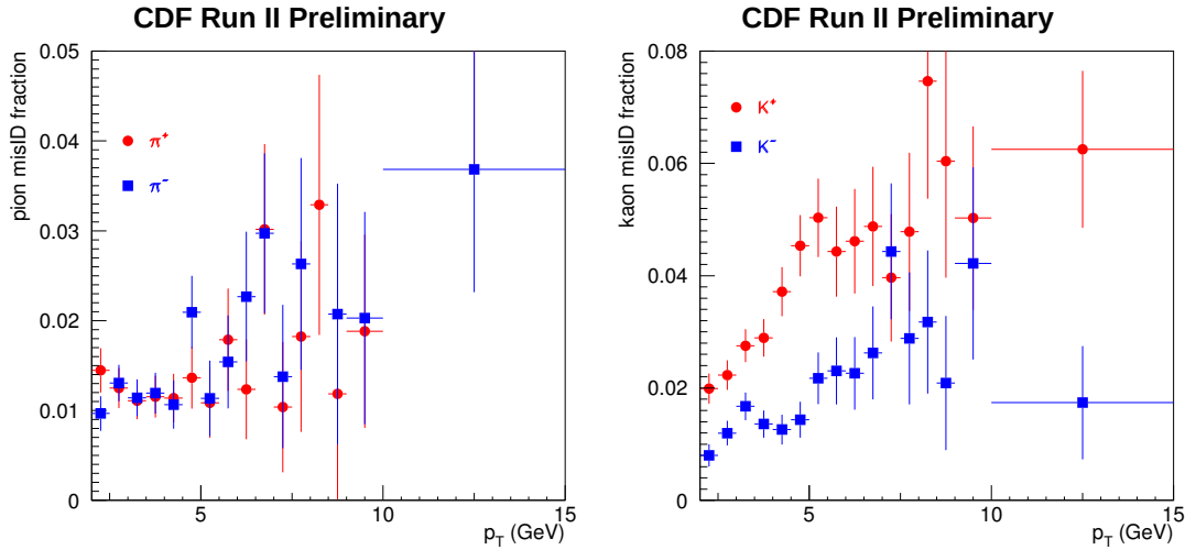
Figure 4.9: Rate of kaon and pion tracks faking muon signals in the CDF-II detector. Roughly 1% of all pions(left) and 2 – 4% of all kaons (right) will fake a muon signal.
