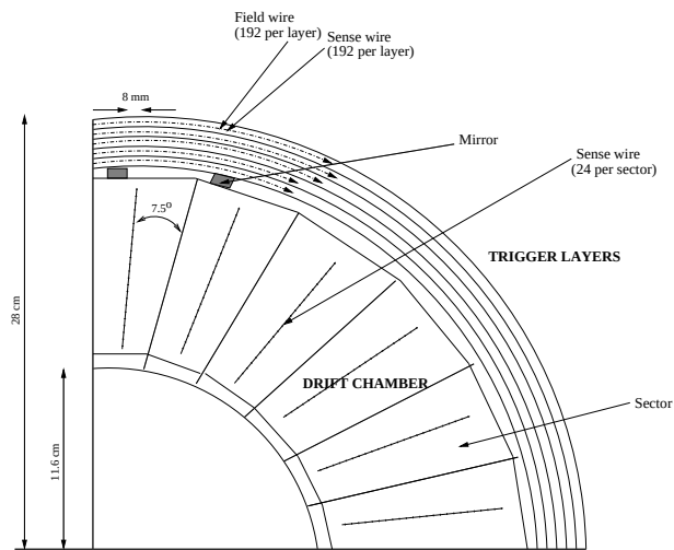
Figure 3.5: Scheme of DELPHI Inner Detector.
