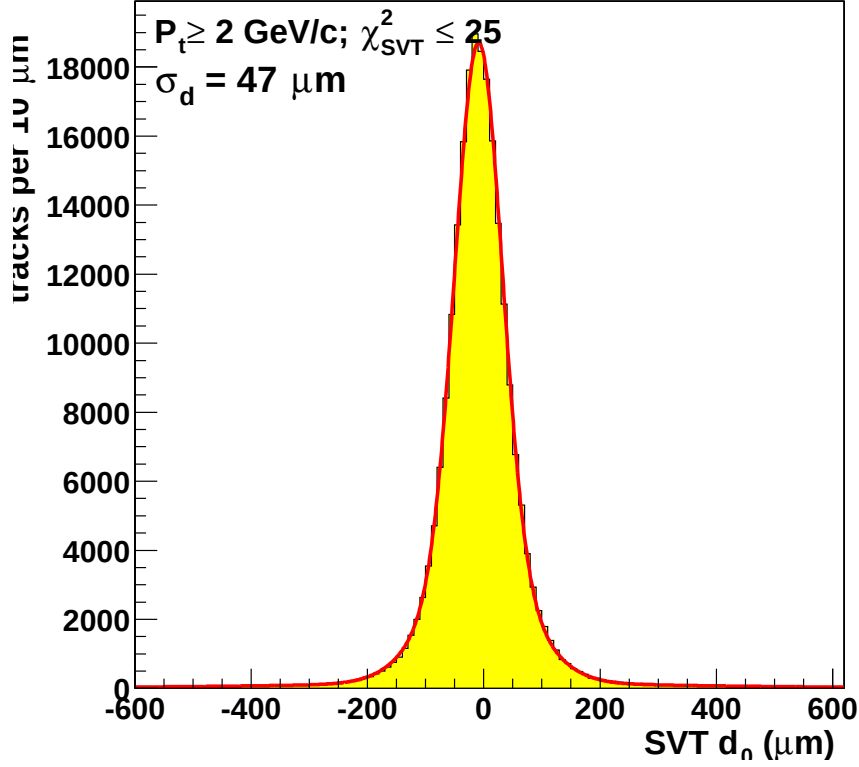
Figure 4.13: SVT impact parameter resolution.
