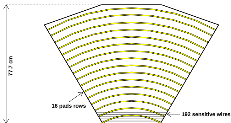
Figure 3.6: Schematic view of the sense wires and pads rows in one sector of the TPC.
