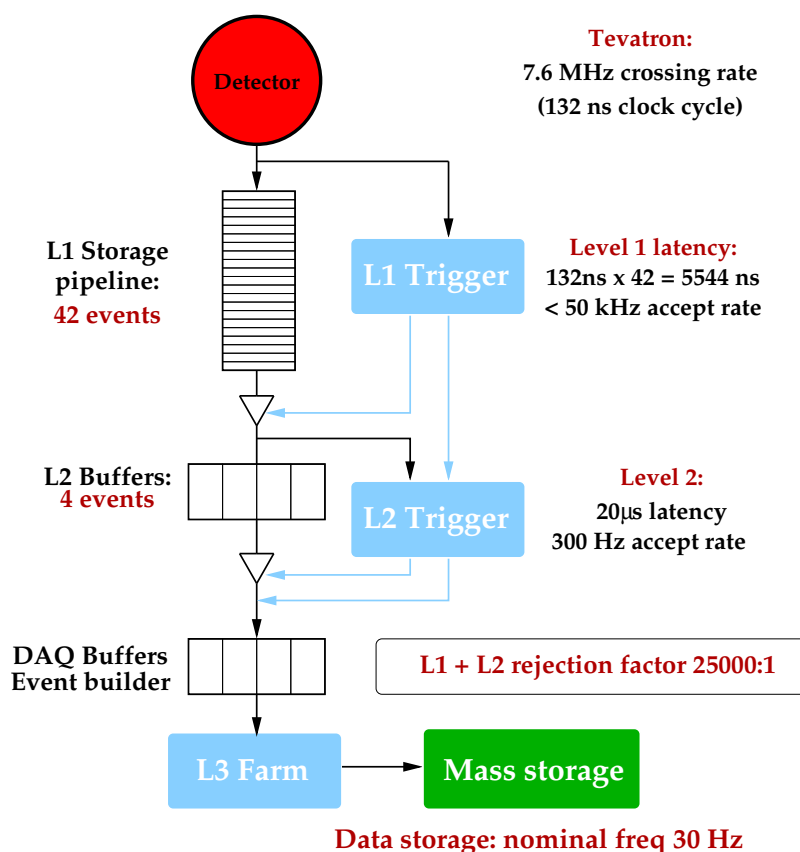
Figure 4.10: Diagram of the CDF-II trigger system.
