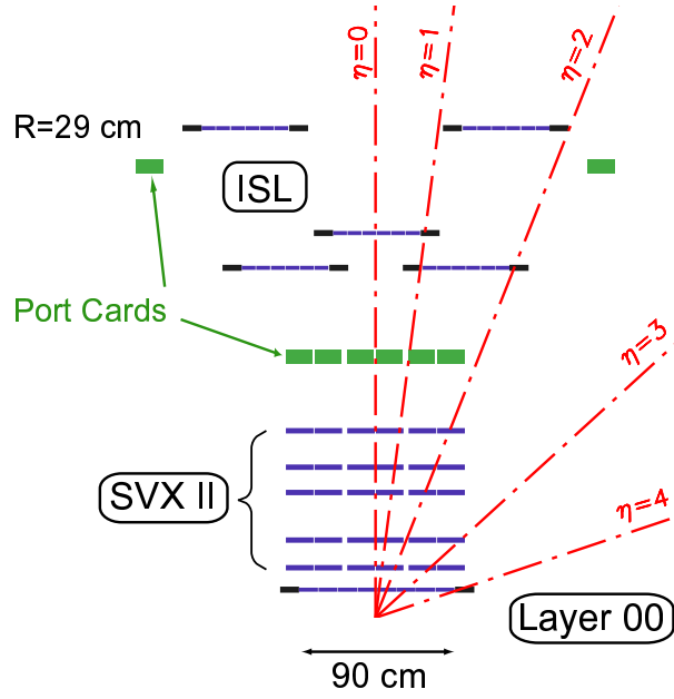
Figure 4.5: Coverage of the different silicon subdetector systems projected into the r - z plane. The r and z axes have different scales.
