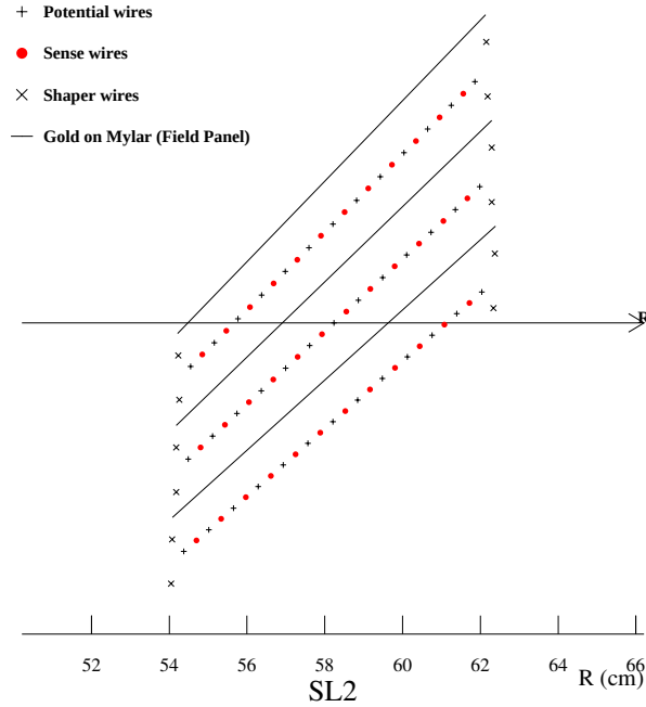
Figure 4.7: Layout of wires in a COT supercell.
