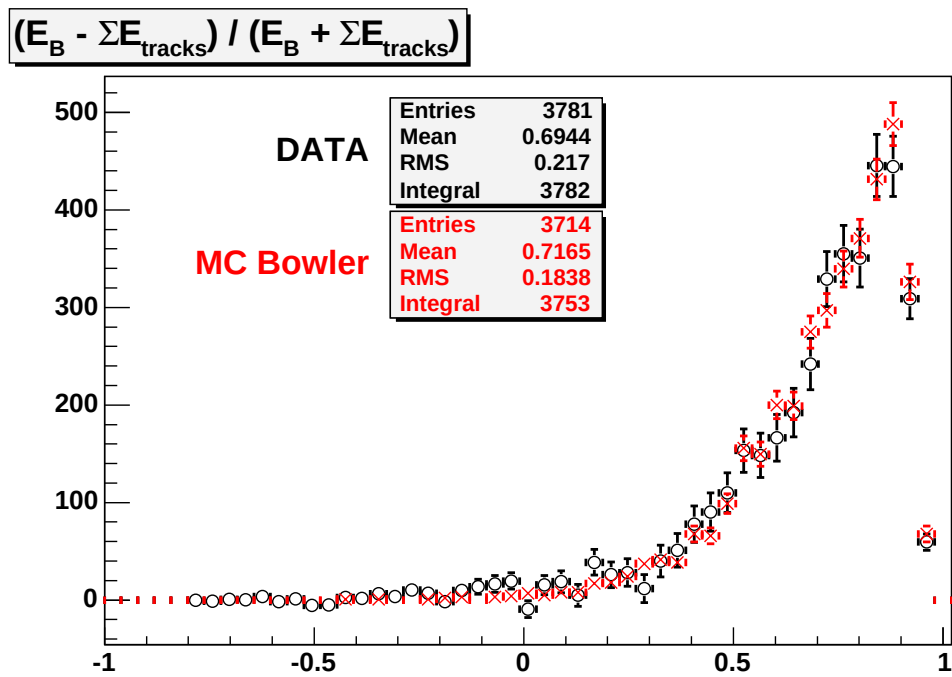
Figure 7.25: The distribution of the variable \frac{E_B - \Sigma E_{\text{tracks}}}{E_B + \Sigma E_{\text{tracks}}} , where the sum is over tracks in a cone of \Delta R < 0.7 around the B meson in the msl=1 PYTHIA sample. Histograms are normalized to the number of B mesons.
