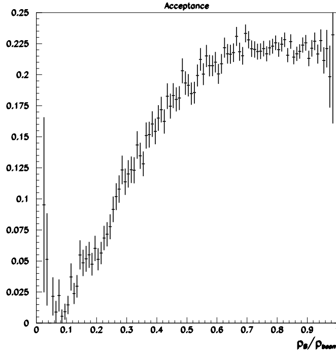
Figure 5.8: Fitted acceptance for signal events versus x_p = p_B/E_{beam} .
