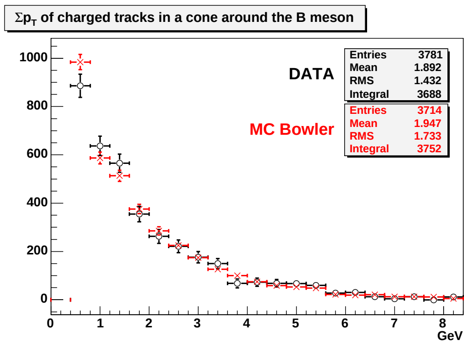
Figure 7.24: The sum of transverse momenta of tracks in a cone of \Delta R < 0.7 around the B meson in the msl=1 PYTHIA sample. Histograms are normalized to the number of B mesons.
