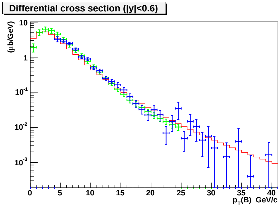
Figure 7.46: The measured differential cross section for |y| < 0.6 (blue histogram with error bars), and the central value of the FONLL theoretical prediction [6] (red solid line). Measurements obtained by CDF [7] using H_b \rightarrow J/\psi X final states have been also displayed (green histogram with error bars).
