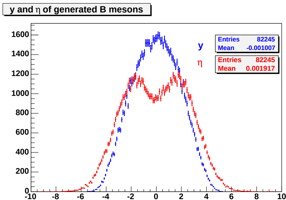
Figure 7.45: Spectra of y (blue) and \eta (red) for B mesons at the generator level of the Monte Carlo sample used for the present analysis. No cuts have been applied.
