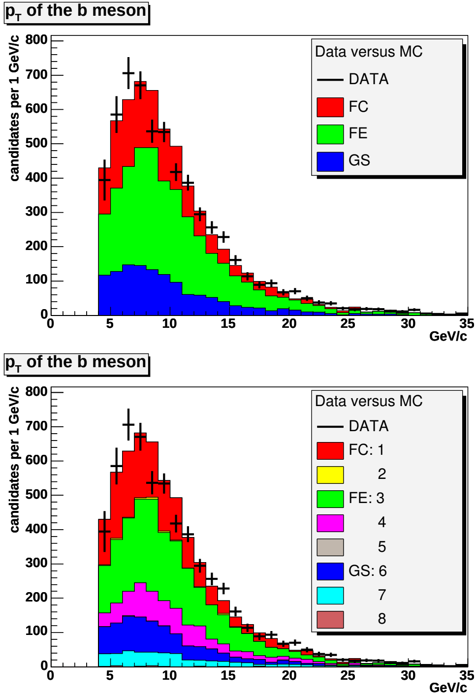
Figure 7.31: Data and Monte Carlo comparison for p_T(B) . The upper plot details the different contributions in the Monte Carlo sample from the FC, FE and GS b quark production mechanisms. The lower plot details the contributions for the classes of processes explained in Section 2.2.2. Histograms are normalized to the number of B mesons.
