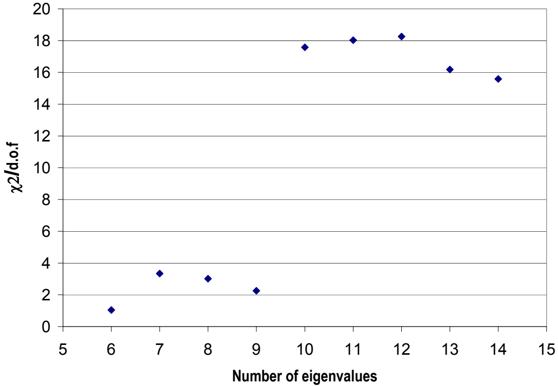
Figure B.1: \chi^2/\text{d.o.f} of the fit as a function of number of eigenvalues for OPAL's fragmentation function.
