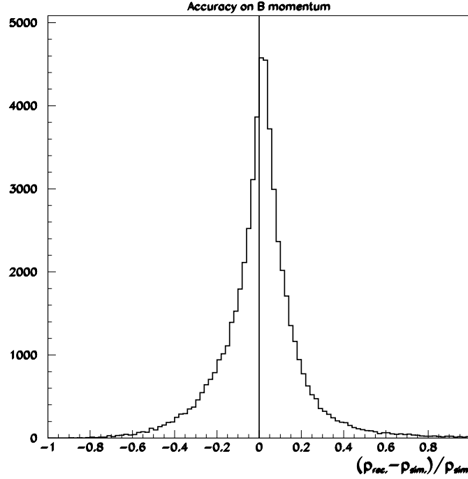
Figure 5.7: (p_{rec} - p_{sim})/p_{sim} for B -hadrons.
