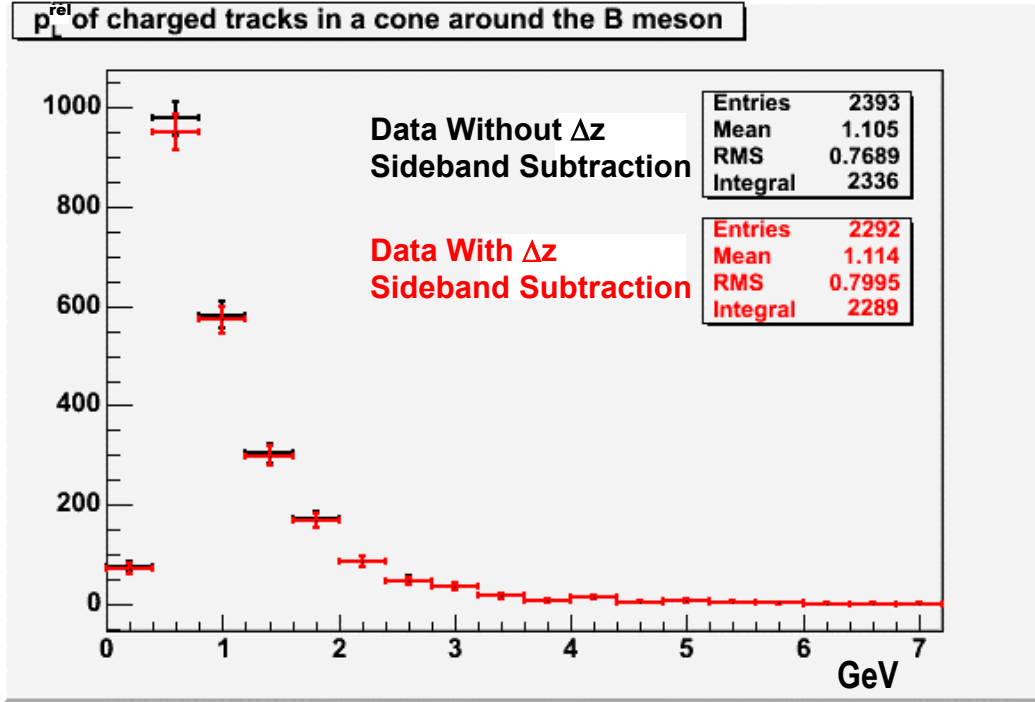
Figure 7.4: The effect of the removal of the pile-up events by subtracting the \Delta z sidebands on p_L^{\text{rel}} , the component of the track momentum parallel to the B meson.
