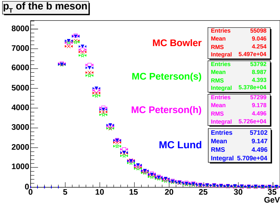
Figure 7.8: The p_T spectrum of the B meson in four Monte Carlo samples, generated with different fragmentation functions. The Lund model is not shown in corresponding plots for tracks.
