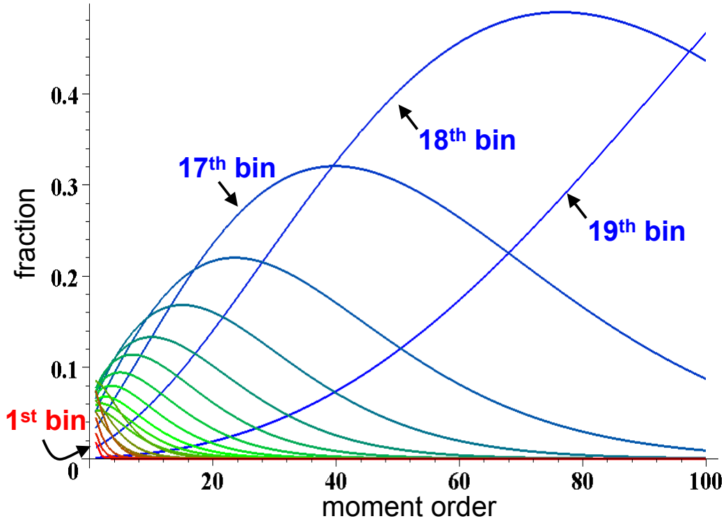
Figure 6.17: The fraction of the moment of N 'th order contributed by the each bin of the measured fragmentation function. This illustration is based on the result from ALEPH [31]. The red curves on the small N side of the figure correspond to the smallest x bins, and the blue curves that mainly contribute to moments of large order N correspond the largest x bins.
