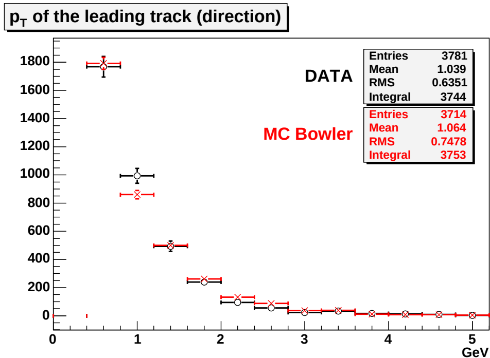
Figure 7.22: The transverse momentum p_T for the leading directional track in a cone of \Delta R < 0.7 around the B meson in the m_{\text{sel}}=1 PYTHIA sample. Histograms are normalized to the number of B mesons.
