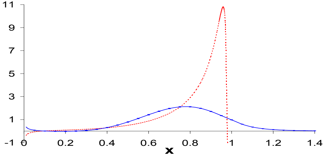
Figure 6.19: x -dependence of the perturbative (red dotted line) and non-perturbative (full blue line) QCD components of the measured charm quark fragmentation distribution. These curves are obtained by interpolating corresponding values determined at a large number of points in the x -variable. The perturbative QCD component is given by the analytic computation of [14].
