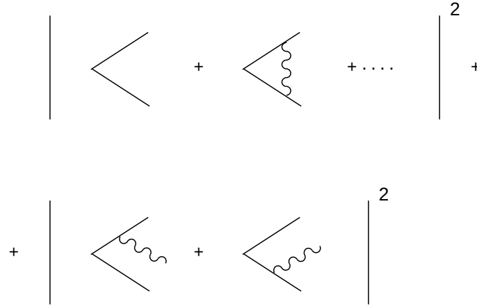
Figure 2.4: Cancellation of real gluon radiation and virtual gluon exchange.
