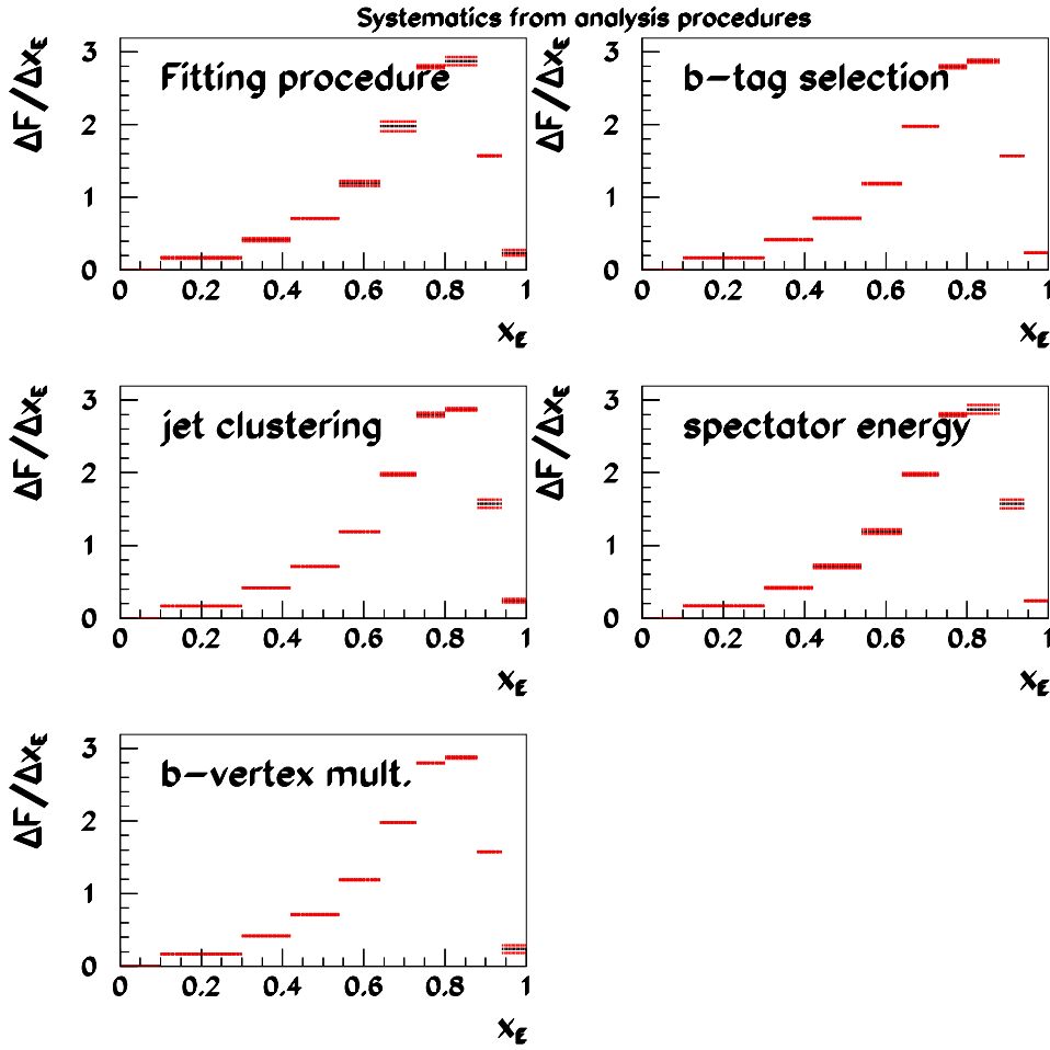
Figure 5.18: Systematic uncertainties related to the stability of results versus the values of criteria used in the analysis.
