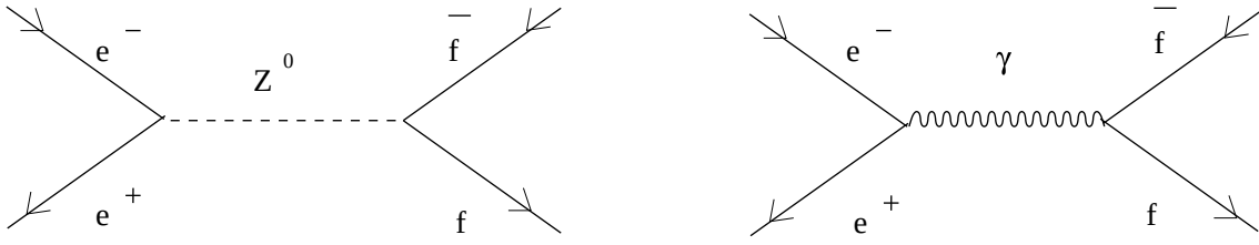
Figure 2.2: Fermion pair production at LEP.
