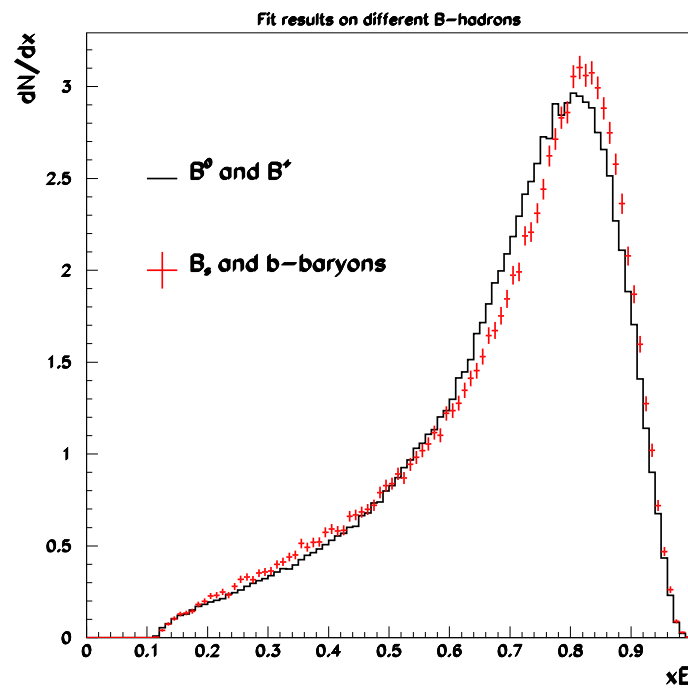
Figure 5.20: Comparison between expected x_E distributions for B_d^0 and B^+ mesons and for B_s^0 and b-baryons.
