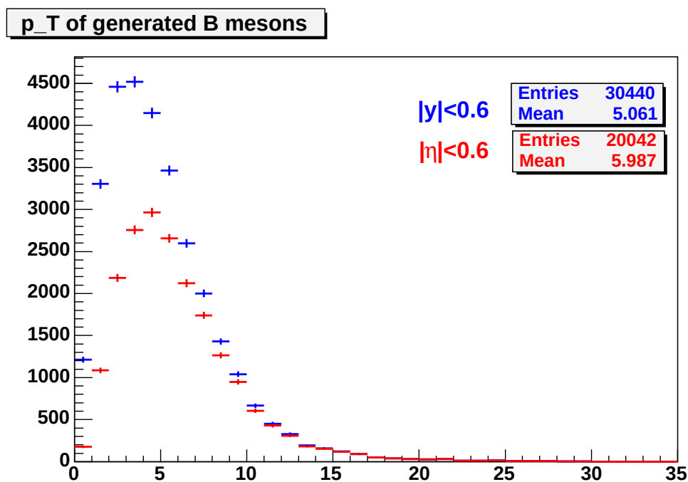
Figure 7.44: p_T spectrum of B mesons that passed the |y| < 0.6 cut (blue) and the |\eta| < 0.6 cut (red), at the generator level of the Monte Carlo sample used for the present analysis.
