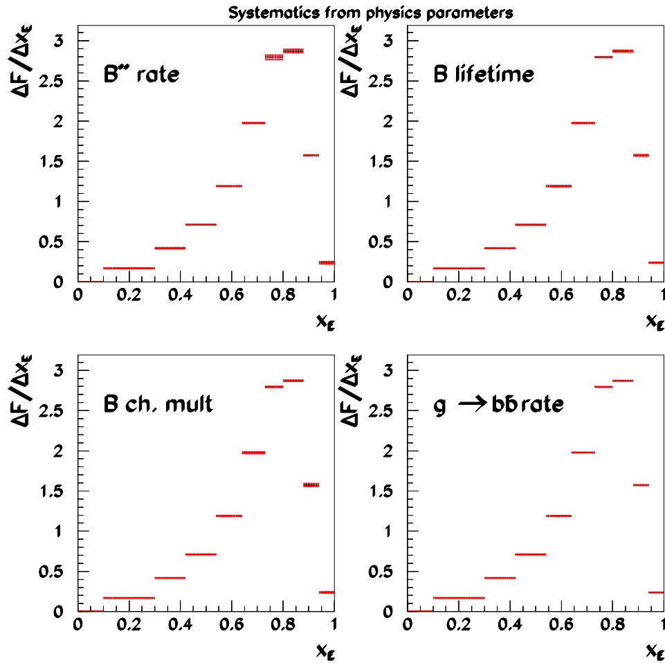
Figure 5.17: Systematic uncertainties originating from uncertainties on physics parameters governing B -hadron decay and production characteristics.
