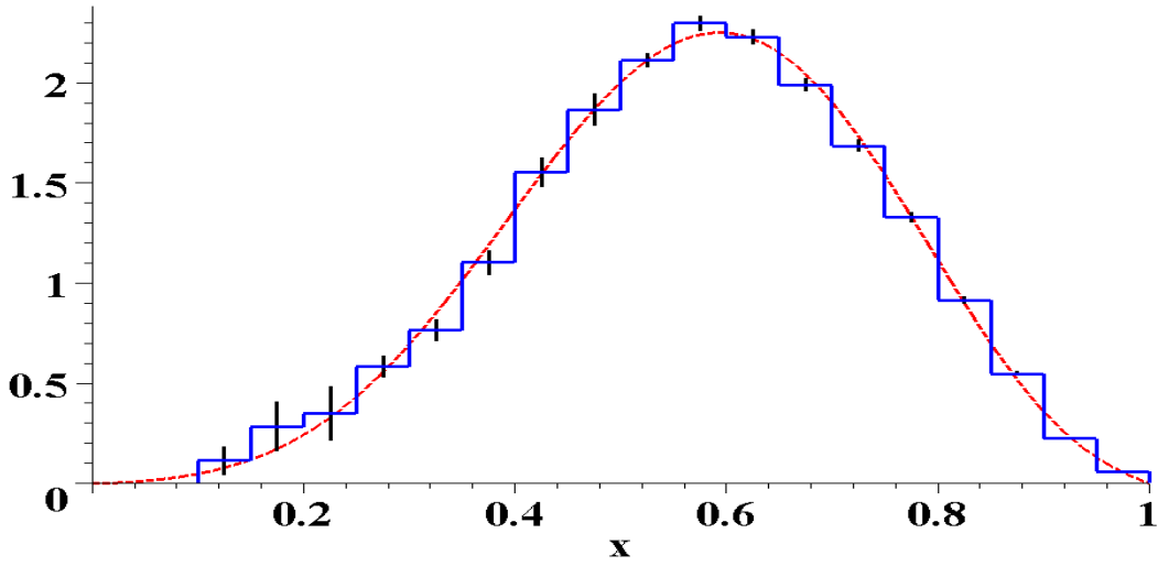
Figure 6.18: Normalized spectrum of the scaled momentum, x_p of D^0 mesons in electron-positron annihilation as measured by CLEO [86]. The dashed curve is the parametrization of Equation (6.6), fit to the histogram.
