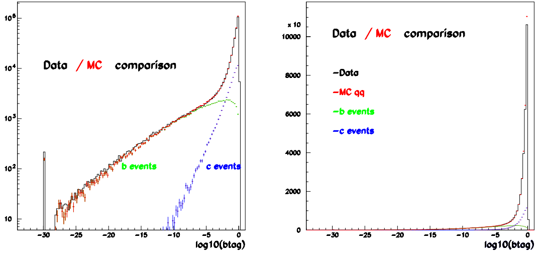
Figure 5.1: Distribution of -\log_{10}(P_{btag}) in log- (left) and lin- (right) scale.
