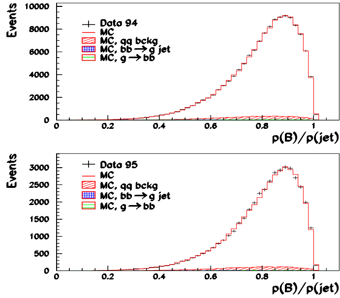
Figure 5.10: Fitted x_p^{rec} = p_B^{rec} / p_{jet} distributions on selected events. Top: 1994 sample. Bottom: 1995 sample.
