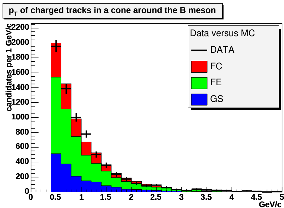
Figure 7.32: Data and Monte Carlo comparison for p_T of tracks in a cone around the B meson. Contributions in the Monte Carlo sample from the FC, FE and GS b quark production mechanisms are detailed. Histograms are normalized to the number of B mesons.
