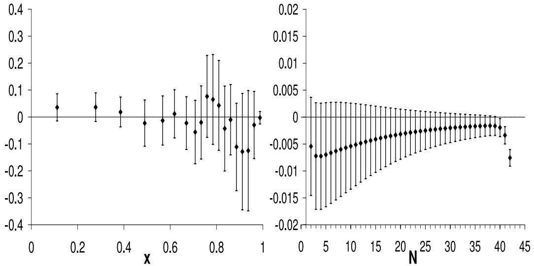
Figure 6.9: Comparison between the fitted and measured b -quark fragmentation distributions. Left: Differences between the fitted and the measured distributions in each x -bin are shown and the total error bars, relative to the measurements, are displayed. The fitted results correspond to the averaged values obtained from Equation (6.1) over the bin. Right: Differences between the fitted and measured moments of the b -fragmentation distribution. Fitted moments result from the product given in Equation (6.4) in which \tilde{\mathcal{D}}_{\text{non-pert.}}(N) are the moments of the fitted non-perturbative QCD distribution corresponding to Equation (6.8) and \tilde{\mathcal{D}}_{\text{pert.}}(N) corresponds to the analytic computation [14].
