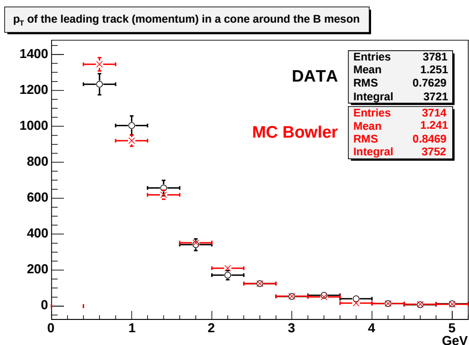
Figure 7.23: The transverse momentum p_T for the leading momentum track in a cone of \Delta R < 0.7 around the B meson in the msl=1 PYTHIA sample. Histograms are normalized to the number of B mesons.
