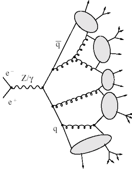
Figure 2.7: A scheme of the cluster hadronization model.
