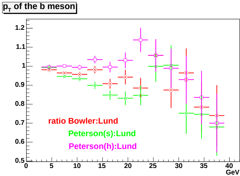
Figure 7.13: Variation of the B production cross section, expected when considering different fragmentation models. Ratios of the production rate expected in bins of the p_T distribution, are presented for Bowler, soft Peterson and hard Peterson fragmentation functions, with respect to the prediction obtained with the Lund fragmentation function.
