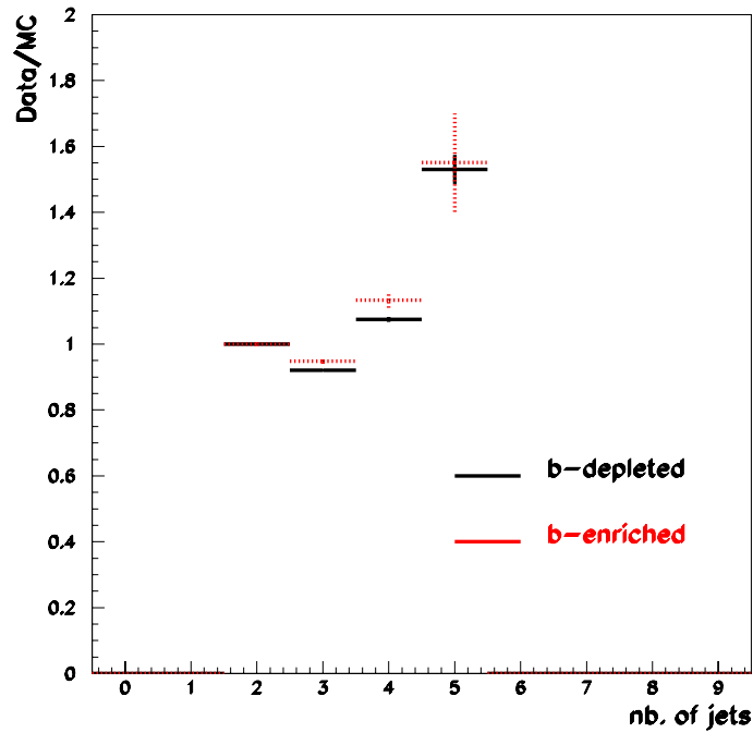
Figure 5.15: Ratio between number of events having a given jet multiplicity in data and in the simulation. For 2-jet events this ratio has been set to unity. Events depleted and enriched in b hadrons have been compared.
