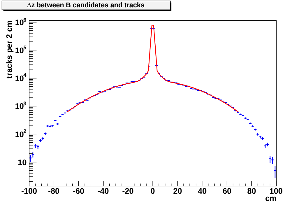
Figure 7.3: The distribution of \Delta z \equiv Z(B^+) - Z_0(\text{track}) where Z(B^+) is the Z coordinate of the B^+ meson's decay point, and Z_0(\text{track}) is the Z coordinate of the point of the closest approach. The \Delta z consists of two narrow Gaussians to describe the signal and a broad Gaussian to describe the contribution of tracks from Pile-Up events.
