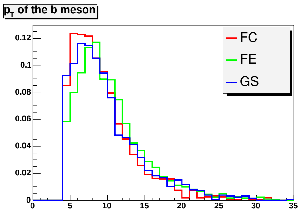
Figure 7.35: Contributions in the Monte Carlo sample from the FC, FE and GS to the p_T distribution of the B meson. Histograms are normalized to unity. Shapes of the distributions differ between the mechanisms.
