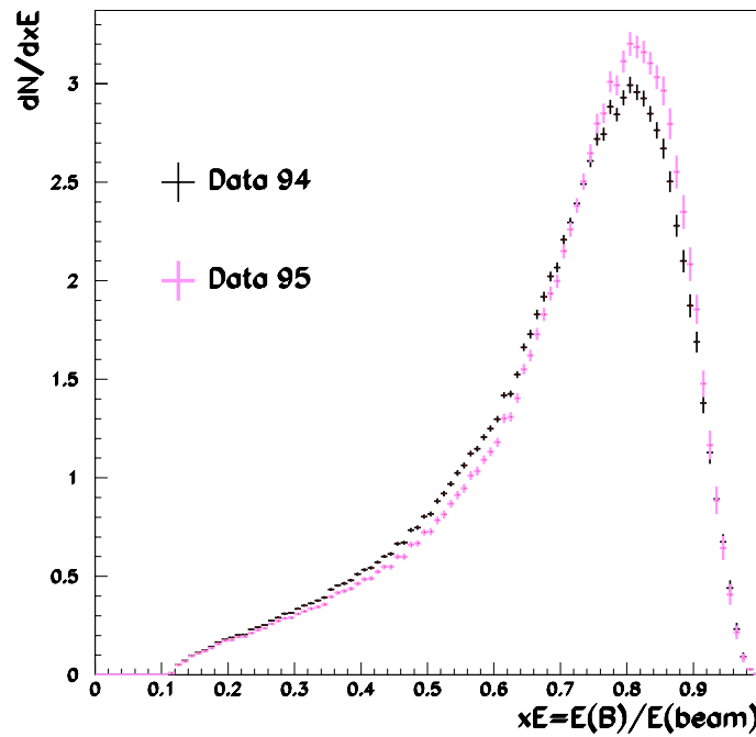
Figure 5.12: Comparison between x_E distributions obtained using the 1994 and 1995 events samples.
