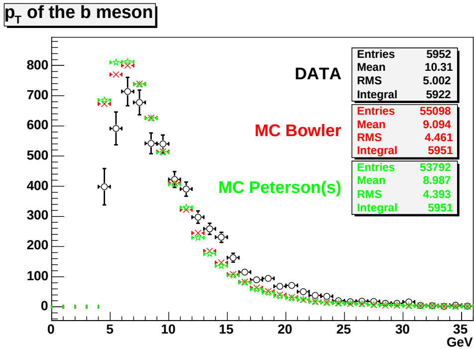
Figure 7.14: The p_T spectrum of the B . Comparison between the data and two Monte Carlo msel=5 samples with the Bowler and Peterson fragmentation functions. Histograms are normalized to the number of B mesons.
