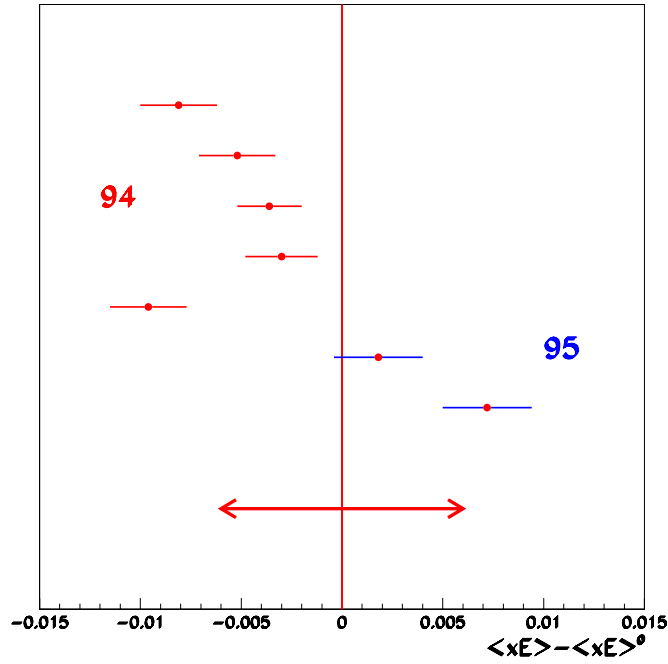
Figure 5.14: Differences between the fitted x_E values, relative to the average, for different data samples.
