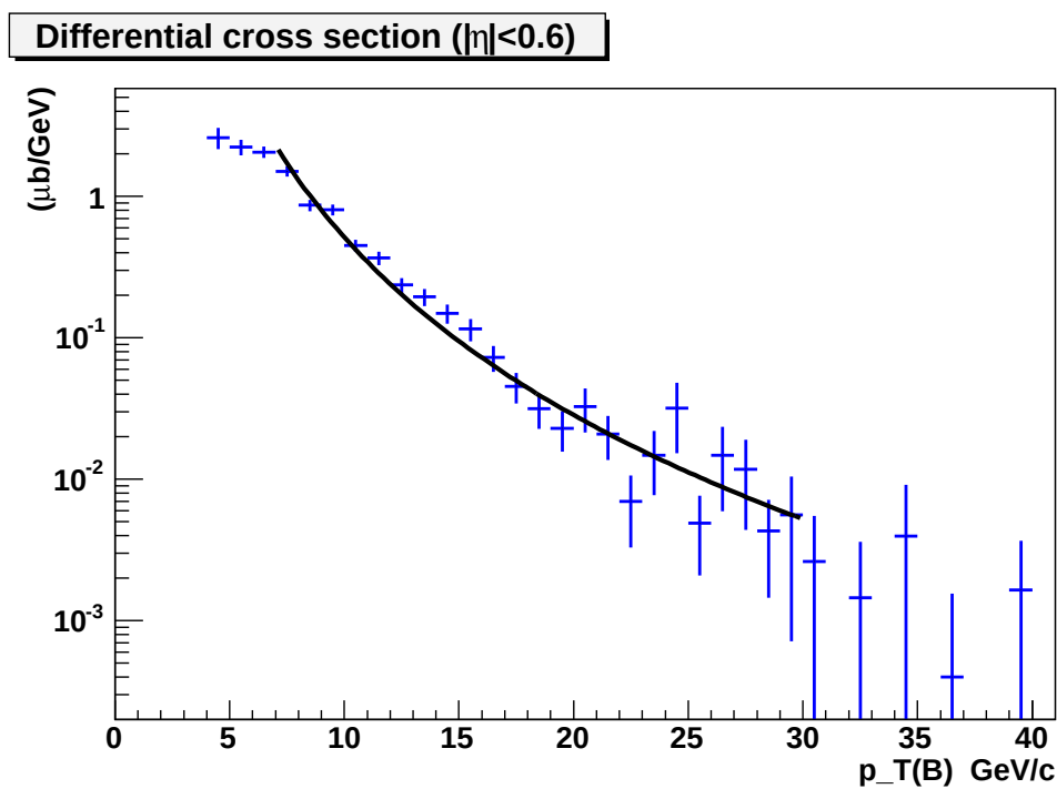
Figure 7.40: The differential cross section for |\eta| < 0.6 .
