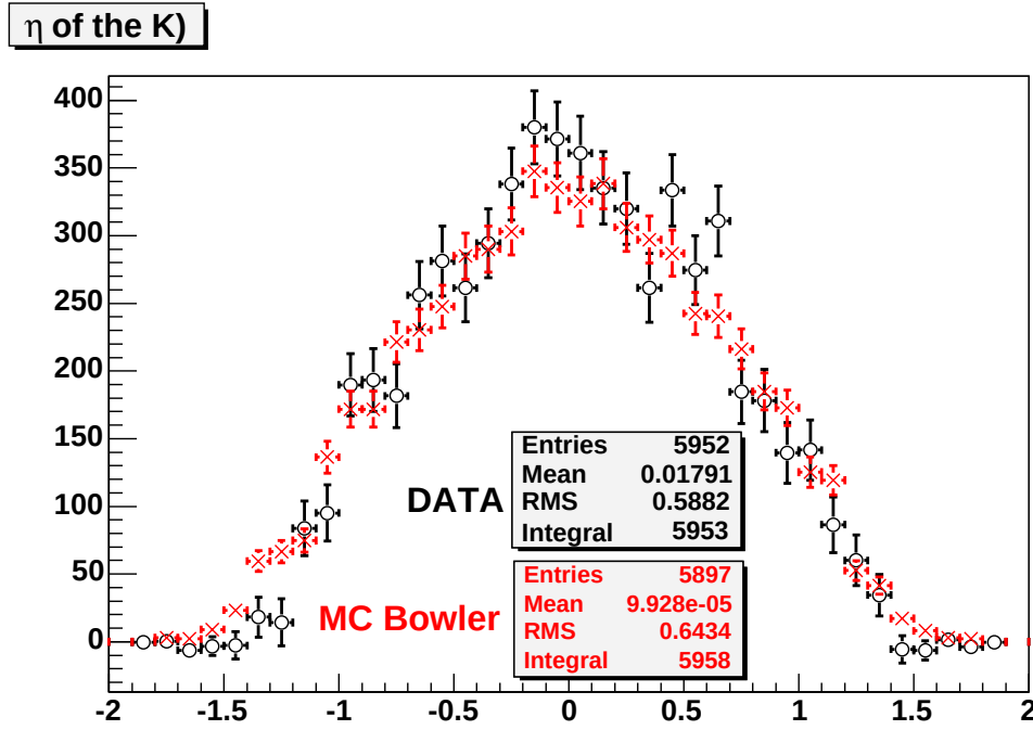
Figure 7.43: \eta distributions of the kaon candidates, in data and in the Monte Carlo sample, used to calculate the efficiency. Histograms are normalized to the number of B mesons.
