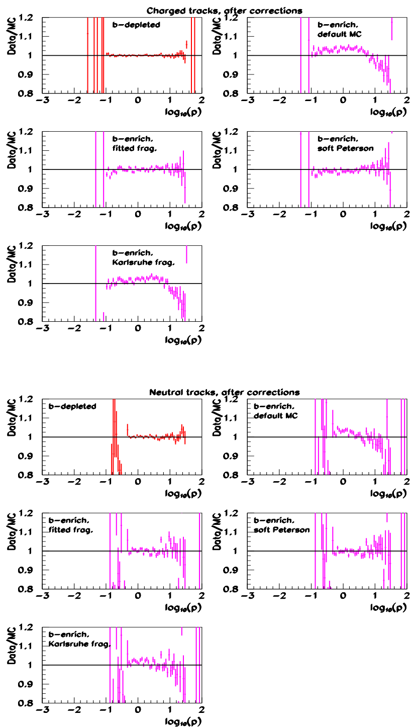
Figure 5.3: Ratio Data/MC for charged (top) and neutral (bottom) track momentum distributions ( \log_{10} p ) after having applied corrections.
