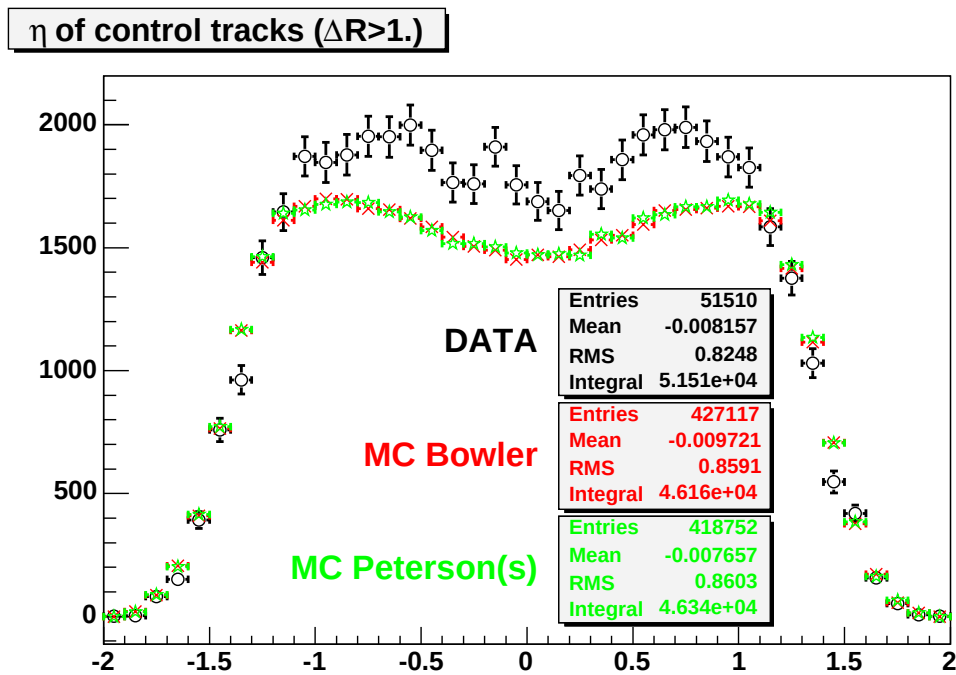
Figure 7.16: The \eta spectrum of tracks in a cone with \Delta R > 1 (control tracks). Comparison between the data and two Monte Carlo ( m_{\text{sel}}=5 ) samples with the Bowler and Peterson fragmentation functions. Histograms are normalized to the number of B mesons.
