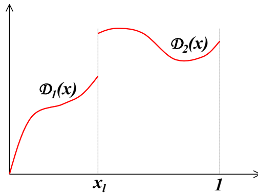
Figure A.2: Piecewise defined function for 0 < x < 1 . In each interval the function is taken as a polynomial of order J .
