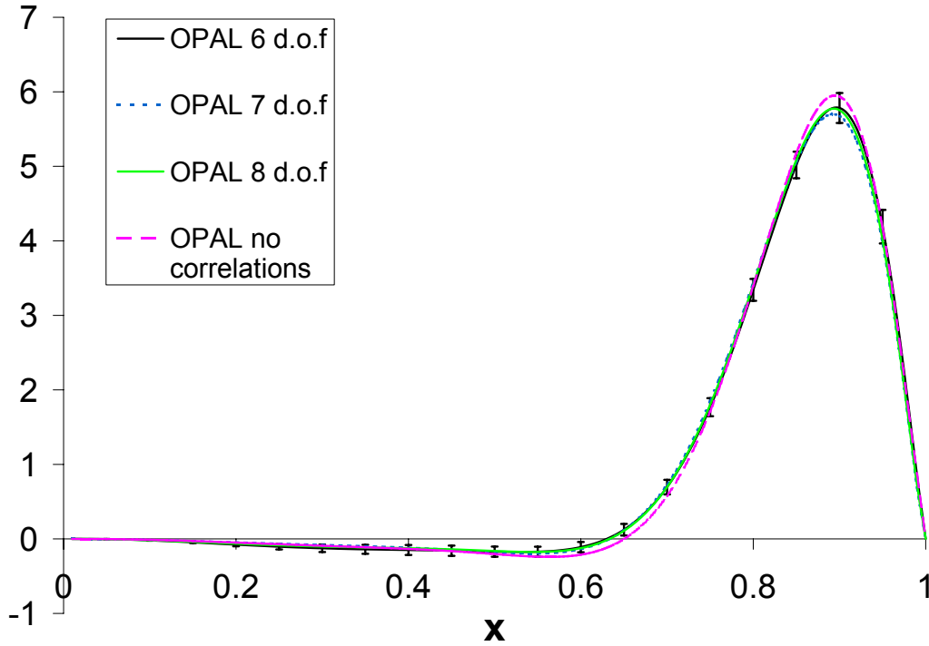
Figure 6.12: The non-perturbative component of the fragmentation function from OPAL [32], obtained with a different number of eigenvalues in the fit of a parametrization to the measured function. The result for the case where correlations between bins have been completely neglected is also presented.
