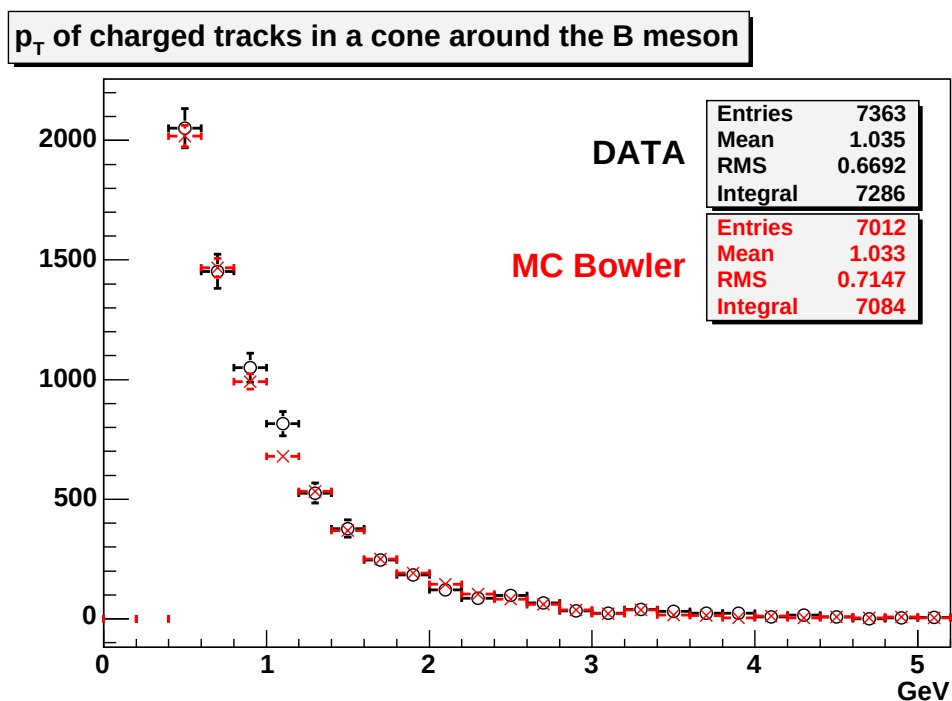
Figure 7.19: The transverse momentum p_T of all tracks within a cone of \Delta R < 0.7 around the B meson in the msl=1 PYTHIA sample. Histograms are normalized to the number of B mesons.
