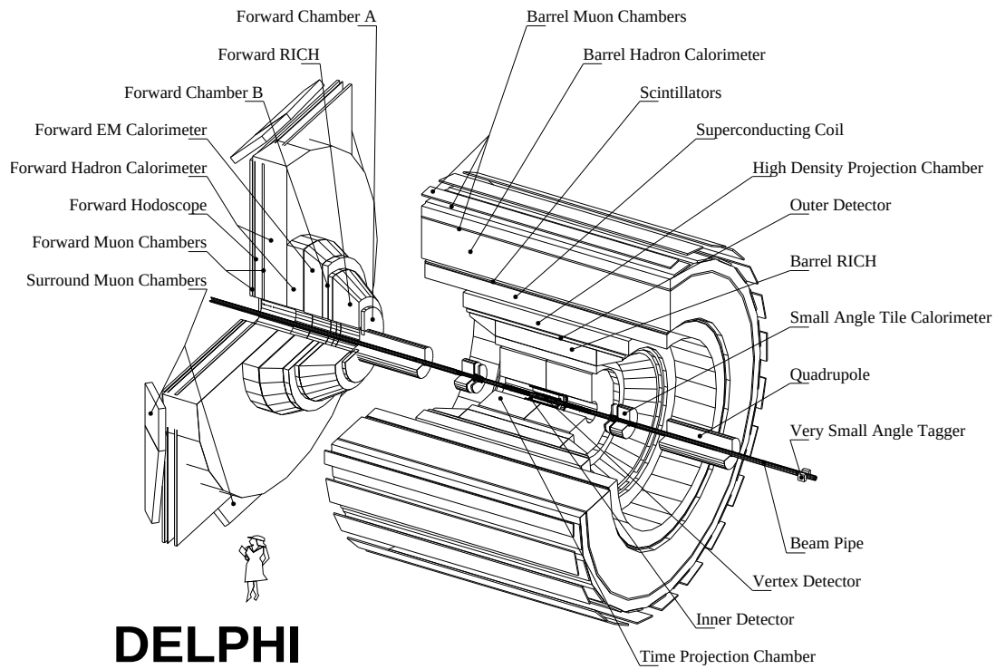
Figure 3.3: Schematic layout of the DELPHI detector.
