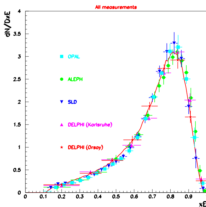
Figure 5.19: Comparison between the measured x_E distribution and corresponding results obtained by ALEPH, DELPHI, OPAL and SLD.
