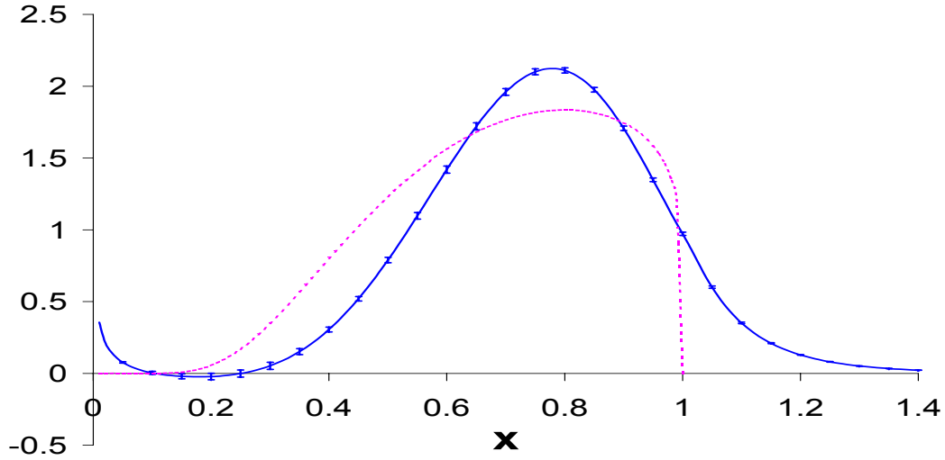
Figure 6.20: x -dependence of the non-perturbative QCD components of the measured charm quark fragmentation distribution. The solid blue curve has been obtained by the extraction procedure, using the perturbative QCD component given by the analytic computation of [14]. The red dotted curve described the Lund Fragmentation function, with the parameters fitted in [86] to reproduce the D^0 spectrum: a = 0.178 and b = 0.393 . The transverse mass in the Lund model was assumed here to be the mass of the D^0 meson.
