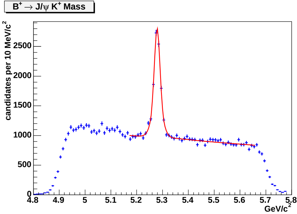
Figure 7.1: The invariant mass of B^\pm \rightarrow J/\psi K^\pm , with the fit overlaid. The signal consists of the two signal Gaussians for B^\pm \rightarrow J/\psi K^\pm , and another one for the Cabibbo-suppressed decay mode B^\pm \rightarrow J/\psi \pi^\pm , which is fixed to 4% of J/\psi K^\pm . The combinatorial background is modeled as a linear function.
