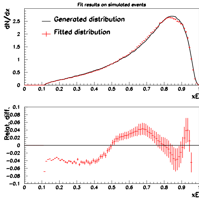
Figure 5.13: Comparison between generated and fitted x_E distributions. Top: The generated (full line) and fitted (points with error bars) distributions are compared. Bottom: The relative difference between the fitted and simulated distributions is given.
