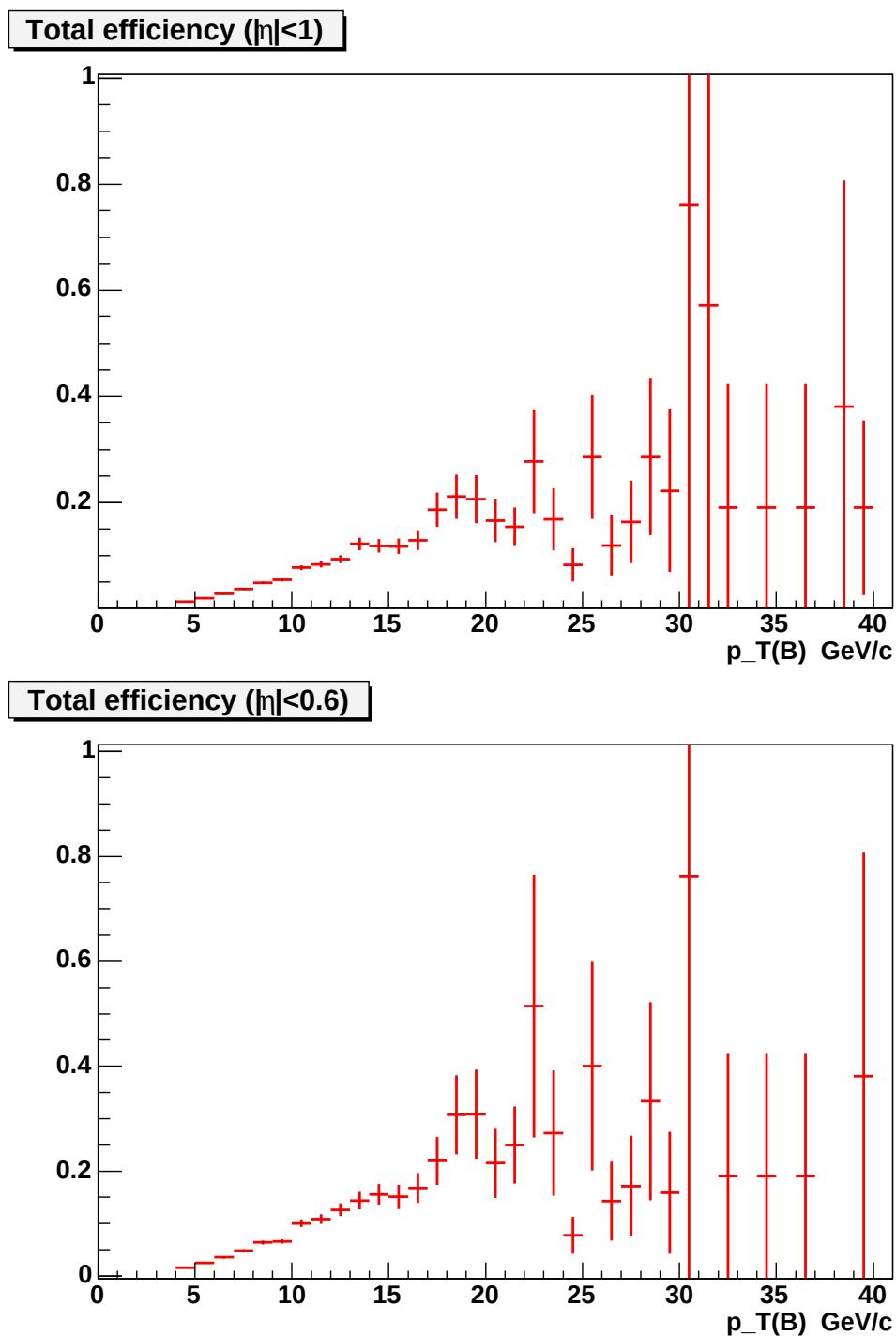
Figure 7.38: Total efficiency of detection and analysis effects for the B^\pm mesons, in two regions of pseudo-rapidity: |\eta| < 1 (top) and |\eta| < 0.6 (bottom)
