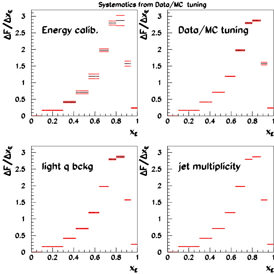
Figure 5.16: Systematic uncertainties originating from uncertainties in the tuning of the simulation.
