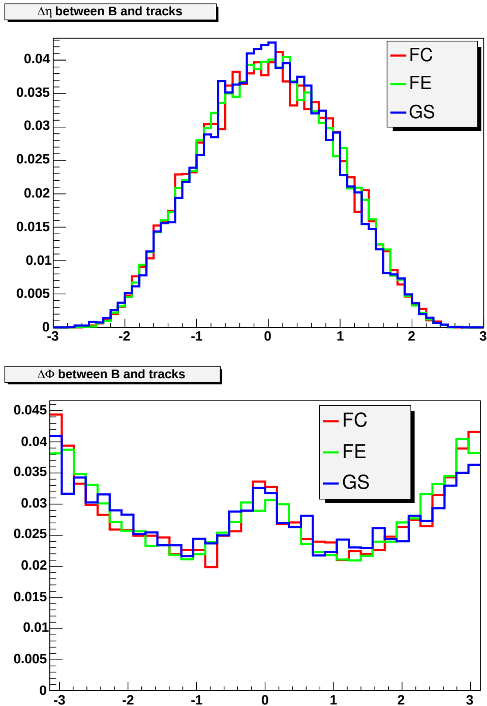
Figure 7.37: Contributions in the Monte Carlo sample from the FC, FE and GS to the \Delta\eta (top) and \Delta\Phi (bottom) distribution of all tracks in the event. Histograms are normalized to unity. Shapes of the distributions from the different mechanisms are similar.
