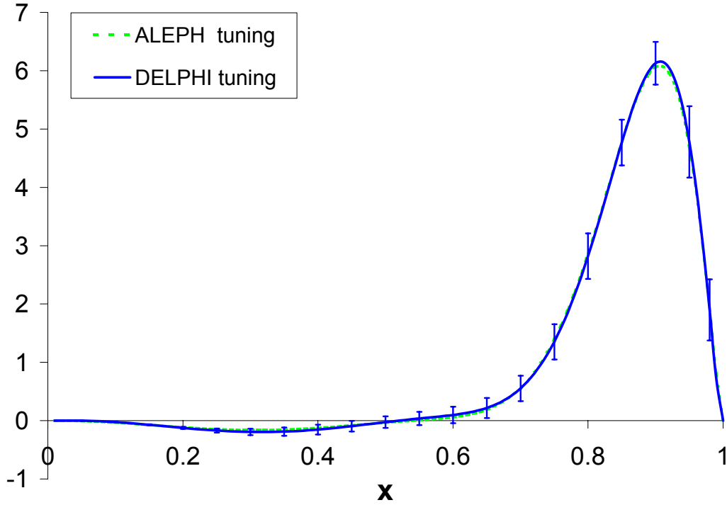
Figure 6.13: The non-perturbative component for jetset with aleph tuning.
