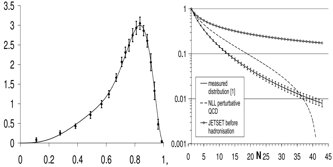
Figure 6.1: Left: Comparison between the measured (points with error bars) b -fragmentation distribution and the fitted parametrization using Equation (6.6). Right: Moments of the measured (full line) x distribution, of the perturbative QCD component [14](dashed line) and of the generated distribution obtained in JETSET before hadronization (full line with circles). Data from [31] have been used.
