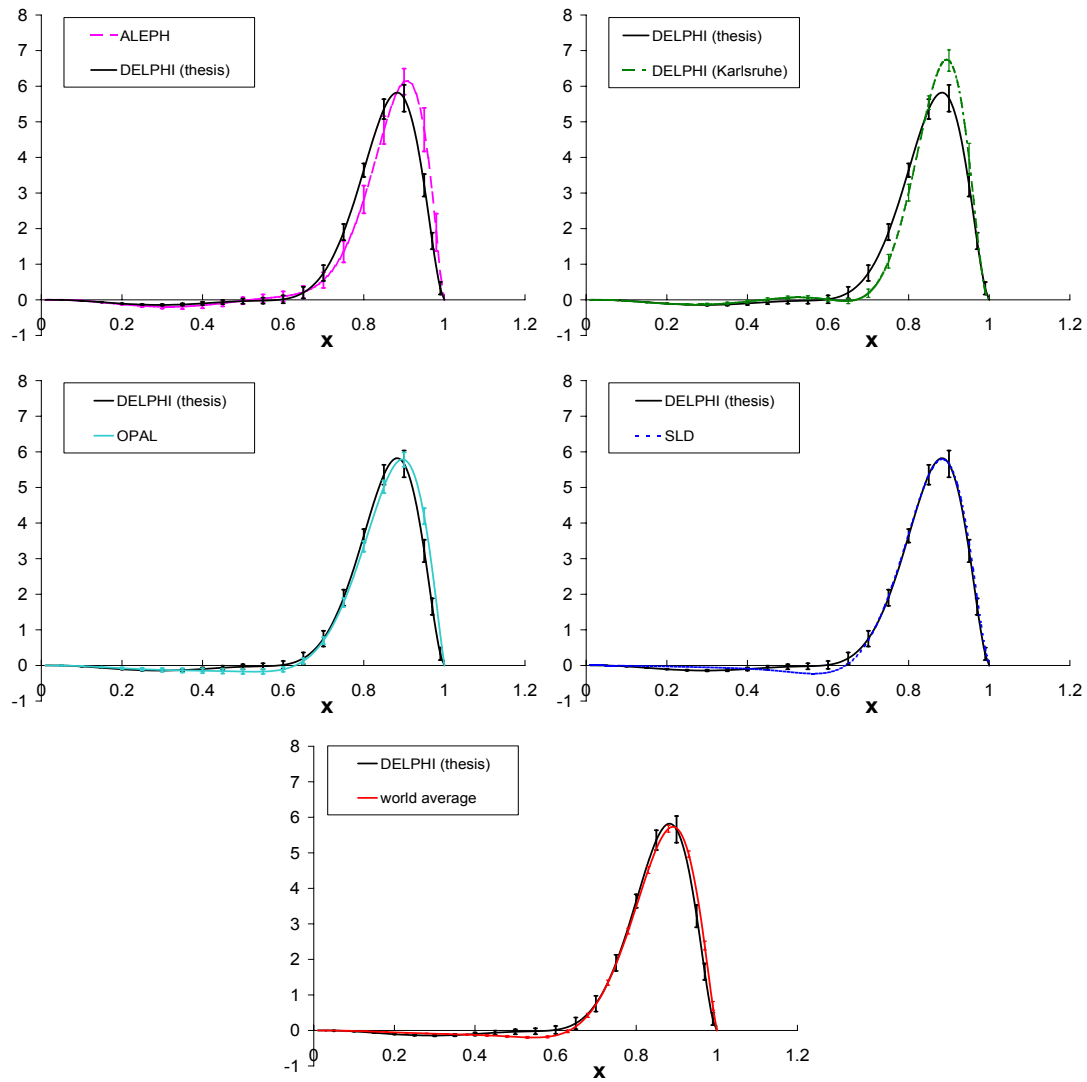
Figure 6.15: The extracted non-perturbative QCD component of the b quark fragmentation function from the present thesis work, compared separately to the results from ALEPH [31], DELPHI- Karlsruhe [34], OPAL [32] SLD [33] and the combined fragmentation distribution. The perturbative QCD component has been taken from JETSET 7.3.
