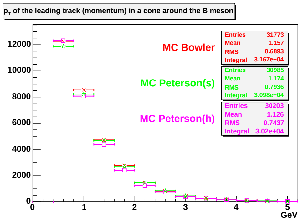
Figure 7.11: The p_T spectrum of the highest p_T track in a cone around the B meson in three Monte Carlo samples, generated with different fragmentation functions.
