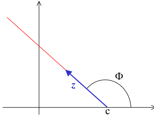
Figure A.1: Integration contour for the inverse Mellin transformation.
