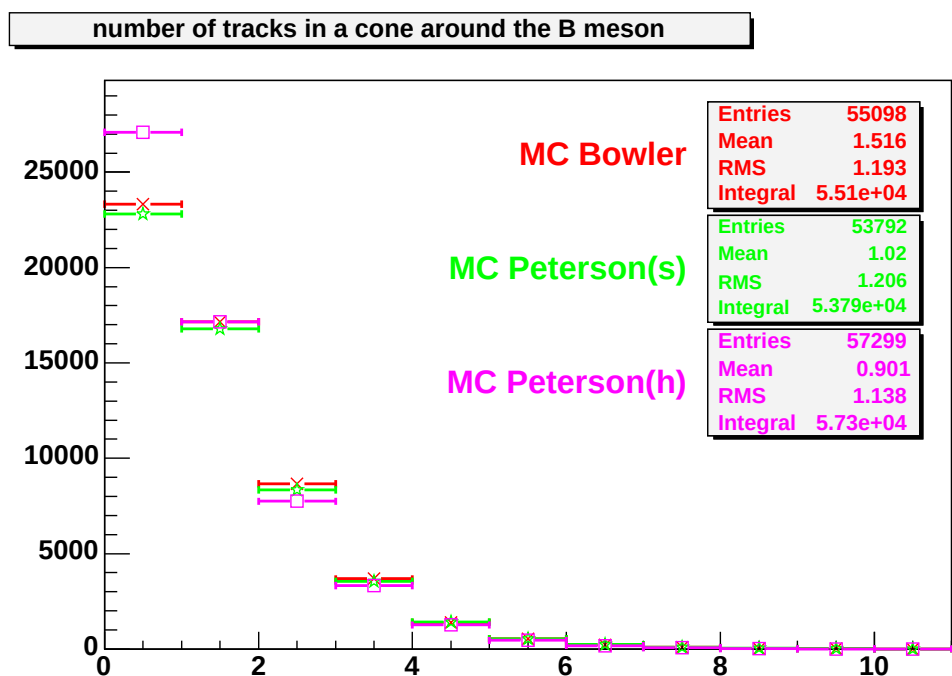
Figure 7.12: The multiplicity of tracks in a cone of opening \Delta R = 0.7 around the B meson, in three Monte Carlo samples, generated with different fragmentation functions.
