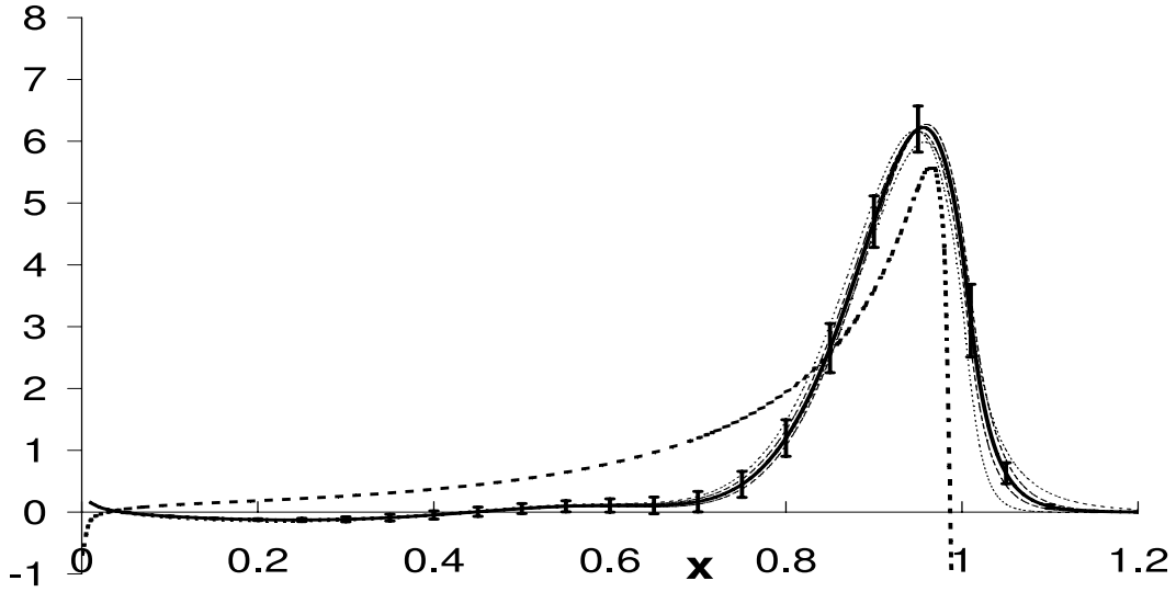
Figure 6.5: x -dependence of the perturbative (dotted line) and non-perturbative (full line) QCD components of the measured b -fragmentation distribution. These curves are obtained by interpolating corresponding values determined at a large number of points in the x -variable. The perturbative QCD component is given by the analytic computation of [14]. The thin lines on both sides of the non-perturbative distribution correspond to \mu_0 = \mu_{0F} = \{m_b/2, 2m_b\} (dotted lines) and \Lambda_{\text{QCD}}^{(5)} = (0.226 \pm 0.025) GeV (dashed lines). Variations induced by the other parameters, \mu = \mu_F = \{Q/2, 2Q\} and m_b = (4.75 \pm 0.25) GeV/c 2 are smaller. In addition, quoted error bars correspond to measurement uncertainties and are correlated for different x -values. The perturbative QCD dotted curve has to be complemented by a \delta -function containing 5% of the events, located at x = 1 .
