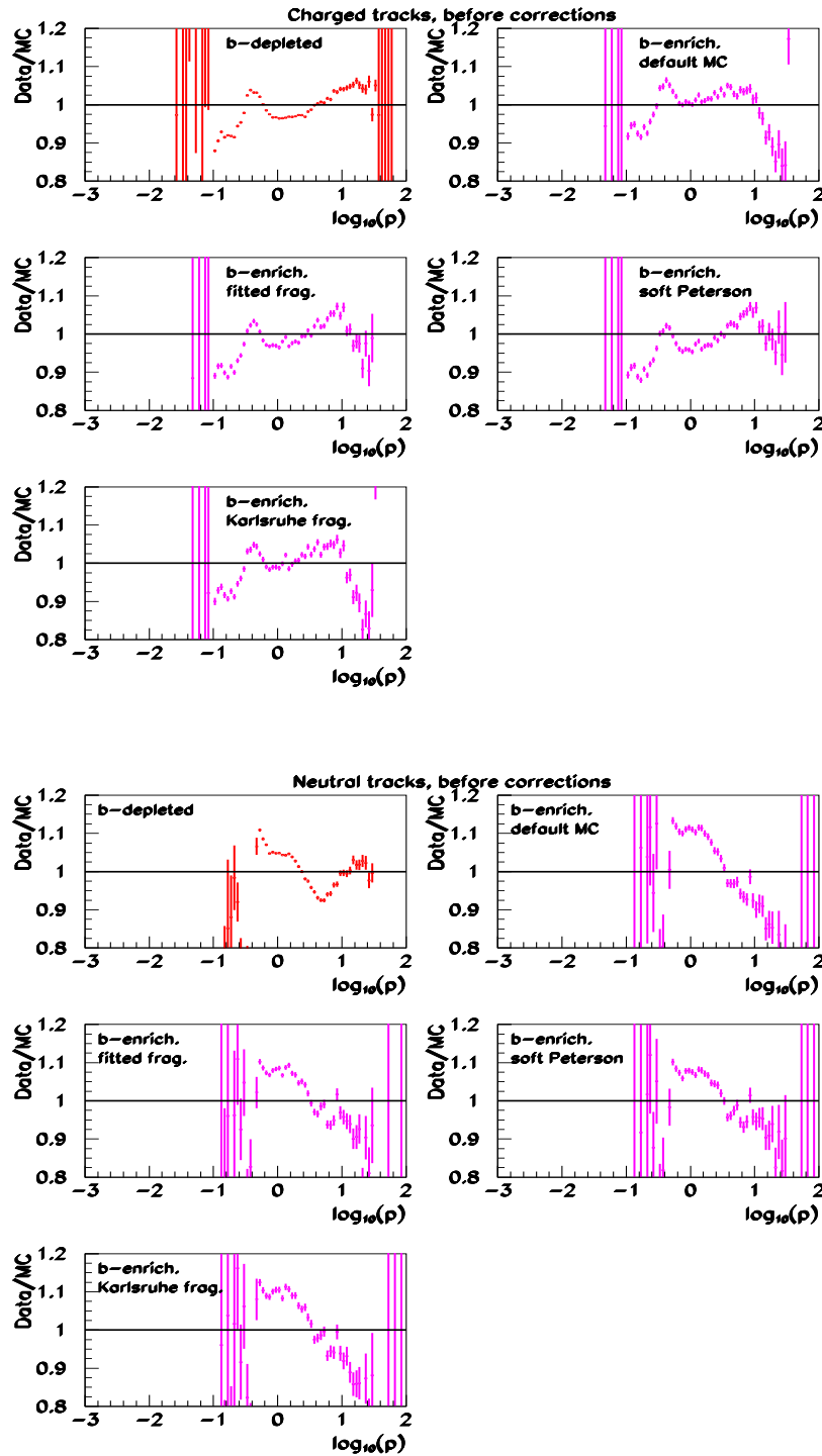
Figure 5.2: Ratio Data/MC for charged (top) and neutral (bottom) track momentum distributions ( \log_{10} p ). Plots in upper left corners correspond to b -depleted samples. The others are obtained using b -enriched samples and different models for the b -fragmentation distribution.
