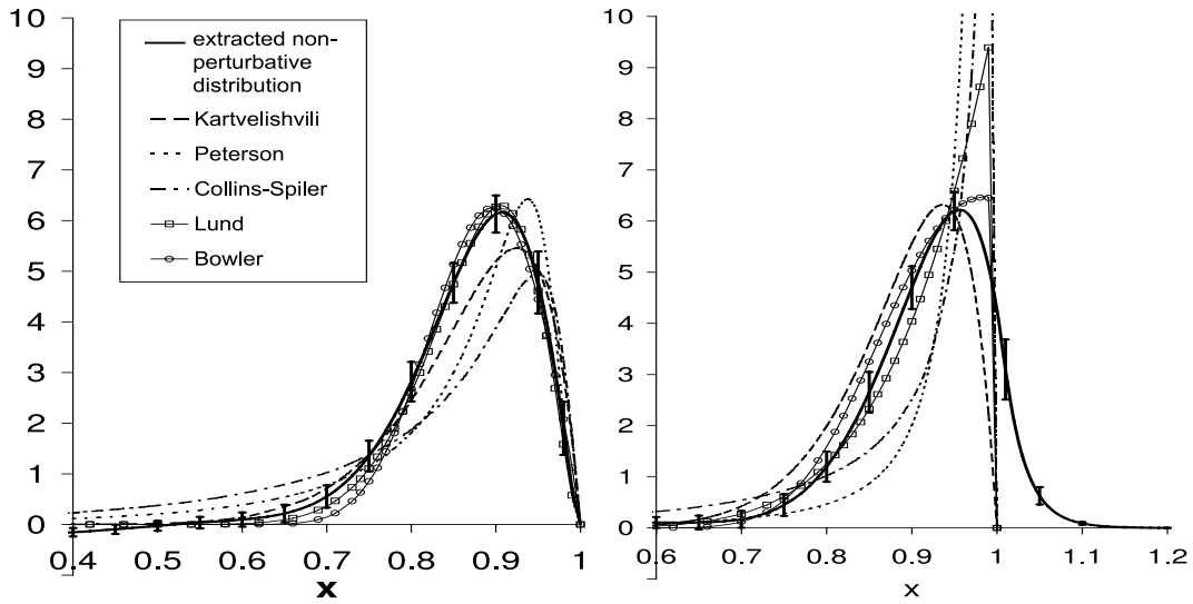
Figure 6.7: Comparison between the directly extracted non-perturbative component (thick full line) and the model fits on data taken from [31]. Left: the perturbative QCD component is taken from JETSET. Right: the theoretical perturbative QCD component[14] is used.
