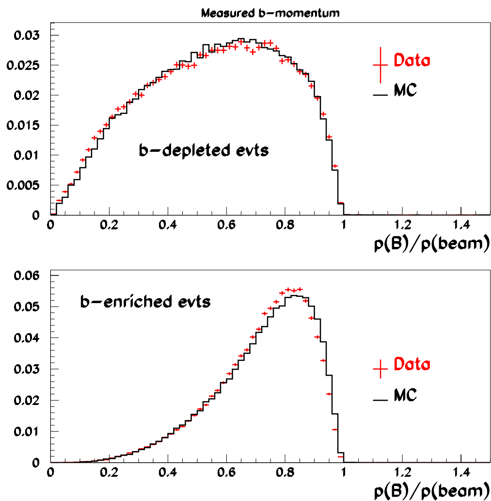
Figure 5.9: Comparison between the measured x_p^{\text{rec}} distributions obtained in data (points with error bars) and in the MC q\bar{q} simulation (histogram). Top: depleted b-sample; Bottom: enriched b-sample.
