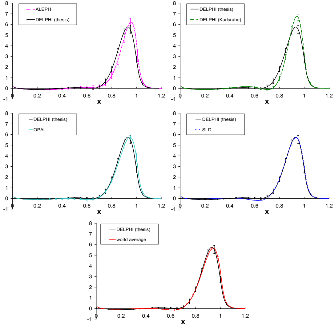
Figure 6.16: The extracted non-perturbative QCD component of the b quark fragmentation function from the present thesis work, compared separately to the results from ALEPH [31], DELPHI- Karlsruhe [34], OPAL [32] SLD [33] and the combined fragmentation distribution. The perturbative QCD component has been taken from NLL QCD [14].
