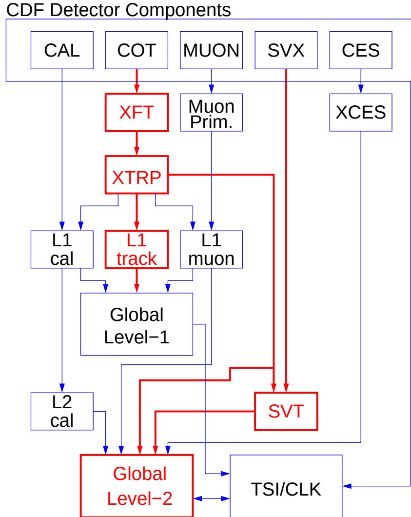
Figure 4.11: Diagram of the different trigger paths at Level 1 and 2. The data flow for the track trigger paths is outlined in red.
