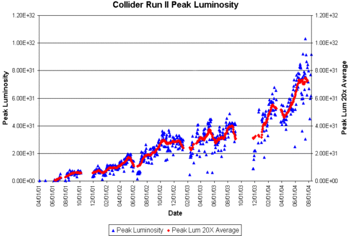
Figure 4.2: Peak luminosities for stores collided between April 2001 and August 2004.
