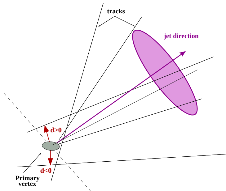
Figure 3.10: Impact parameter sign definition.
