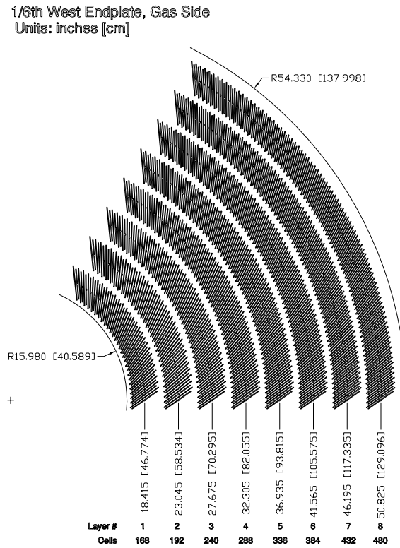
Figure 4.6: Layout of wire planes on a COT endplate.
