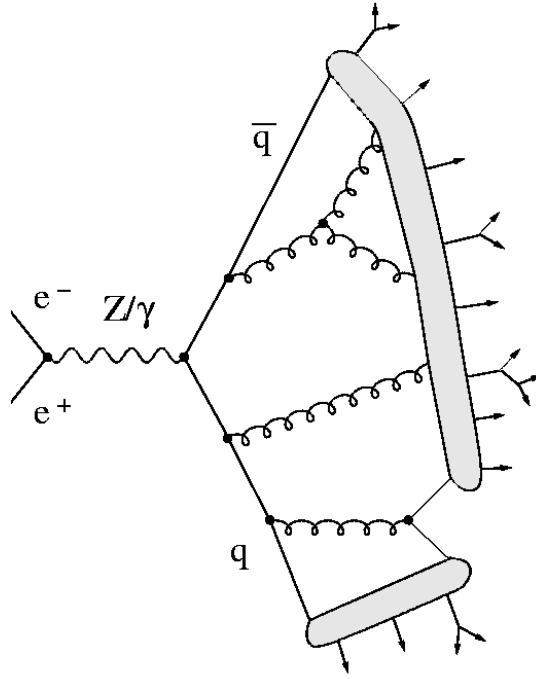
Figure 2.8: A scheme of the string hadronization model.
