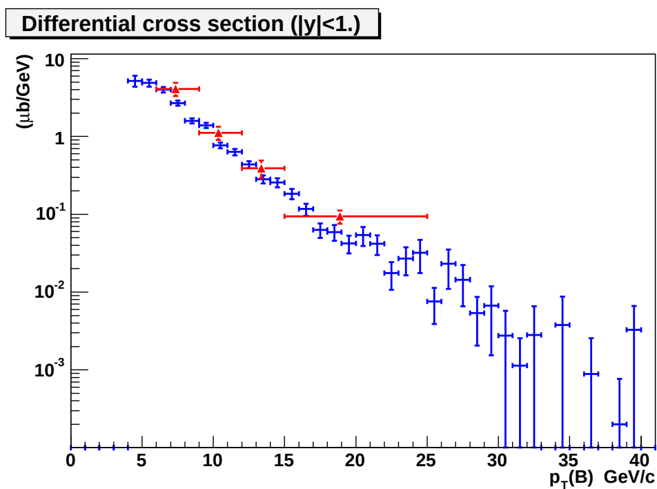
Figure 7.47: The measured differential cross section for |y| < 1 , obtained in the present thesis (blue histogram), compared to the similar measurement from CDF RunI [94] (red histogram).
