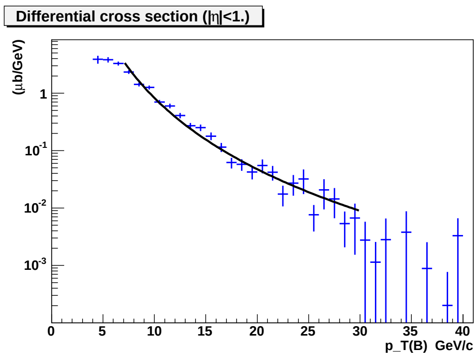
Figure 7.39: The differential cross section for |\eta| < 1 .
