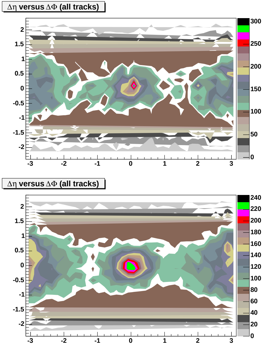
Figure 7.30: The track activity in the \Delta\eta - \Delta\phi plane around the B meson in data (top) and the Monte Carlo msel=1 sample (bottom). The activity in the vicinity of the opposite side B meson is also visible.
