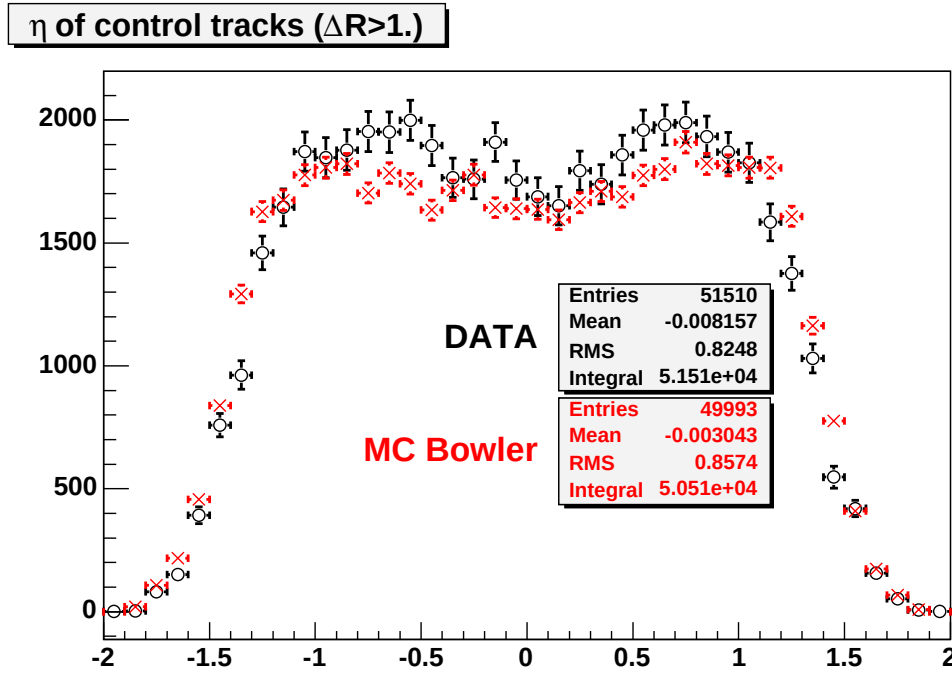
Figure 7.29: Plot of the pseudo-rapidity variable \eta for the control tracks in the msl=1 PYTHIA sample. Histograms are normalized to the number of B mesons.
