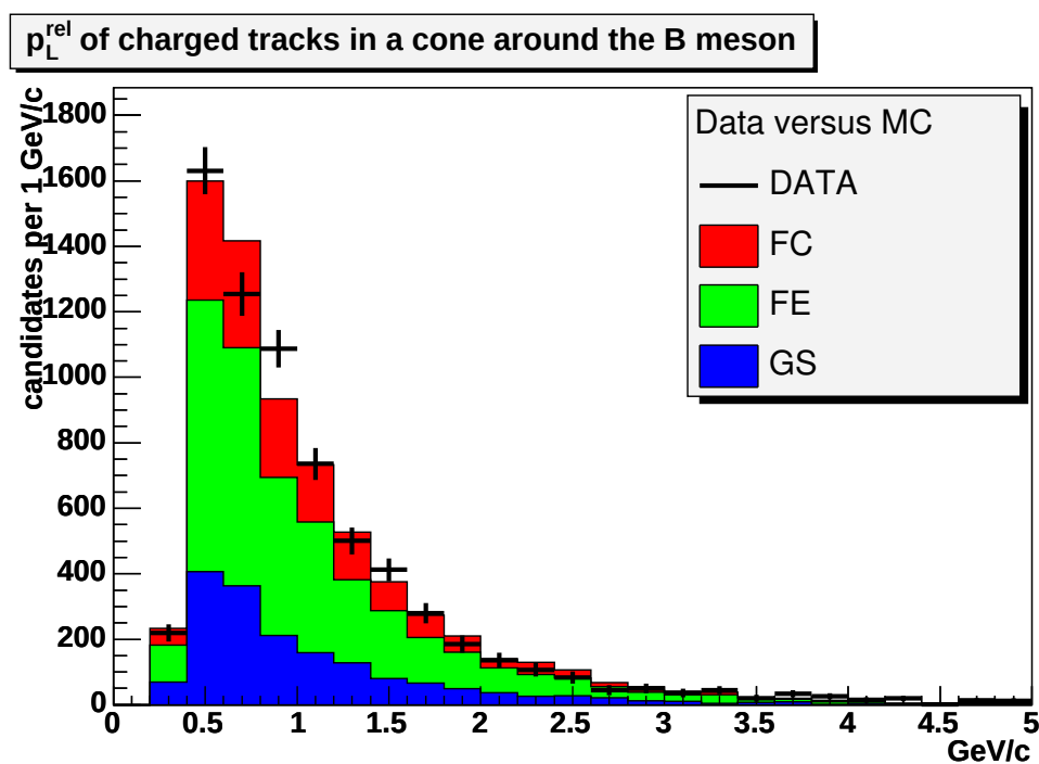
Figure 7.33: Data and Monte Carlo comparison for p_L^{\text{rel}} of tracks in a cone around the B meson. Contributions in the Monte Carlo sample from the FC, FE and GS b quark production mechanisms are detailed. Histograms are normalized to the number of B mesons.
