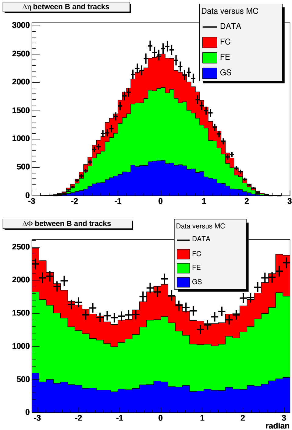
Figure 7.34: Data and Monte Carlo comparisons for the angular distributions of all the tracks in the event with respect to the B meson direction. The upper plot shows the distribution for \Delta\eta , and the lower for \Delta\Phi . Contributions in the Monte Carlo sample from the FC, FE and GS b quark production mechanisms are detailed. Histograms are normalized to the number of B mesons.
