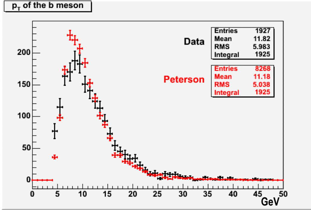
Figure 7.6: B^+ \rightarrow J/\psi K^+ data (black) and PYTHIA with msel=5 (red) and CKIN(3)=5 . With this value of CKIN(3) , events are missed when p_T(B) is \sim 5 GeV/c or below. All other msel=5 plots in this text have been produced with CKIN(3) set to 0. The histograms are normalized to the same number of B mesons.
