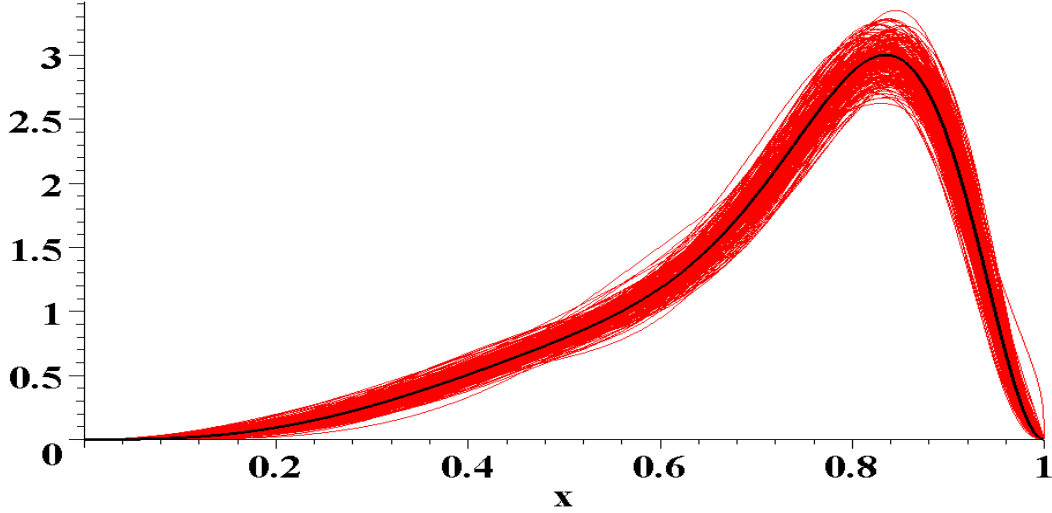
Figure 6.2: Curves that have been used for the error bar generation (red), together with the central curve that represents the central values of the parameters p_{1,..,5} (black).
