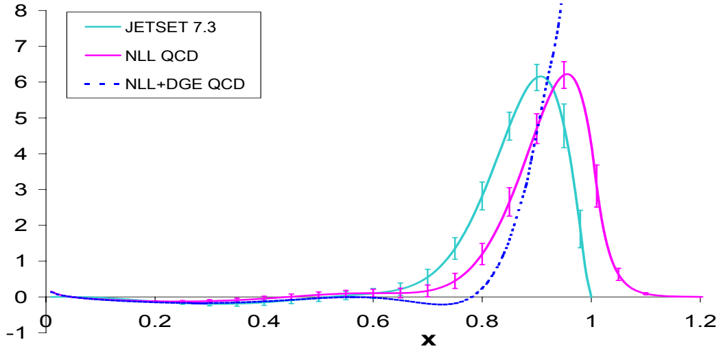
Figure 6.6: Comparison between the not-perturbative component obtained for the three perturbative QCD approaches treated in this chapter: JETSET, a NLL theoretical QCD computation [14] and a theoretical NLL+DGE computation [14]
