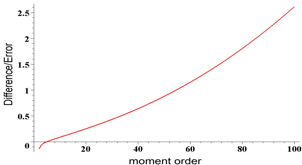
Figure 6.10: The difference between moments of a smooth fragmentation distribution and its binned version divided by the error as a function of the moment order.
