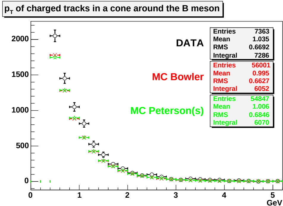
Figure 7.15: The p_T spectrum of tracks in a cone around the B meson. Comparison between the data and two Monte Carlo ( msel=5 ) samples with the Bowler and Peterson fragmentation functions. Histograms are normalized to the number of B mesons.
