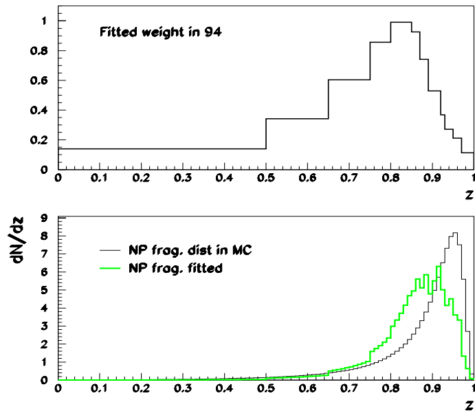
Figure 5.11: Fitted z distribution on 1994 selected events. Top: Distribution of the fitted weights. Bottom: Comparison between the initial Peterson distribution, used in the simulation generator, and the corresponding distribution favored by data events.
