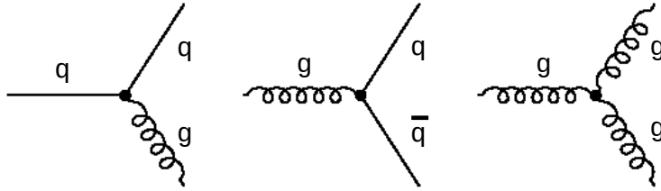
Figure 2.5: Elementary processes contributing to the parton shower model.
