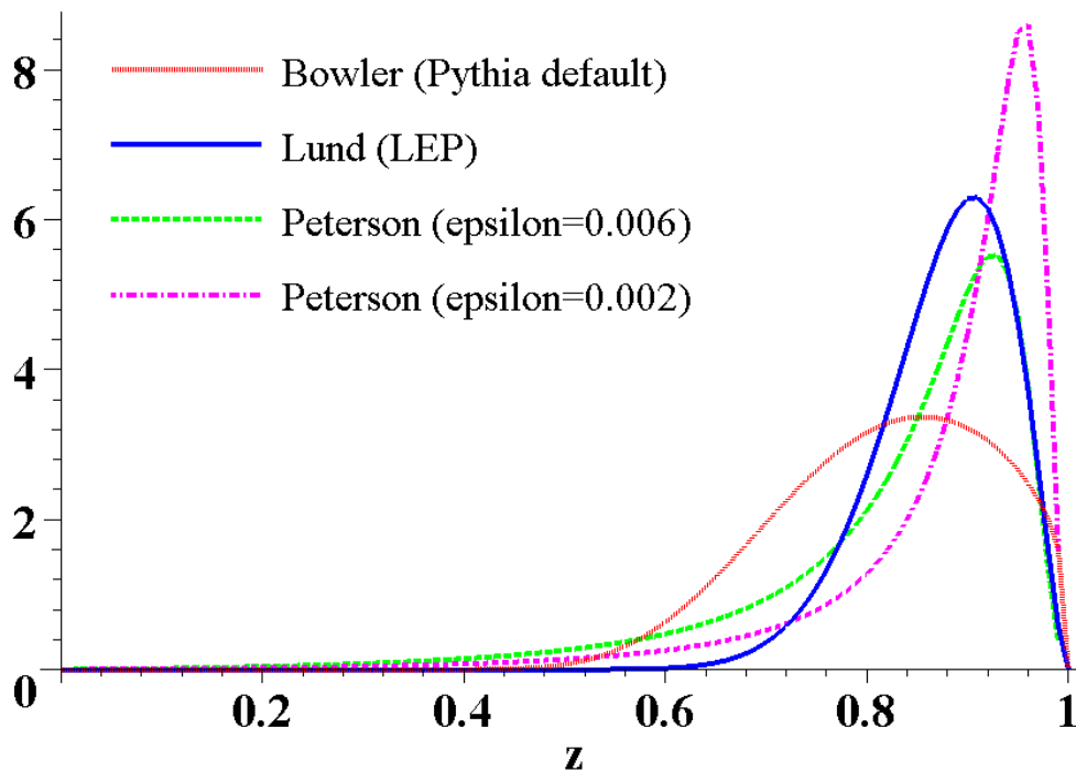
Figure 7.7: Three hadronization models: Peterson [35] with \epsilon = 0.006 (soft) and \epsilon = 0.002 (hard), Bowler [24] with (a = 0.3, b = 0.58, r_Q = 1) (the default in PYTHIA), and Lund [38] with (a = 1.68 ; b = 0.55) .
