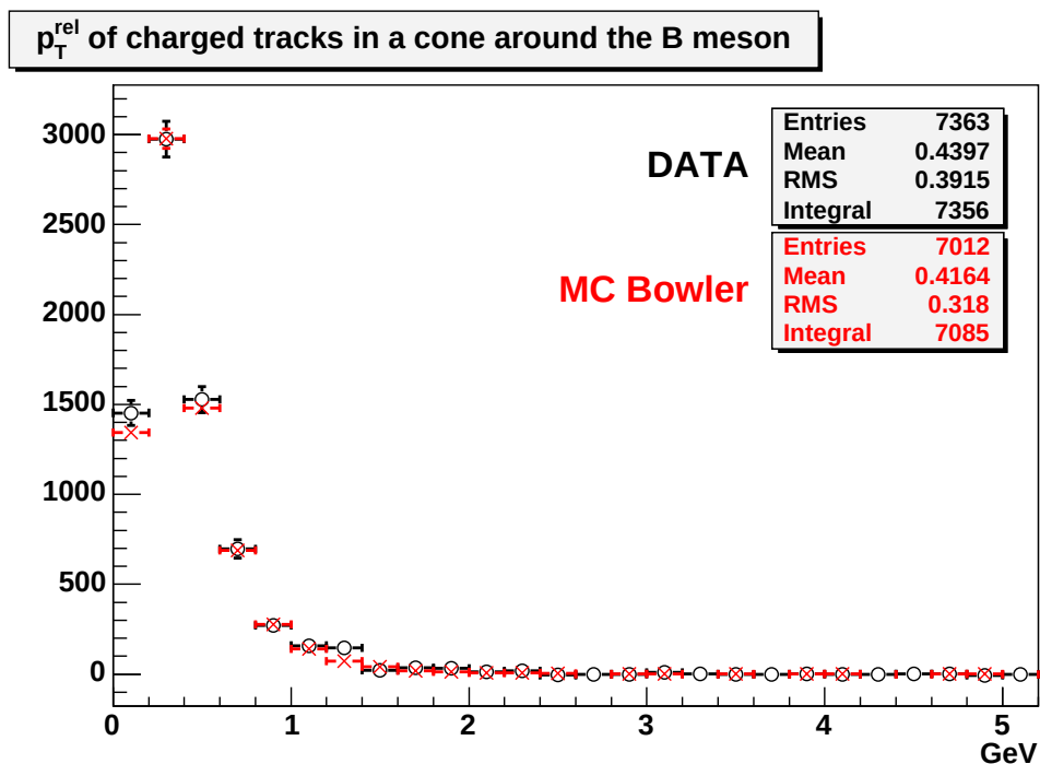
Figure 7.20: p_T^{rel} of tracks within a cone of \Delta R < 0.7 around the B meson in the msl=1 PYTHIA sample. Histograms are normalized to the number of B mesons.
