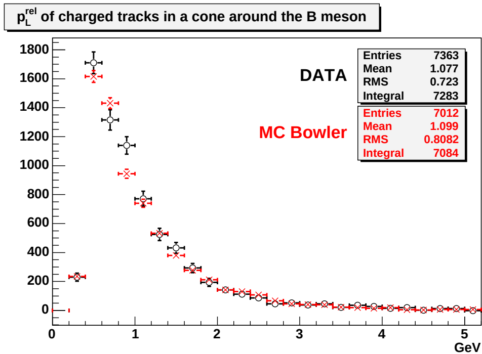
Figure 7.21: p_L^{\text{rel}} of tracks within a cone of \Delta R < 0.7 around the B meson in the m_{\text{sel}}=1 PYTHIA sample. Histograms are normalized to the number of B mesons.
