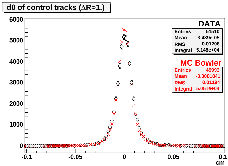
Figure 7.27: Plot of the impact parameter d_0 for control tracks in the m_{\text{sel}}=1 PYTHIA sample. Histograms are normalized to the number of B mesons.
