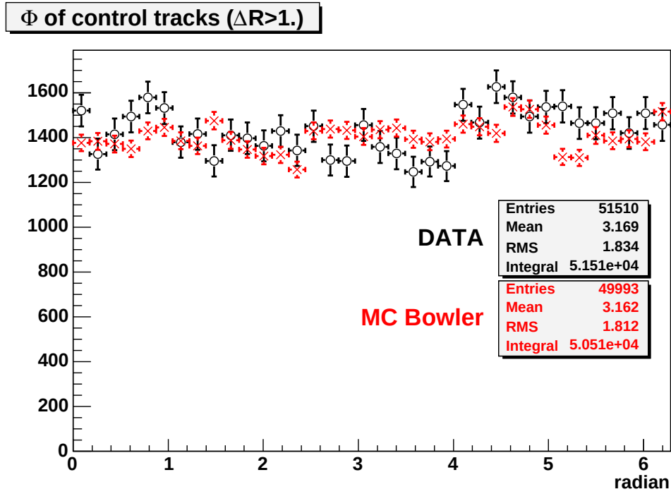
Figure 7.28: Plot of the angular variable \phi for control tracks in the msel=1 PYTHIA sample. Histograms are normalized to the number of B mesons.
