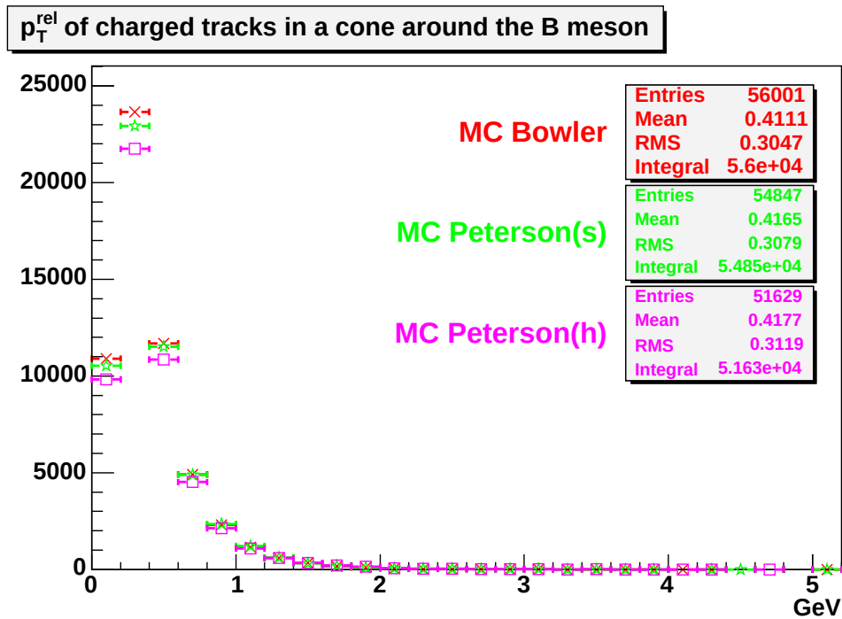
Figure 7.10: The component of tracks momentum transverse to the B meson, for tracks in a cone around it in three Monte Carlo samples, generated with different fragmentation functions.
