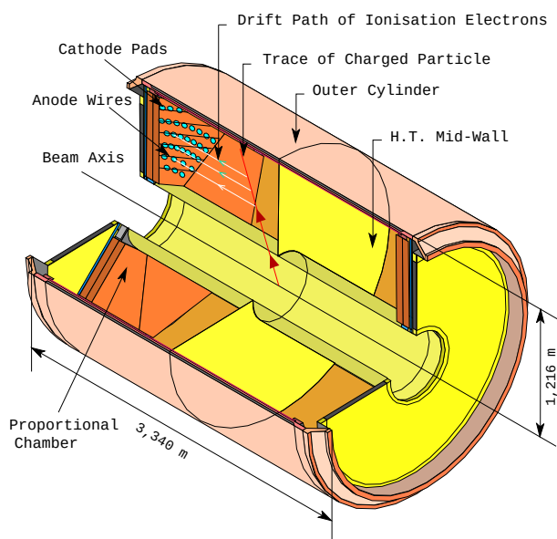
Figure 3.7: Scheme of the DELPHI Time Projection Chamber.
