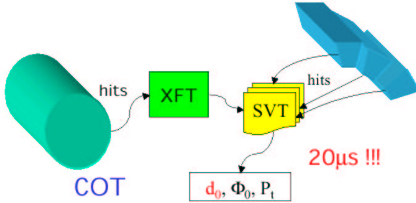
Figure 4.12: SVT principle of operation.
