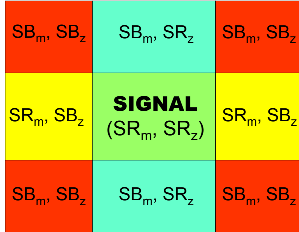
Figure 7.5: Regions of signal and sidebands for m(J/\psi K^+) and \Delta z
