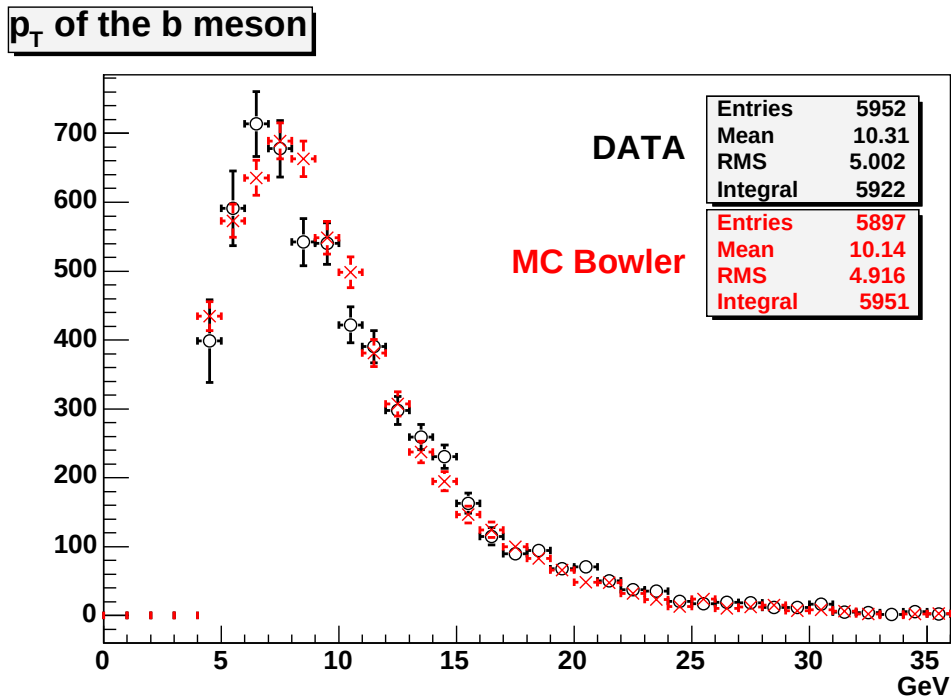
Figure 7.17: With the \text{msl}=1 PYTHIA setting, there is good agreement between data and Monte Carlo for the p_T of the B meson. Histograms are normalized to the number of B mesons.
