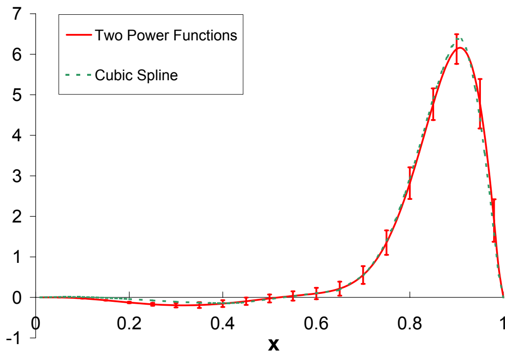
Figure 6.11: The extracted non-perturbative component of the fragmentation function from ALEPH, obtained using two different parametrizations: the power function of Equation (6.6) and a cubic spline. The perturbative QCD component has been taken from JETSET.
