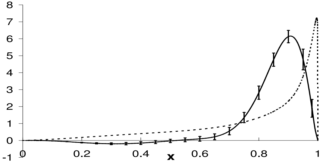
Figure 6.3: x -dependence of the perturbative (dotted line) and non-perturbative (full line) QCD components of the measured [31] b -fragmentation distribution. These curves are obtained by interpolating corresponding values determined at a large number of points in the x -variable. Quoted error bars correspond to measurement uncertainties and are correlated for different x -values. The perturbative QCD component is extracted from the JETSET 7.3 Monte Carlo generator. The dotted curve has to be complemented by a \delta -function containing 4% of the events, located at x = 1 .
