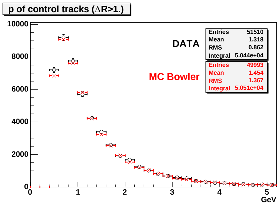
Figure 7.26: Plot of the 3-momentum for control tracks in the msl=1 PYTHIA sample. Histograms are normalized to the number of B mesons.
