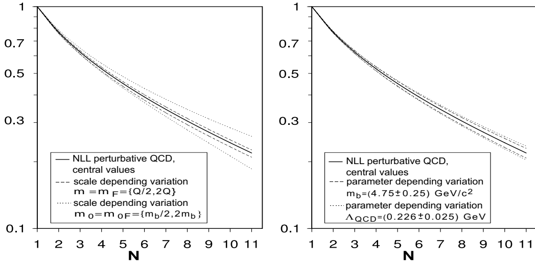
Figure 6.4: Variations of the calculated perturbative QCD component [14], depending on the renormalization scales ( \mu , \mu_0 ), the factorisation scales ( \mu_F , \mu_{0F} ), the b -quark mass ( m_b ) and \Lambda_{QCD}^{(5)} . The full lines are corresponding to the central values ( \mu = \mu_F = Q = 91.2 GeV, \mu_0 = \mu_{0F} = m_b , m_b = 4.75 GeV/ c^2 and \Lambda_{QCD}^{(5)} = 0.226 GeV).
