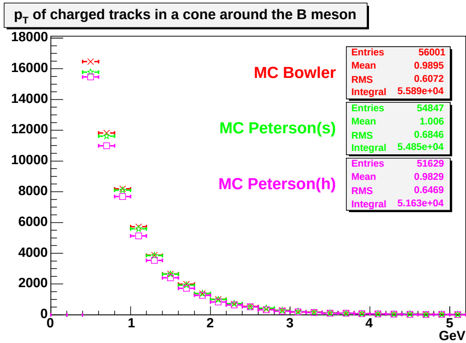
Figure 7.9: The p_T spectrum of tracks in a cone around the B meson in three Monte Carlo samples, generated with different fragmentation functions.
