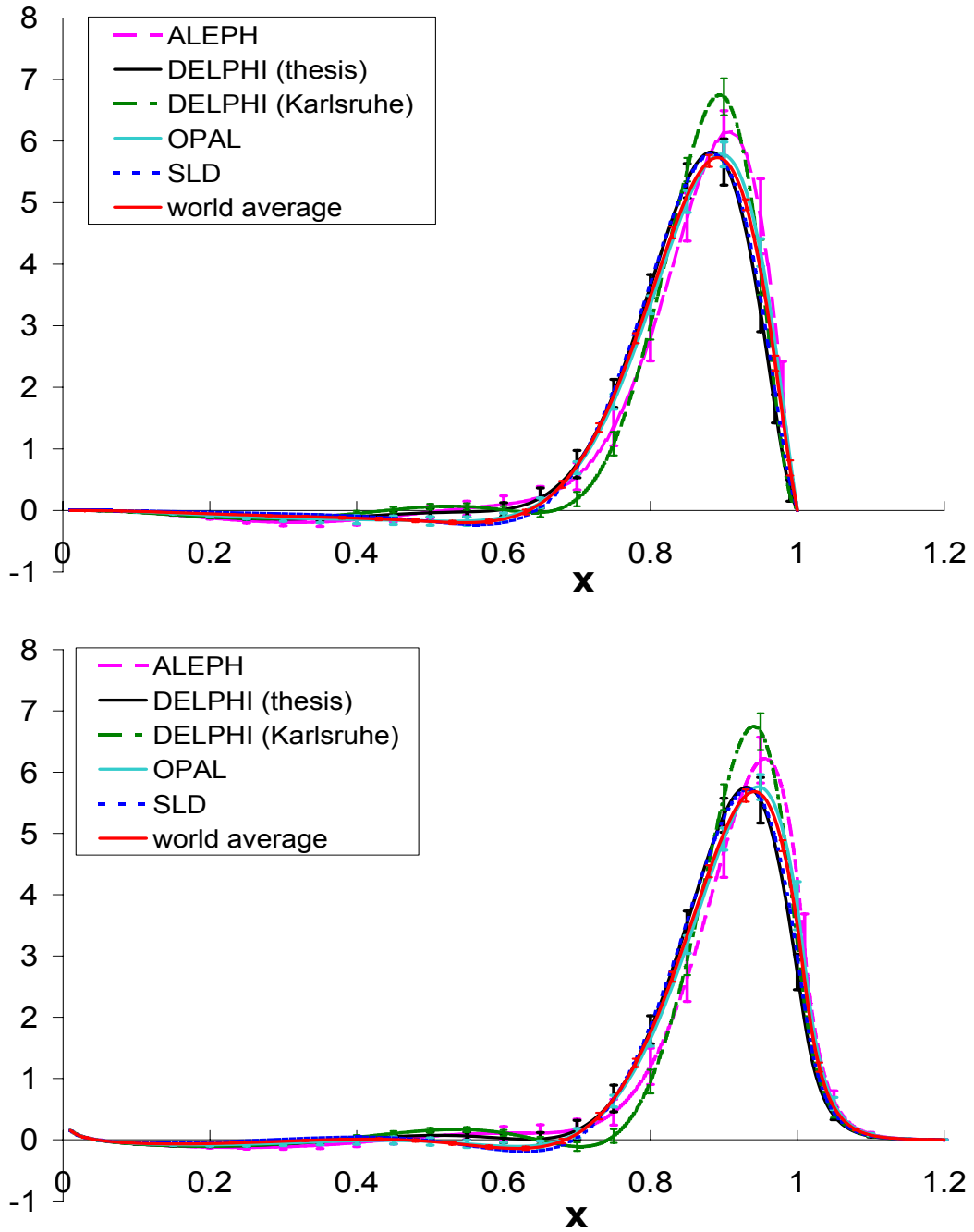
Figure 6.14: Comparison of the extracted non-perturbative QCD component of the b quark fragmentation function for ALEPH [31], DELPHI (the result presented in this thesis), DELPHI- Karlsruhe [34], OPAL [32], SLD [33] and the combined fragmentation distribution. Top: the perturbative QCD component has been taken from JETSET 7.3. Bottom: the perturbative QCD component has been taken from NLL QCD [14].
