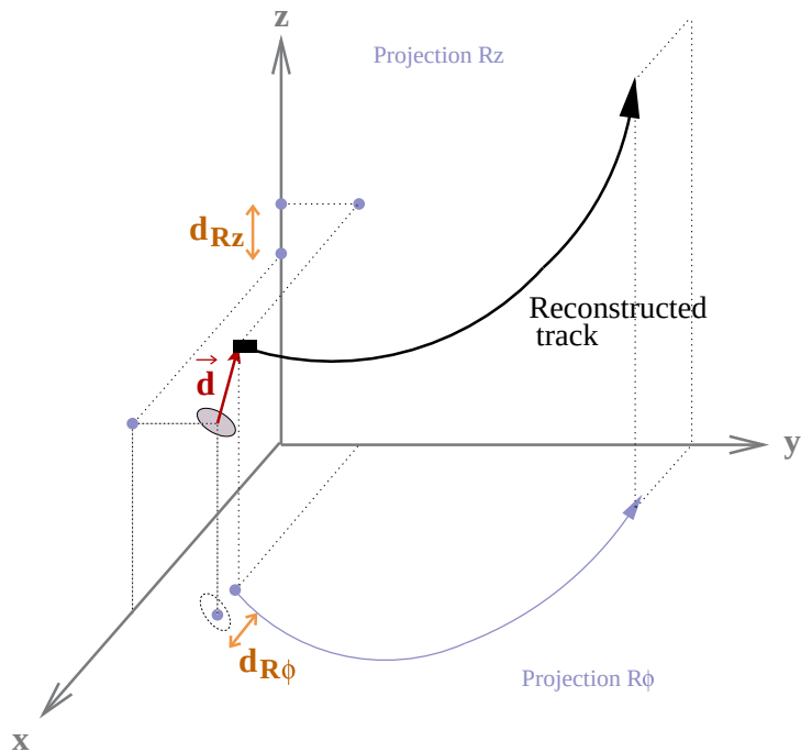
Figure 3.9: Impact parameter definition for the R\phi and Rz planes. d is the minimal distance, in space between the primary and secondary vertices.
