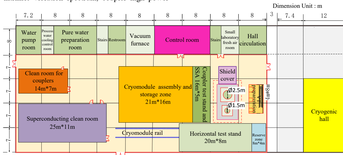
Figure 4: Layout of superconducting radio-frequency hall.
