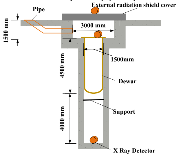
Figure 3: Diagram of vertical test pit.
