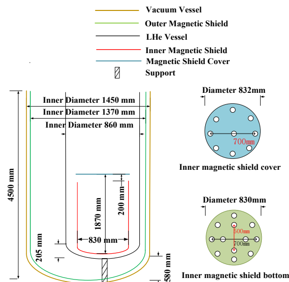
Figure 2: Vertical test dewar diagram.
