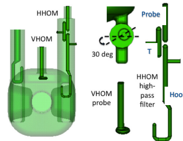
Figure 2: HHOM and VHOM couplers of the rf-dipole crabbing cavity.
