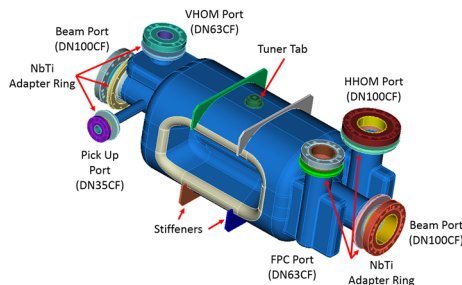
Figure 1: 400 MHz LARP prototype rf-dipole cavity.
