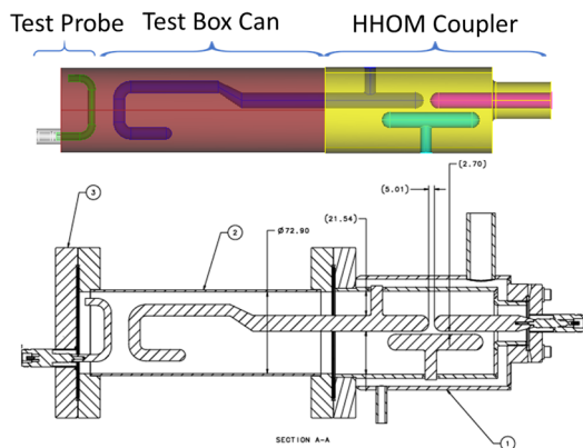
Figure 3: Schematic (top) and mechanical drawing (bottom) of the rf test box with HHOM coupler.
