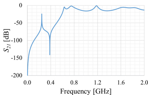
Figure 4: S_{21} transmission of the HHOM coupler in the rf test box.
