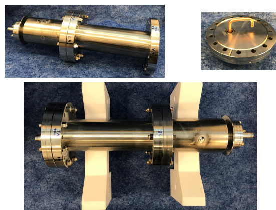
Figure 6: Test box can assembly with HHOM coupler (top left), test probe (top right), and fully assembled setup (bottom).
