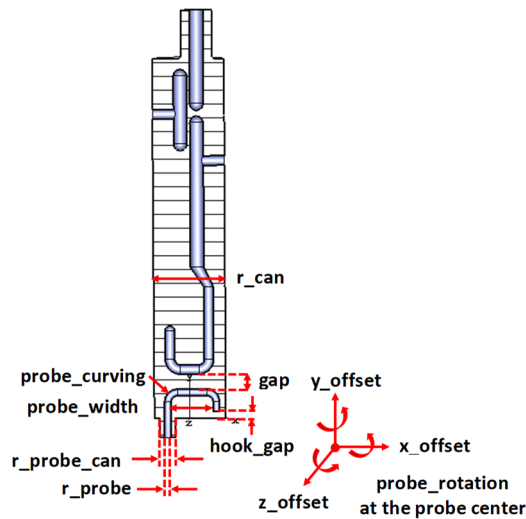
Figure 5: RF test box parameters evaluated for tolerances.
