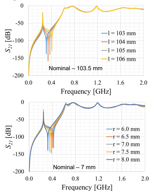
Figure 10: Dependence on S_{21} transmission with varying probe length (top) and diameter (bottom).
