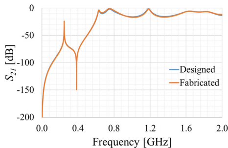
Figure 8: S_{21} transmission for the designed and fabricated rf test box.
