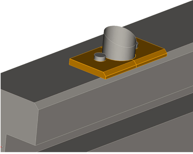
FIG. 8. The numerical simulation model for a pair of ferrite dampers.
