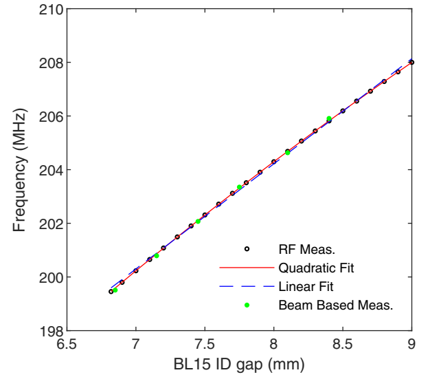
FIG. 3. Tracking the resonant frequency of the HOM #3 at different BL15 ID gap.
