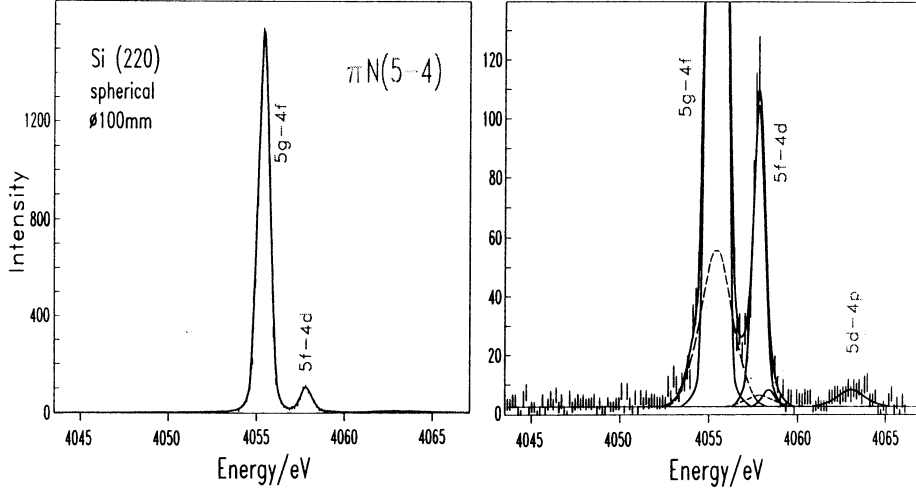
Fig. 3. The spectrum of the 5 \rightarrow 4 transition in pionic N. The left-hand side shows the total view of the collected data. The right-hand side is the same spectrum at expanded vertical scale, revealing details about the weaker components.
