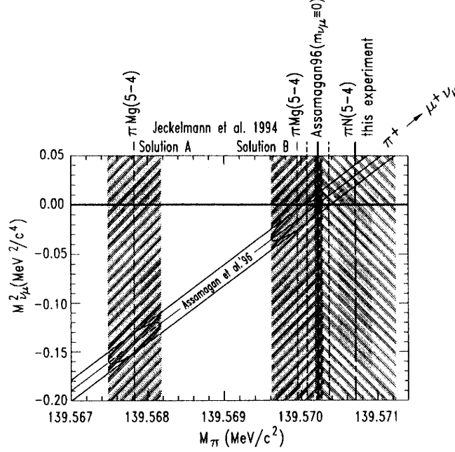
Fig. 4. The squared neutrino mass as a function of the pion mass. The slanted band denotes the muon momentum p_\mu . The vertical bands indicate recent pion mass measurements. The overlap regions of the p_\mu band with the individual pion mass bands denote the corresponding M_{\nu_\mu}^2 values.
