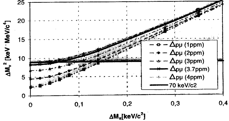
Fig.1. The uncertainty of the squared muon neutrino mass. For details see the text.
