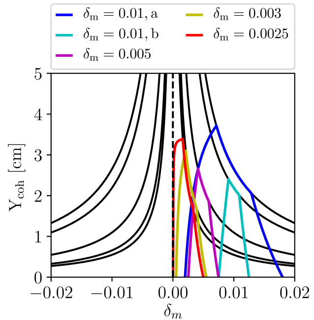
Figure 3: Comparison of coherent amplitudes with different \delta_m values. \delta_m = 0.01, a corresponds to results with the natural chromaticity and \delta_m = 0.01, b is \xi = -0.5 ; all results besides \delta_m = 0.01 correspond to \xi = -0.5 .
