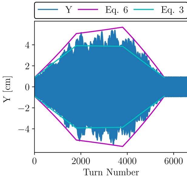
Figure 1: The vertical position of the bunched beam and its comparison with Eq. (3) and Eq. (6) for helions crossing the |G\gamma| = 12 - \nu_y with \xi = -2.64 .
