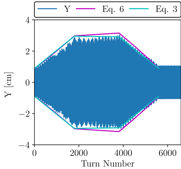
Figure 2: The vertical position of the bunched beam and its comparison with Eq. (3) and Eq. (6) for helions crossing the |G\gamma| = 12 - \nu_y with \xi = -0.5 .
