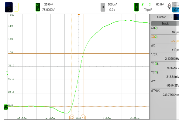
Figure 2: Driver output voltage measurement with 160 V driver supply and 50 Ohm load (attenuator with 18 GHz BW) on Keysight scope DSO-X 6002 (1 GHz BW).
