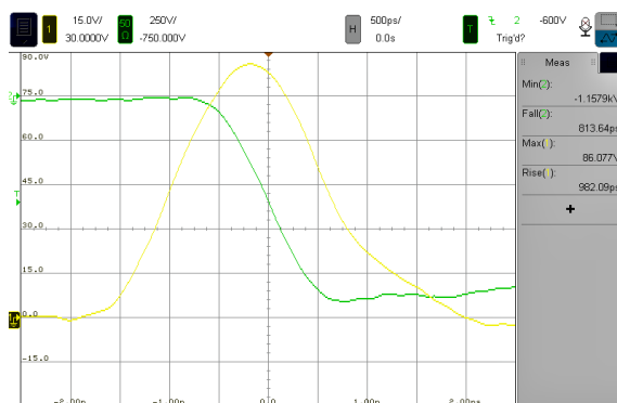
Figure 4: Gate-source (yellow) and load voltage (green) with 280 V driver and U_{ds} = 1.3 kV; measurements are influenced by scope and probe BW limitation (1 GHz and 700 MHz respectively).
