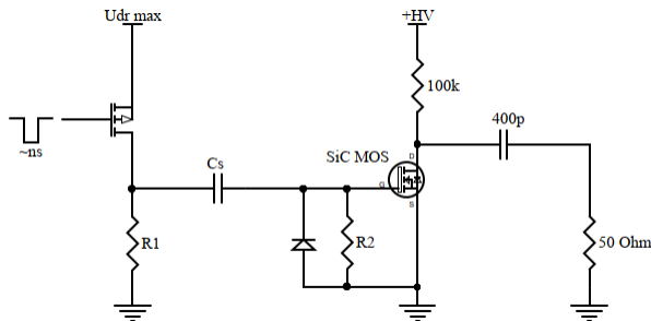
Figure 1: Schematic of super boosting setup.
