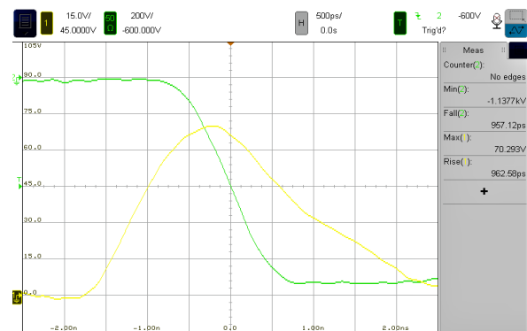
Figure 3: Gate-source voltage (yellow, 15V/div) and load voltage (50 Ohm, green, 200V/div) with 160 V driver; measurement on SiC MOS IMBF170R450M1 operating at U_{ds} = 1.3 kV.
