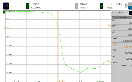
Figure 5: Output of the two stage Marx generator with Si diode sharpener; due to scope BW the real slew rate is higher than 4 kV/ns measured.
