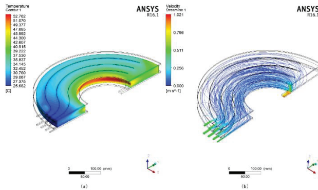
Figure 5: Distribution of temperature and water velocity on MA core indirect-cooling structure.
