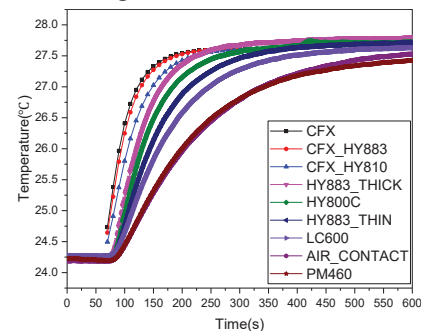
Figure 4: Temperature rising curve of different TIM in the flow outlet.
