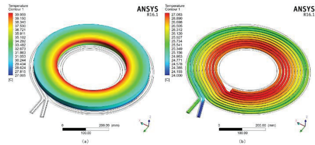
Figure 3: Distribution of temperature on MA core and water in indirect-cooling structure.
