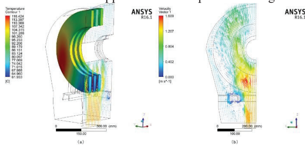
Figure 2: Distribution of temperature and air velocity on MA core in air-forced cooling structure.
