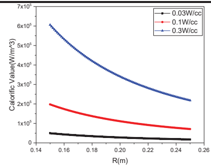
Figure 1: Power density distribution along the radius in MA core.
