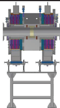
Figure 6: A cross-section of high power test cavity.
