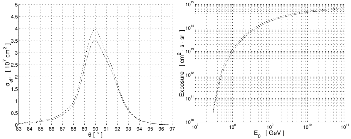
Figure 3: Left : effective surface at the trigger level as a function of the incoming \nu_\tau angle with the local vertical for 10^{19} eV \nu_\tau . Right : expected exposure in one year of data taking as function of the incident neutrino energy. The different curves correspond to triggers requiring 3 or 4 coincident antennas.
