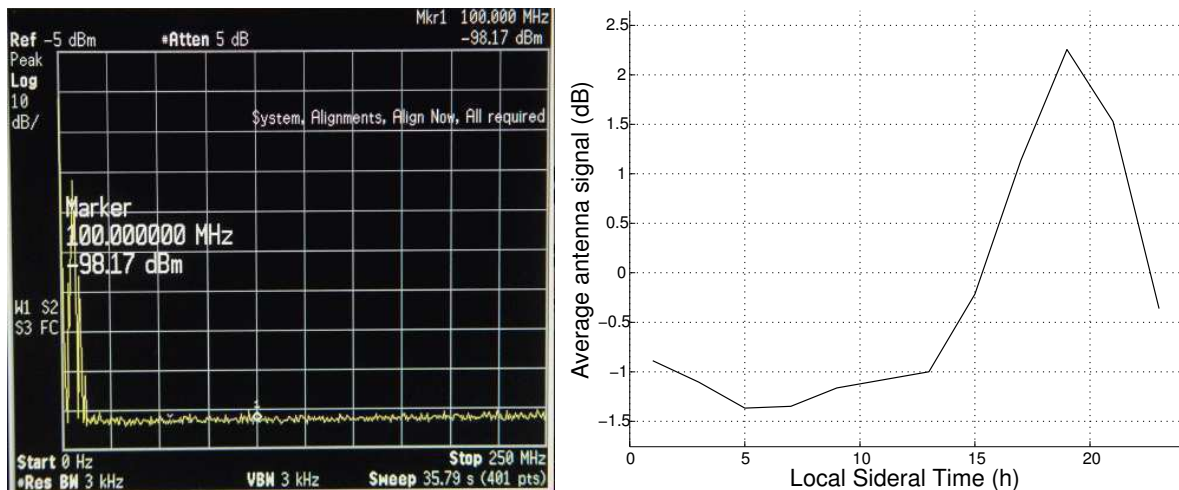
Figure 1: Left : average Fourier transform of the background noise for a 21CMA antenna. Right : antenna signal averaged over 15 hours of data taking as a function of the local sideral time, peaking to the galactic radio emission.
