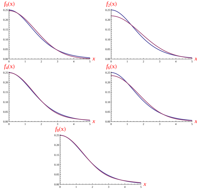
Fig. 2. Free-GCS example. The \sigma parameter of f_0 is adjusted for each order for a best fit. Approximations do not improve uniformly with increasing order of the partial sum.
