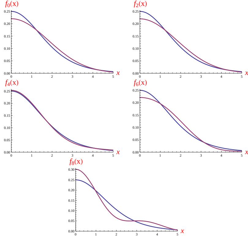
Fig. 1. Fixed GCS example. Partial sums of order beyond k = 4 do not improve as approximations of the non-Gaussian f(x) , the curve peaking at 0.25.
