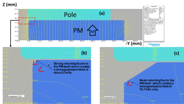
Figure 2: Magnetic flux lines of a quarter-period-long model of a 28-mm-period undulator (the bottom half is shown). The moment is set along the Z (beam axis).
