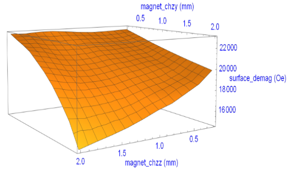
Figure 3: The maximum PM surface demagnetization field of the APS-U 28-mm period undulator design as a function of the PM-zz and -zy chamfers size at a gap of 8.5 mm.
