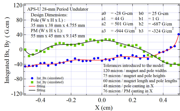
Figure 5: Simulation results of the integrated Bx and By field errors over the length of the APS-U 28-mm model at each different position in X. The "a" and "b" components inserted in the plot represent the integrated field errors of B_x and B_y , respectively.
