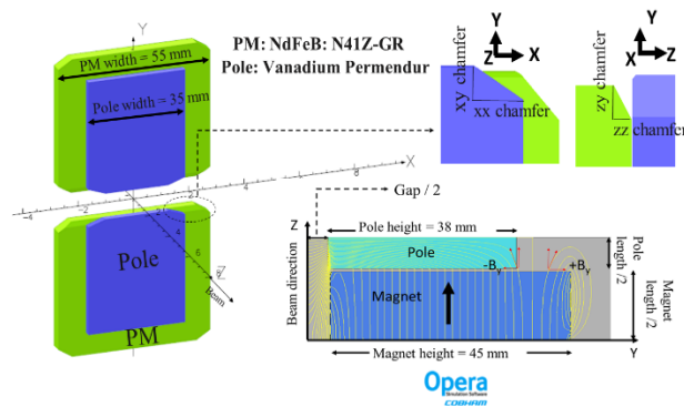
Figure 1: A quarter-period-long narrowed pole 28-mm period undulator designed for the APS-U. The definitions of the chamfers on the pole and magnet edges are shown on top right images. The yellow lines are the magnetic flux lines in 2D (bottom right image). The red arrows show the magnetic flux contributions to the B field components.
