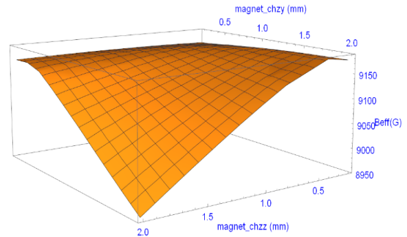
Figure 4: The B_{eff} of the APS-U 28-mm period undulator design as the PM-zz and -zy chamfers change at a gap of 8.5 mm.
