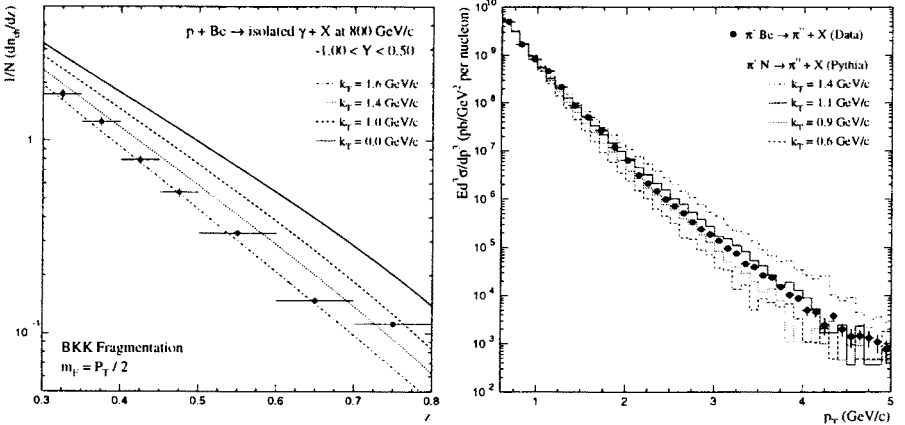
Fig. 3. Left: The distribution of charged particles in jets opposite isolated photons with p_T > 5.5 GeV/c in the 800 GeV/c data ( z is momentum of particles, rescaled to the photon momentum). Curves are expectations using BKK fragmentation and various k_T values. Right: Comparison of Pythia Monte Carlo for several k_T values with \pi^0 data.
